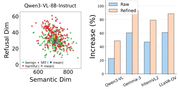
Figure 7: Illustration of internal validation.
