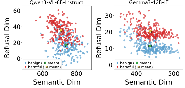
Figure 3: RV-plane visualization of paired samples on Qwen3-VL-8B-Instruct and Gemma-3-12B-IT at layer 22 and layer 30, respectively.
