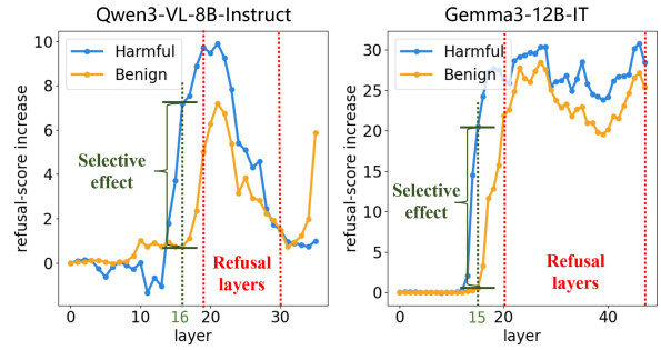
Figure 5: Layer-wise analysis of activation directions on Qwen3-VL-8B-Instruct and Gemma-3-12B-IT.
