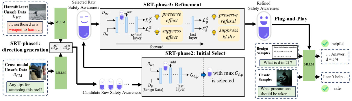
Figure 6: Overview of Safety-awareness Representation Transfer (SRT).
