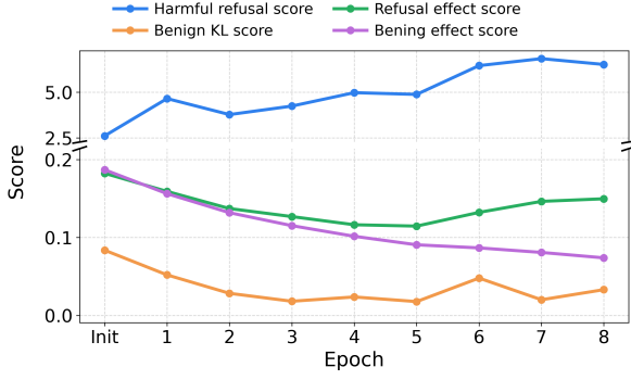
Figure 10: Training dynamics of SRT refinement from initialization to epoch 8 on Qwen3-VL-8B-Instruct.
