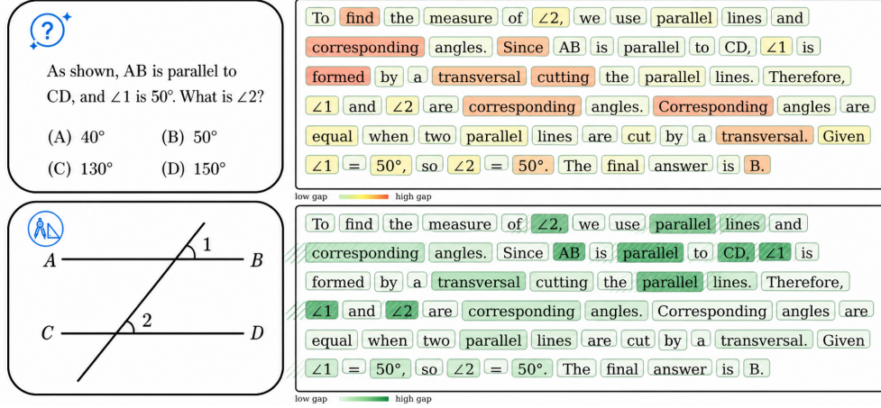
Figure 1: Token-level grounding visualization. Standard student–teacher gaps highlight both visual and generic tokens, whereas factual–counterfactual teacher gaps more selectively emphasize image-dependent tokens.
