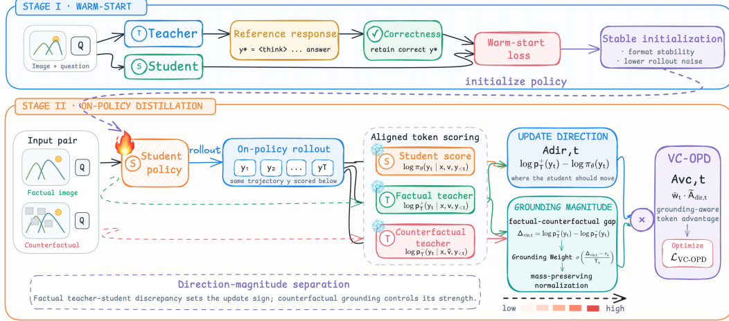
Figure 3: Overview of VC-OPD. The framework first warm-starts the student with filtered teacher-generated reasoning responses. During visual counterfactual on-policy distillation, student rollouts are scored by the teacher under factual and counterfactual visual inputs. The factual teacher provides the update direction, while the factual-counterfactual gap produces grounding-aware token weights that modulate the final token-level advantage.
