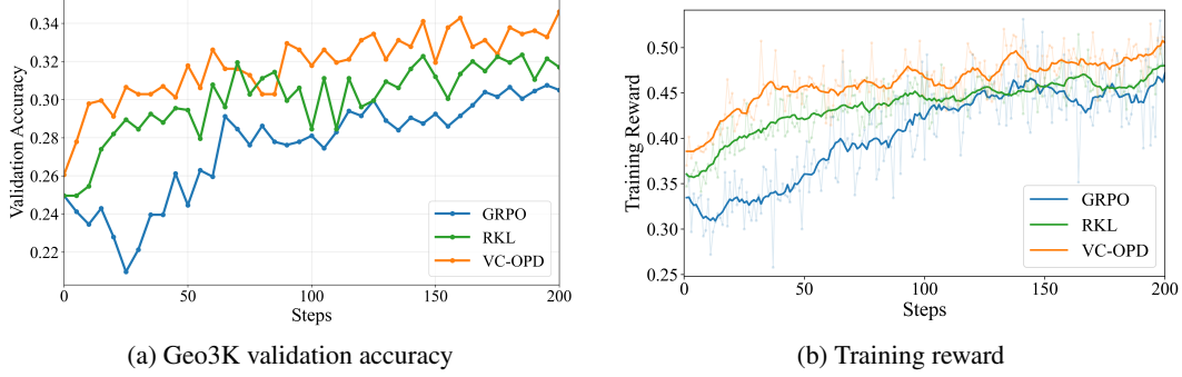
Figure 4: Training dynamics over 200 optimization steps. VC-OPD improves faster than GRPO, is more stable than RKL, and achieves the highest validation accuracy and training reward.
