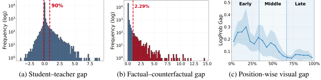
Figure 2: Token-level signal statistics. Standard OPD gaps are often small, while factual-counterfactual gaps reveal sparse and position-dependent visual grounding signals.
