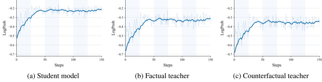
Figure 5: Log-probability diagnostics during VC-OPD training. We plot the average response-token log probability of the student, factual teacher, and counterfactual teacher over training steps. The curves stabilize after the early optimization phase, indicating that both teacher-scoring branches remain in a comparable and numerically stable prediction regime.
