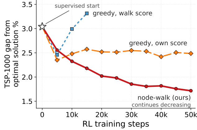
Figure D.3: Three GRPO runs from the same supervised model. The runs differ only in how routes are sampled and scored during RL training. Blue: sampling with the greedy decoder and scoring with the node-walk likelihood, the TSP-1000 gap rises above the supervised starting point. Orange: sampling with the greedy decoder and scoring with its own exact likelihood, the gap stays flat. Red: sampling and scoring with node-walk decoding (our approach), the gap falls steadily.
