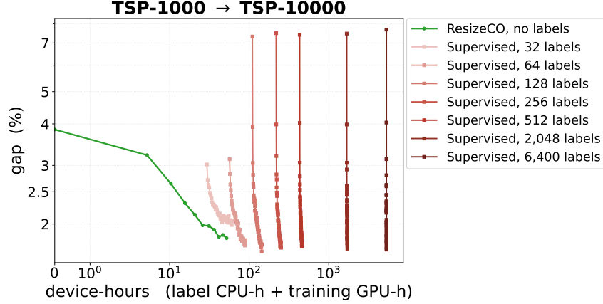
Figure D.1: Gap on TSP-10000 against total device hours, the CPU hours of computing the LKH-3 labels plus the GPU hours of training. Every run starts from the same supervised model trained at size 1000. The green line is the label-free GRPO training of ResizeCO, and each red line is supervised training with a fixed number of labels.
