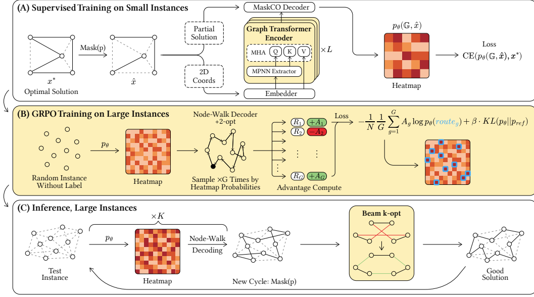
Figure 1: The three stages of ResizeCO. Yellow marks our novel contributions. (A) Supervised training. A masked-diffusion model is trained using small labeled instances with a Graph Transformer encoder. (B) RL training. Label-free GRPO training on larger instances. A node-walk decoder samples G routes from the heatmap. Each route is denoted route_g , and their lengths alone determine the advantage. (C) Inference on large instances. Multiple correction cycles are executed. Each cycle runs K unmasking steps to build an edge heatmap and decodes the heatmap into a route with the node-walk decoder. The route is then “polished” with our GPU beam k -opt search. Before the next cycle, the route is partly re-masked.
