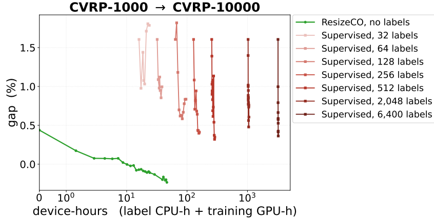
Figure D.2: Gap on CVRP-10000 against total device hours, the CPU hours of computing the HGS labels plus the GPU hours of training. Every run starts from the same supervised model trained at size 1000. The green line is the label-free GRPO training of ResizeCO, and each red line is supervised training with a fixed number of labels.
