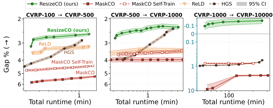
Figure 3: CVRP solution quality (gap) against total run time for three source-to-target pairs. Each line varies the compute budget of one method. Our approach ResizeCO in green achieves superior quality in short durations. From CVRP-1000 to CVRP-10000, ResizeCO’s routes are shorter than the HGS reference solutions (negative gap).
