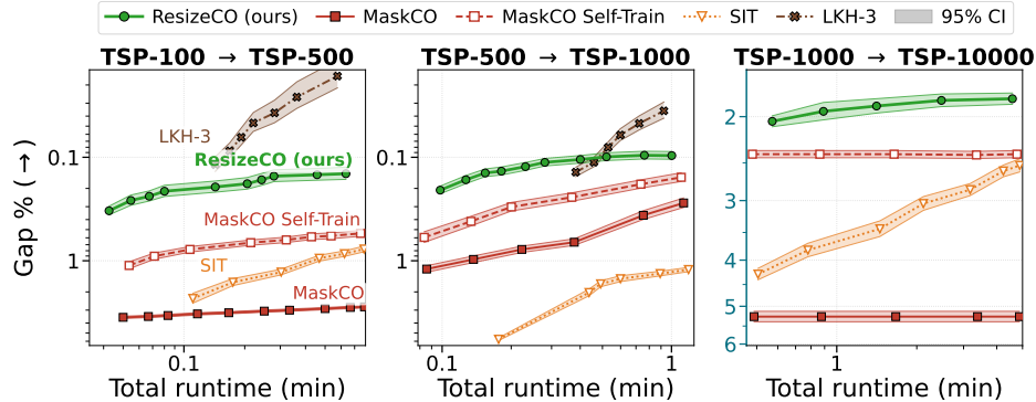
Figure 4: TSP solution quality (gap) against total run time for three source-to-target pairs. Each line varies the compute budget of one method. Our approach ResizeCO in green achieves superior quality in short durations. We limit runs on TSP-10000 to less than 5 minutes, which LKH-3 exceeds. Error bars correspond to 95% confidence intervals.
