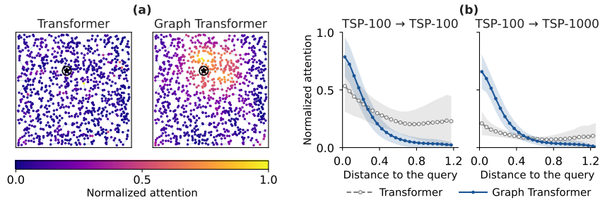
Figure 2: Encoder attention, averaged over all layers and normalized per row. (a) One query node (star) at TSP-1000. (b) Mean attention by distance to the query node. Shaded bands denote std over query nodes.
