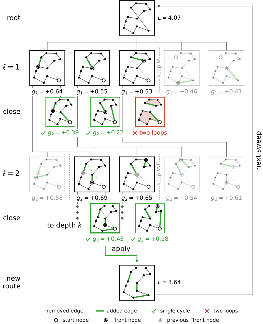
Figure B.1: An example sweep of the GPU beam k -opt search on a 12-node instance. Every panel draws the same nodes and differs only in its edges. Each level extends every branch of the beam and keeps the branches with the largest gains, and the beam narrows with depth. Each level also closes every branch back to the start node, and a closing that splits the route into two loops is discarded. The sweep applies the kept closures that do not overlap on the route, here only the one with the largest gain. Sweeps repeat until no route improves.
