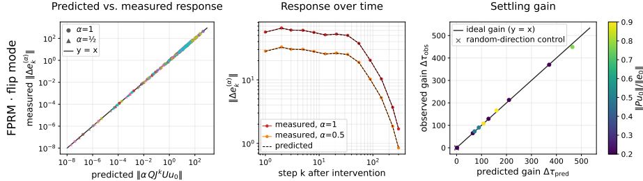
Figure 2: Local oscillatory-coupling theory predicts the response and settling cost in the original FPRM recurrence. We control only the Jacobian-identified oscillatory coordinate once with \alpha \in \{0, 0.5, 1\} and then resume unmodified recurrent updates. HRM results in Appendix A.4.1.
