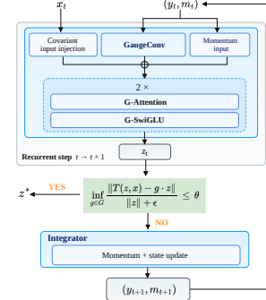
Figure 4: Overview of the QRR recurrent block.
