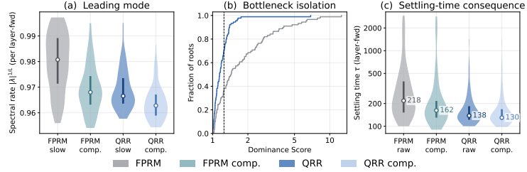
Figure 5: Spectral analysis and settling near solution roots for FPRM and QRR. Results for HRM in Appendix A.4.2
