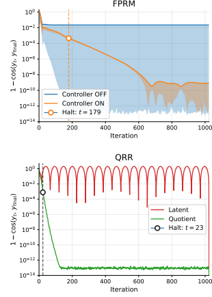
Figure 3: Convergence and halting in quotient space.
