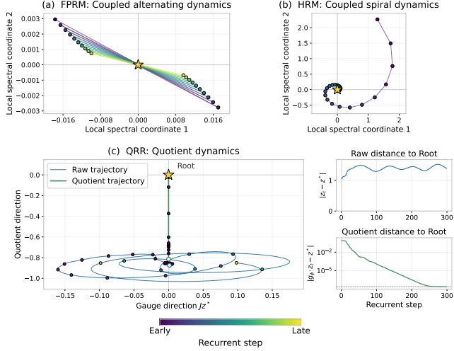
Figure 1: Oscillatory geometry and quotient convergence. FPRM and HRM exhibit distinct alternating and spiral dynamics near solution roots. In QRR, raw motion persists while quotient trajectory contracts.
