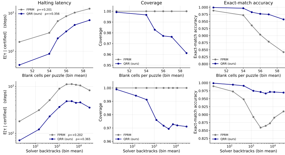
Figure 9: Adaptive halting as a function of Sudoku difficulty. Difficulty as the number of blank cells (top) and the backtrack count (bottom). Left: mean halting time among certified examples. Middle: fraction of examples certified within the rollout budget. Right: exact-match accuracy.
