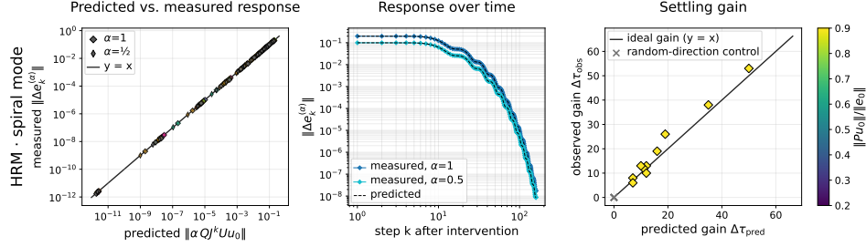
Figure 6: The local oscillatory-coupling prediction extends to the two-dimensional spiral dynamics of HRM. We modify only the Jacobian-identified oscillatory coordinate once with \alpha \in \{0, 0.5, 1\} and subsequently resume the original nonlinear HRM recurrence.
