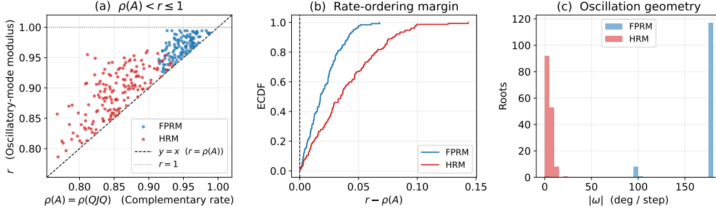
Figure 8: Spectral separation of leading oscillatory modes. (a) Leading-mode modulus r and complementary spectral radius \rho(A) . (b) Spectral margin r - \rho(A) . (c) Oscillation angle |\omega| for FPRM and HRM.
