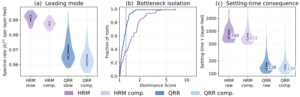
Figure 7: Spectral organization and settling in HRM and QRR. (a) Leading and complementary spectral rates near certified solution equilibria. QRR rates are measured in quotient space. (b) Distribution of the dominance score D = \log r_{\text{comp}} / \log r_{\text{lead}} . (c) Root-relative settling time before and after factoring out the leading-mode response.
