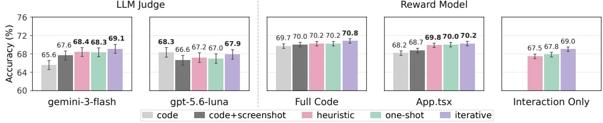
Figure 3: We train a reward model with varying levels of interaction and observe that including interaction data improves accuracy in terms of alignment with human preferences. GPT 5.6 Luna is the only exception where adding interaction offers comparable performance to code only. We fine-tune from Qwen-3.5-9B as our base model and train each approach 5 times. Bolded values are statistically significant against code+snapshot, calculated by a sample-wise paired t-test.
