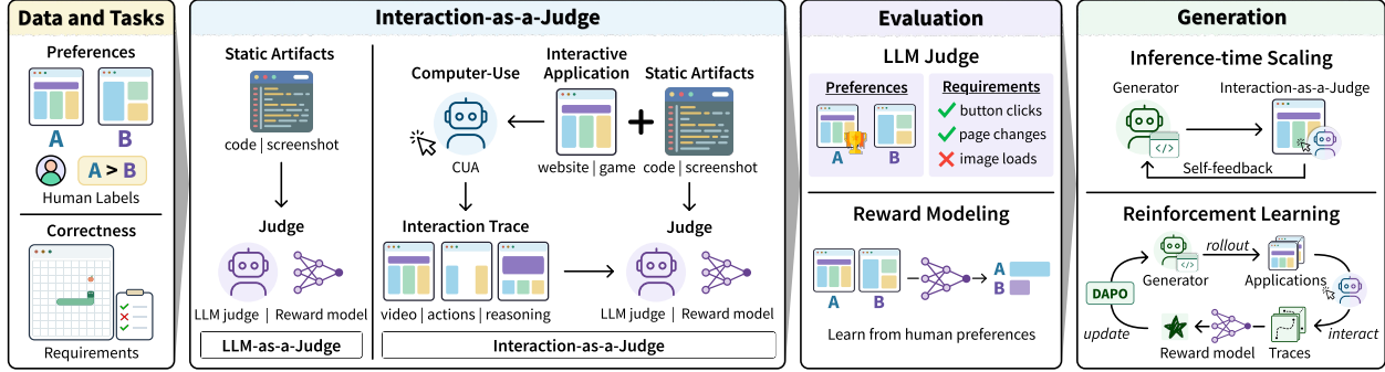
Figure 1: We present Interaction-as-a-Judge, an evaluation paradigm that uses interaction traces to improve evaluation and generation. We compare against non-interactive judges and evaluate on pairwise preferences and reward modeling. We also show how to apply Interaction-as-a-Judge for inference-time scaling and as a reward signal for standard post-training via reinforcement learning.
