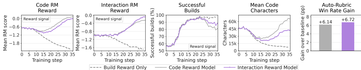
Figure 6: We train a Qwen-3.5-9B model using code-only and interaction-only reward models. As expected, each performs better on its respective training objective, but the interaction-only model leads to improvements in neutral criteria such as build success rate and decreased code length. We use an auto-rubrics based judge and find a significant improvement over the base model. The build reward baseline naturally degrades in reward for both reward models.
