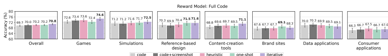
Figure 9: Per-category reward-model agreement (%) with full code input, averaged over five seeds. Error bars show 95% Wilson intervals over pooled seed-battle outcomes.
