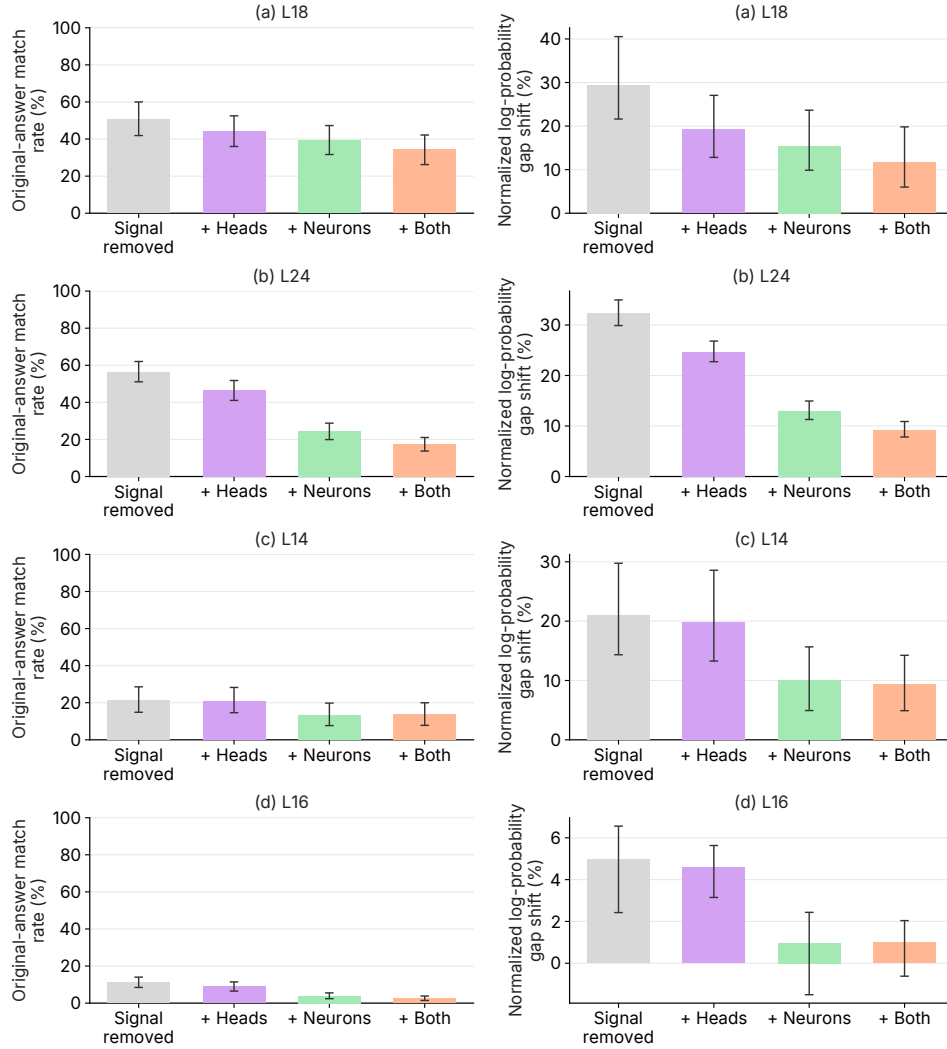
Figure 15: Signal removal followed by restoration of natural negated component values ( \beta = 1 ). Rows show (a) Gemma 3-4B-IT, (b) Gemma 3-12B-IT, (c) Llama 3.1-8B-Instruct, and (d) Qwen3.5-9B.
