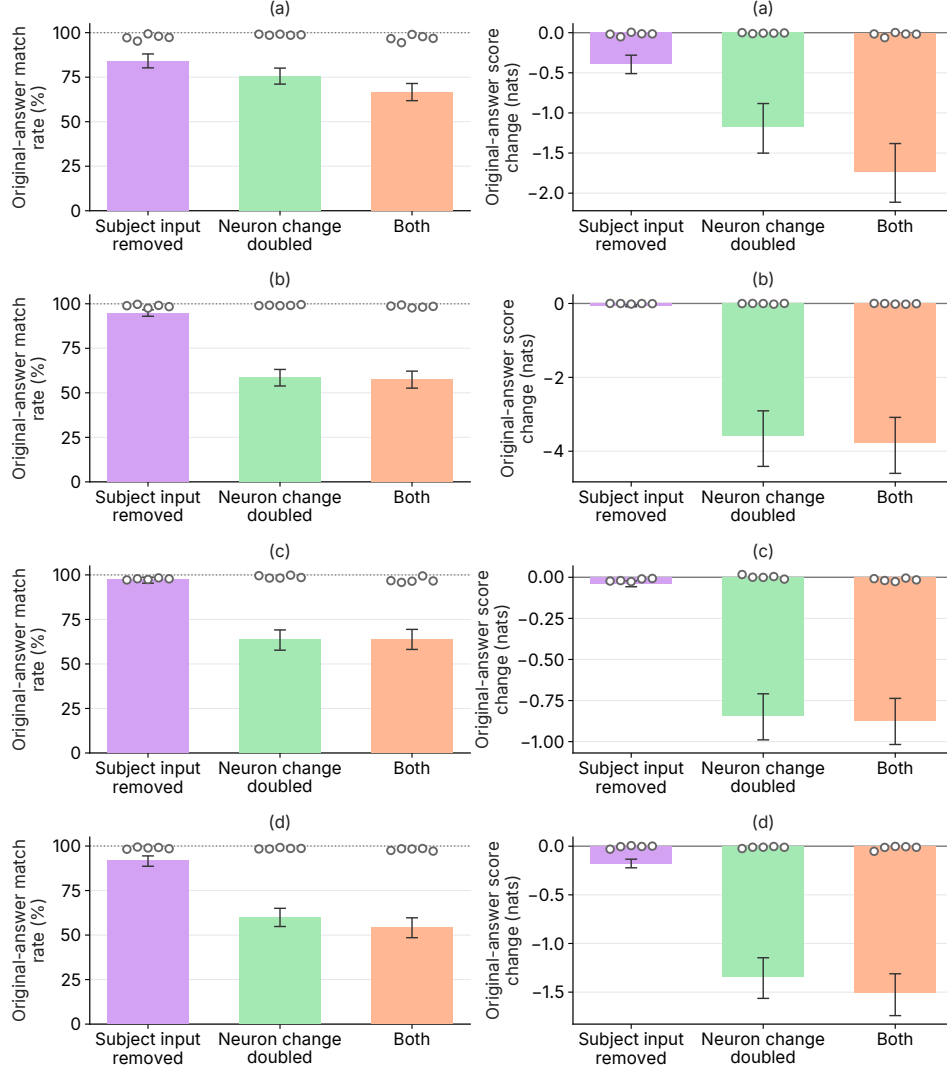
Figure 16: Interventions on repeated-answer failures in (a) Gemma 3-4B-IT, (b) Gemma 3-12B-IT, (c) Llama 3.1-8B-Instruct, and (d) Qwen3.5-9B. Left: original-answer match rate. Right: change in the original answer’s full-sequence log-probability relative to its unmodified negated baseline. Interventions continue during generation; error bars show 95% question-bootstrap intervals.
