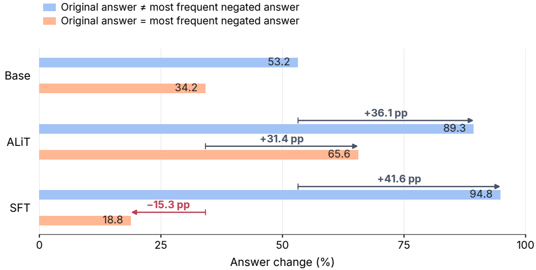
Figure 17: Answer change for Base, ALiT, and SFT, grouped by whether the original answer matches the most frequent negated answer. Arrows show percentage-point changes from Base within each group.
