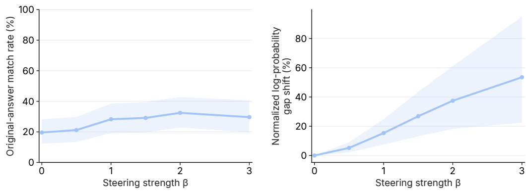
Figure 14: Prompt-only negation-direction removal at L15 in Llama 3.1-8B-Instruct.
