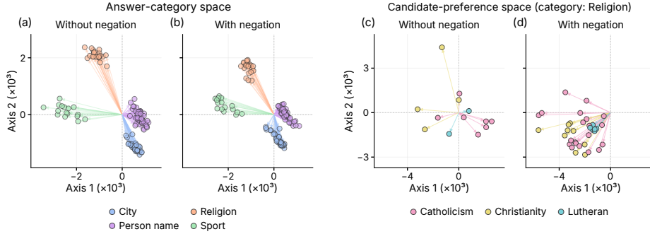
Figure 5: Negation largely preserves the shared answer category structure (a–b), while redirecting candidate-space representations toward a specific direction (c–d). Arrows show independently computed activations without centering or normalization.
