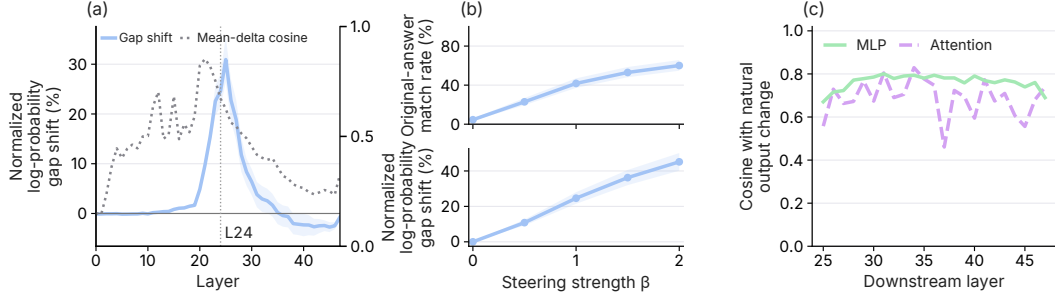
Figure 3: Removing the negation direction in Gemma 3-12B-IT. (a) Layerwise effects of steering with the negation signal ( \beta = 1 ), overlaid with negation-delta similarity. (b) Causal effects of steering with the negation signal at (L24). (c) Cosine similarity between attention and MLP output changes induced by natural negation and by steering ( \beta = 3 ). Effects are averaged over six benchmarks. Shading indicates 95% bootstrap intervals.
