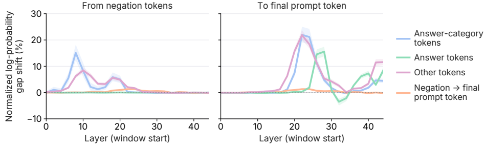
Figure 9: Information flow in Gemma 3-12B-IT. Left: from negation tokens to other token groups and Right: from each group to the final prompt token.
