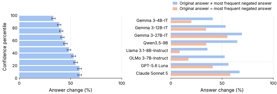
Figure 2: Left: Answer change rates decrease with confidence in the original answer (mean token log-probability; results averaged across six open-source models). Right: Answer change rates are also lower when the original answer is the model’s most common response under negation.
