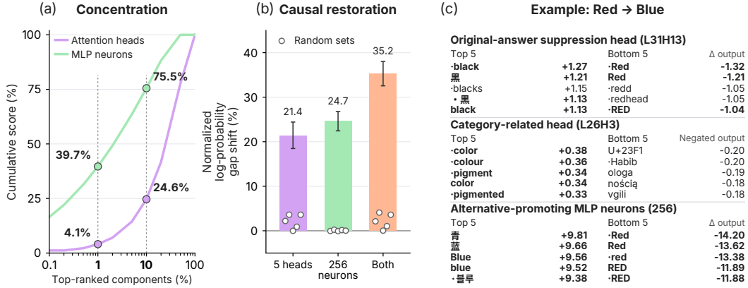
Figure 4: Components involved in forming alternatives in Gemma 3-12B-IT. (a) Cumulative head and neuron scores. (b) Effects of restoring their non-negated values, averaged across six benchmarks; dots show matched random controls. (c) Unfiltered logit lens top/bottom five for an illustrative example.
