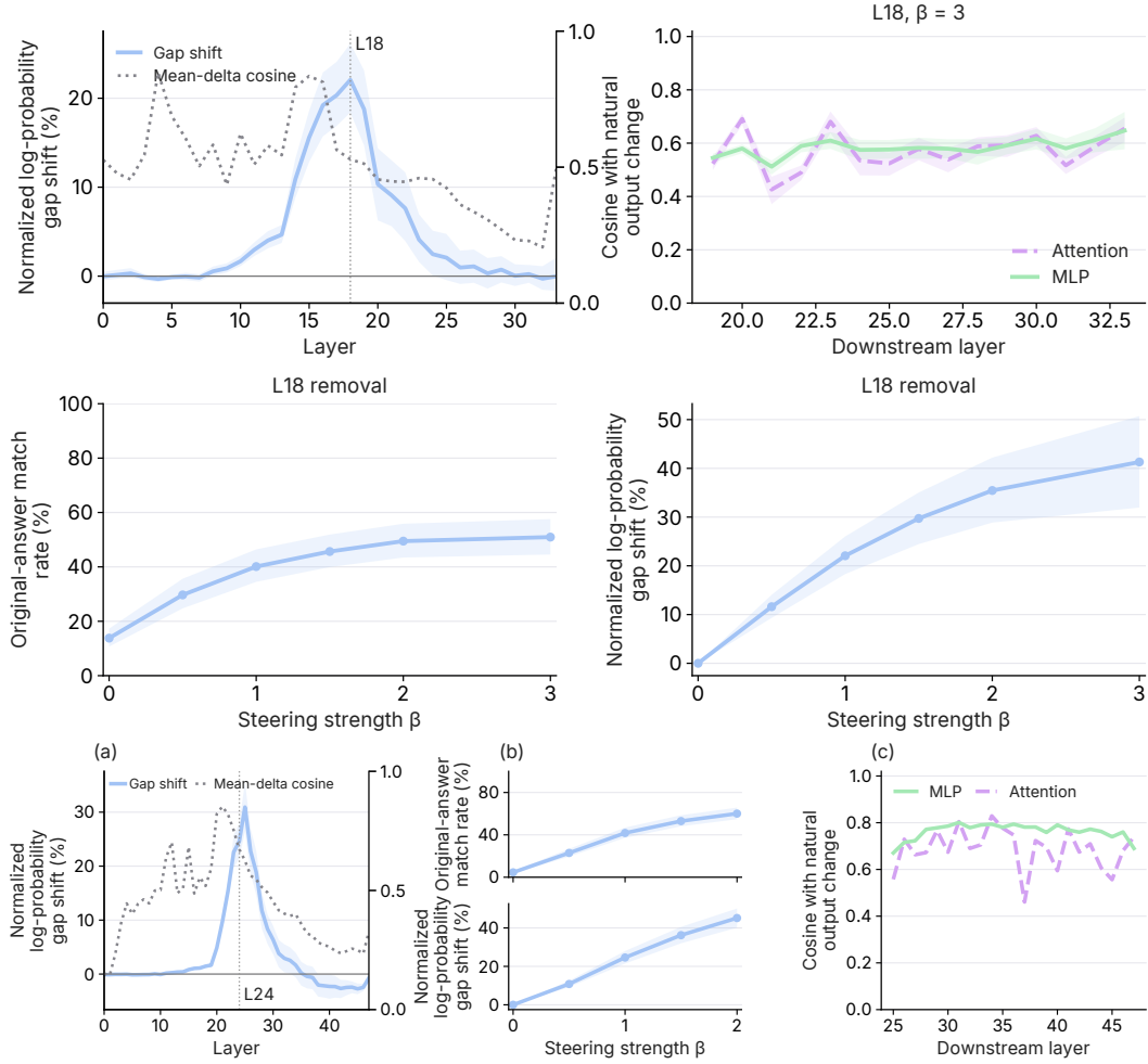
Figure 12: Negation-direction removal in Gemma 3-4B-IT (top) and Gemma 3-12B-IT (bottom). Dose layers are L18 and L24; downstream alignment uses \beta = 3 and \beta = 2 , respectively. Effects equally weight six benchmarks. Shading shows available 95% question-bootstrap intervals; Gemma 12B downstream cosine is shown without a pooled interval.
