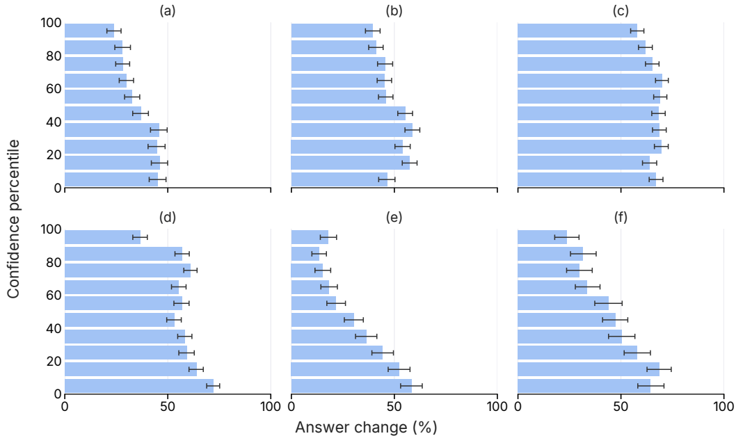
Figure 7: Answer change by confidence percentile for each model on the test split. Confidence is measured by mean token log-probability of the original answer, with percentiles computed within each model. We include only originally correct cases and average negation forms within each question. Error bars show 95% question-bootstrap intervals.
