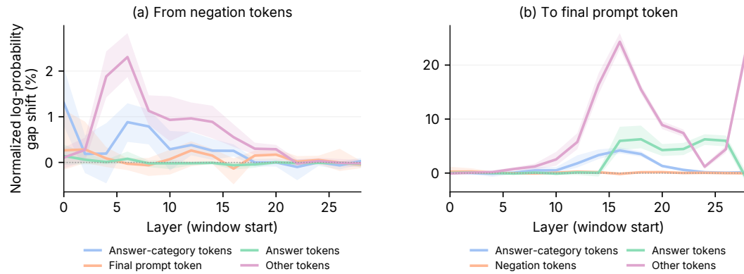
Figure 11: Information flow in Qwen3.5-9B, including softmax and linear attention. Final-position interventions continue during generation. Effects equally weight six benchmarks; shading shows 95% question-bootstrap intervals.
