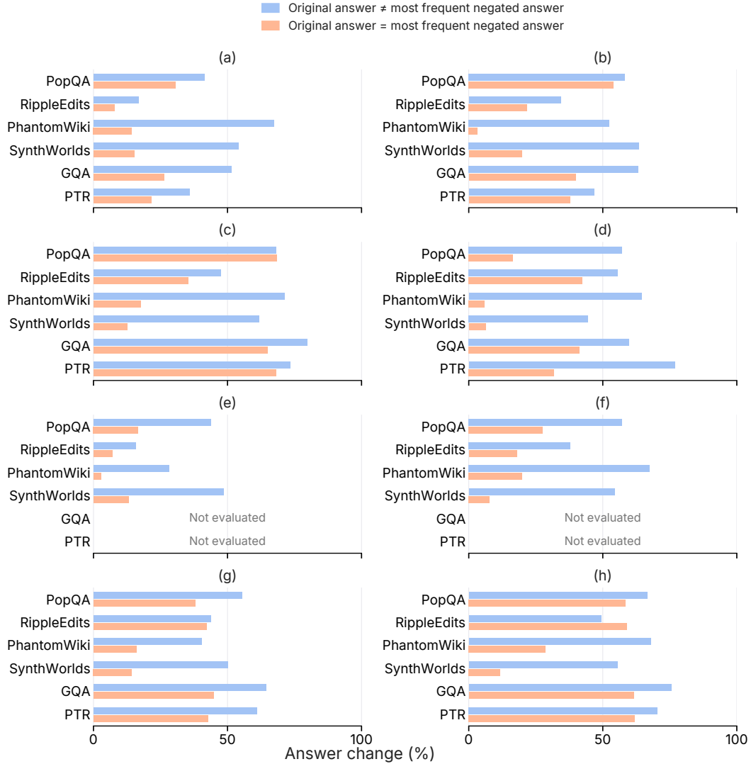
Figure 8: Answer change by model and benchmark on the test split. The most frequent negated answer is identified within each model’s relation/type group using its test outputs. Rates are computed over originally correct pairs with a judged repetition outcome. Not evaluated indicates unavailable model–benchmark results.
