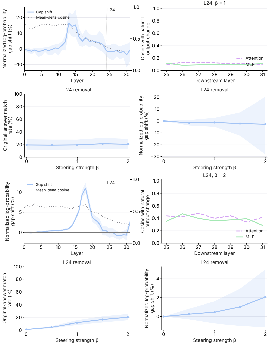
Figure 13: Negation-direction removal in Llama 3.1-8B-Instruct (top; four text benchmarks) and Qwen3.5-9B (bottom; six benchmarks). Both displayed dose experiments use L24. Downstream alignment uses \beta = 1 and \beta = 2 , respectively.
