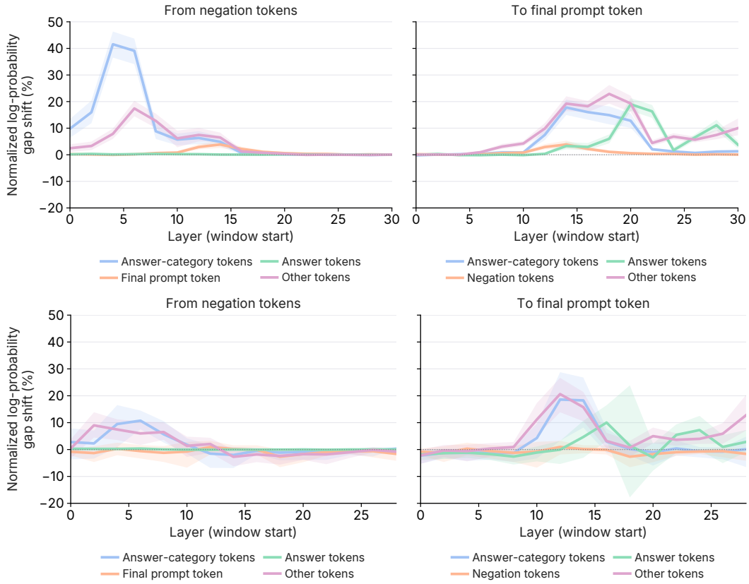
Figure 10: Information flow in Gemma 3-4B-IT (top) and Llama 3.1-8B-Instruct (bottom). Left: paths from negation tokens. Right: paths to the final prompt token. Curves show normalized log-probability gap shift; shading shows 95% question-bootstrap intervals.
