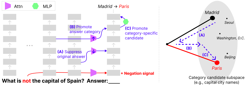
Figure 1: Overview of LLMs’ negation mechanism. Left: The negation signal triggers three downstream changes: (A) suppressing the original answer, (B) promoting answer category information, and (C) promoting a category-specific alternative. Right: These changes preserve the answer category subspace while shifting preference to an alternative answer (“Paris”).
