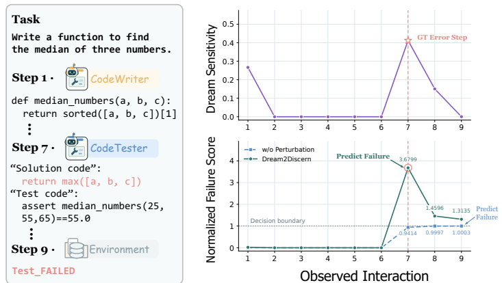
Figure 6. Case study of runtime failure prediction on a held-out coding trajectory from AFTRAJ-2K.
