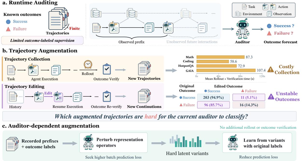
Figure 1. Motivation of Dream2Discern. (a) A runtime auditor predicts terminal outcomes from observed prefixes but learns from a limited labeled corpus. (b) Trajectory augmentation seeks broader failure coverage, but collection is costly and editing can invalidate outcome labels (right). Broader coverage alone does not identify prefixes that the current auditor finds hard to classify. (c) We construct hard latent variants through operator perturbations chosen to increase batch prediction loss, then train on these variants while keeping recorded prefixes and labels unchanged.
