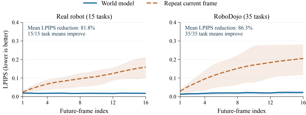
Figure 13: Prediction error over the full future horizon. Solid blue curves show the world model. Dashed orange curves show the LPIPS between the unchanged current image and each recorded future frame: the current image is reused as the future prediction, without model inference. Lines are task means, and shaded bands show the 25th–75th percentiles across the selected task windows, not confidence intervals. Both panels use the same vertical scale. Relative reductions use all 16 frames; the condition is excluded.
