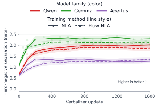
Figure 3: Better reconstruction accompanies more relevant information. Hard-negative separation across the 12 classification datasets for point-reconstruction NLA (solid) and Flow-NLA (dashed); higher is better.
