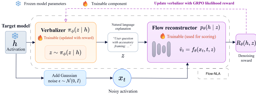
Figure 5: Learning activation explanations with Flow-NLA. An activation h from a frozen target model is passed to a verbalizer, which generates an explanation z , and corrupted with Gaussian noise to form x_t . The flow reconstructor learns to denoise x_t conditioned on z , modeling the distribution of activations compatible with the explanation. Denoising errors across noise levels define a reward derived from a conditional diffusion likelihood bound. This reward trains the verbalizer to produce explanations that make the observed activation more predictable under the conditional model.
