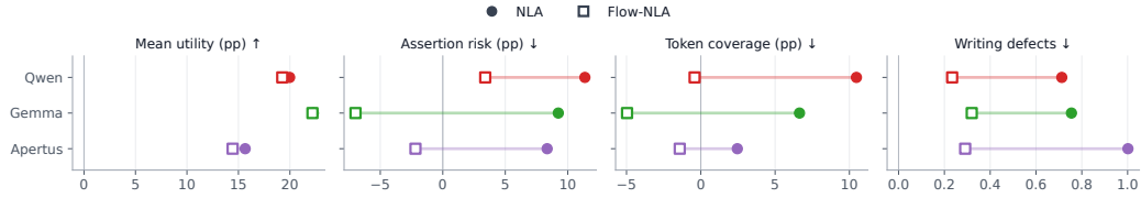
Figure 7: Changes from supervised initialization in mean utility, assertion risk, token coverage, and writing defects, averaged over the second half of the training range shared by both methods. Filled circles denote NLA; open squares denote Flow-NLA; lines show the gap between methods.
