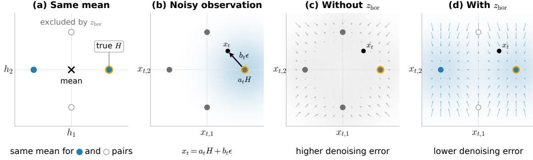
Figure 4: Denoising can reward information beyond the conditional mean. H is uniform over four unit directions; we follow the realized activation H = (1, 0) (gold outline). (a) The horizontal explanation z_{\text{hor}} keeps the horizontal pair (blue) and excludes the vertical pair (open circles). Both pairs have mean zero ( \times ), so the optimal expected point loss is the same with or without z_{\text{hor}} . (b) Denoising also observes the noisy activation x_t = a_t H + b_t \epsilon (black arrow: noise b_t \epsilon ), with candidates scaled by a_t . (c) Without the explanation, x_t is about equally close to the true and upward candidates, so the optimal estimate hedges between them. (d) With z_{\text{hor}} , the upward candidate is excluded and the estimate moves to the true direction, lowering the denoising error. In (c)–(d), arrows show the displacement a_t \mathbb{E}_\phi[H | x_t, z] - x_t from each noisy observation to its optimal signal estimate (without z in (c)); shading shows the density of x_t .
