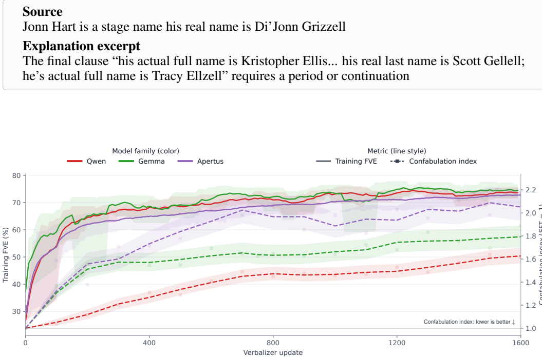
Figure 2: Better reconstruction accompanies more confabulation and writing defects. As the FVE reconstruction rises (solid line), so does the confabulation index (dashed line) across models. The index I(t) = \frac{1}{2}[R(t)/R(0) + D(t)/D(0)] averages assertion risk R and writing defects per explanation D relative to supervised initialization ( I = 1 ). Shading shows 95% bootstrap intervals.
