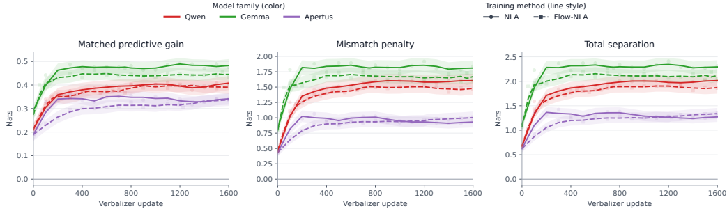
Figure 9: Matched predictive gain, mismatch penalty, and total hard-negative separation across the 12 classification datasets for point-reconstruction NLA (solid) and Flow-NLA (dashed). Curves are three-checkpoint means over raw markers; shading shows 95% bootstrap intervals.
