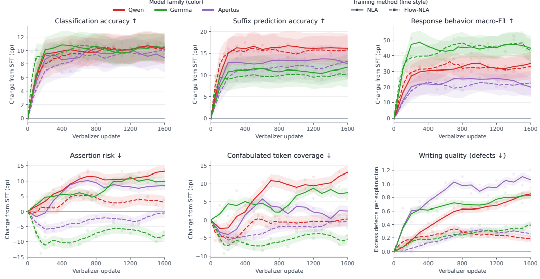
Figure 6: Changes in utility, confabulation, and writing defects from supervised initialization for point-reconstruction NLA (solid) and Flow-NLA (dashed). Markers show raw measurements, curves show three-checkpoint means, and shading shows pointwise 95% bootstrap intervals.
