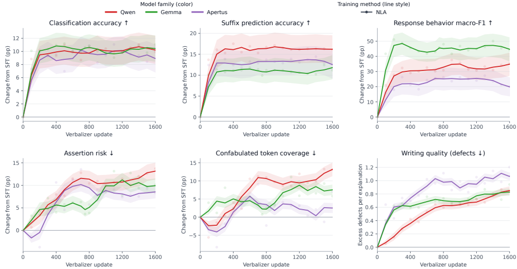
Figure 8: Changes in utility, confabulation, and writing defects from supervised initialization for the point-reconstruction NLA reruns. Shading shows pointwise 95% bootstrap intervals.
