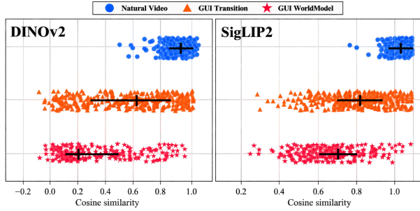
Figure 2: Natural videos exhibit strong temporal continuity, whereas GUI transitions show lower visual similarity and large variance, increasing the range of future appearance variations that must be modeled in pixel space.
