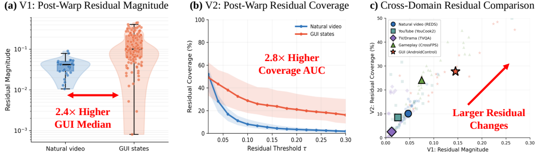
Figure A2: (a) GUI transitions exhibit stronger discontinuities than natural videos. (b) These GUI discontinuities also extend over broader spatial regions. (c) Across diverse visual domains, GUI dynamics show the highest degree of discontinuity, motivating latent-space GUI state forecasting.
