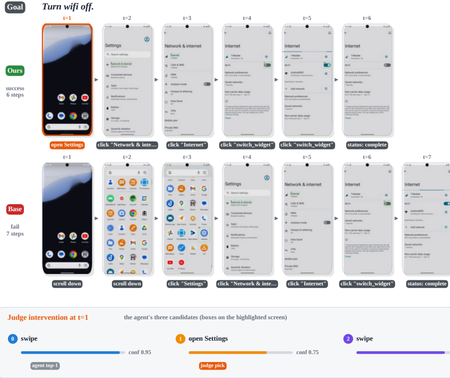
Figure A5: Same intervention, different task. After the same first-step correction, Ours turns Wi-Fi off and verifies the toggle state. Base reaches the same toggle but leaves Wi-Fi on before declaring completion.
