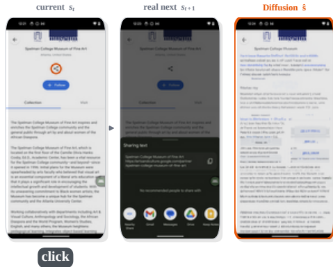
Figure A6: Identity shortcut of the diffusion-based world model (1/2).
