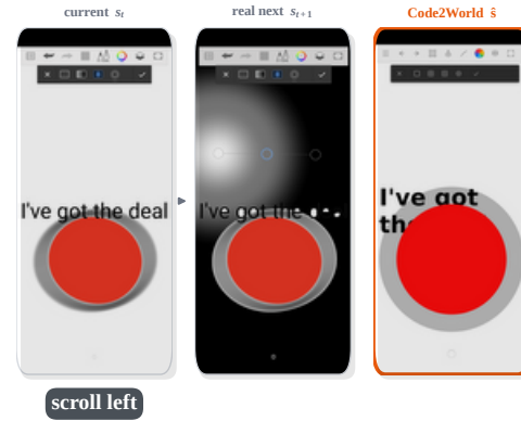
Figure A8: Code2World predictions on transitions with large real screen changes (1/2).
