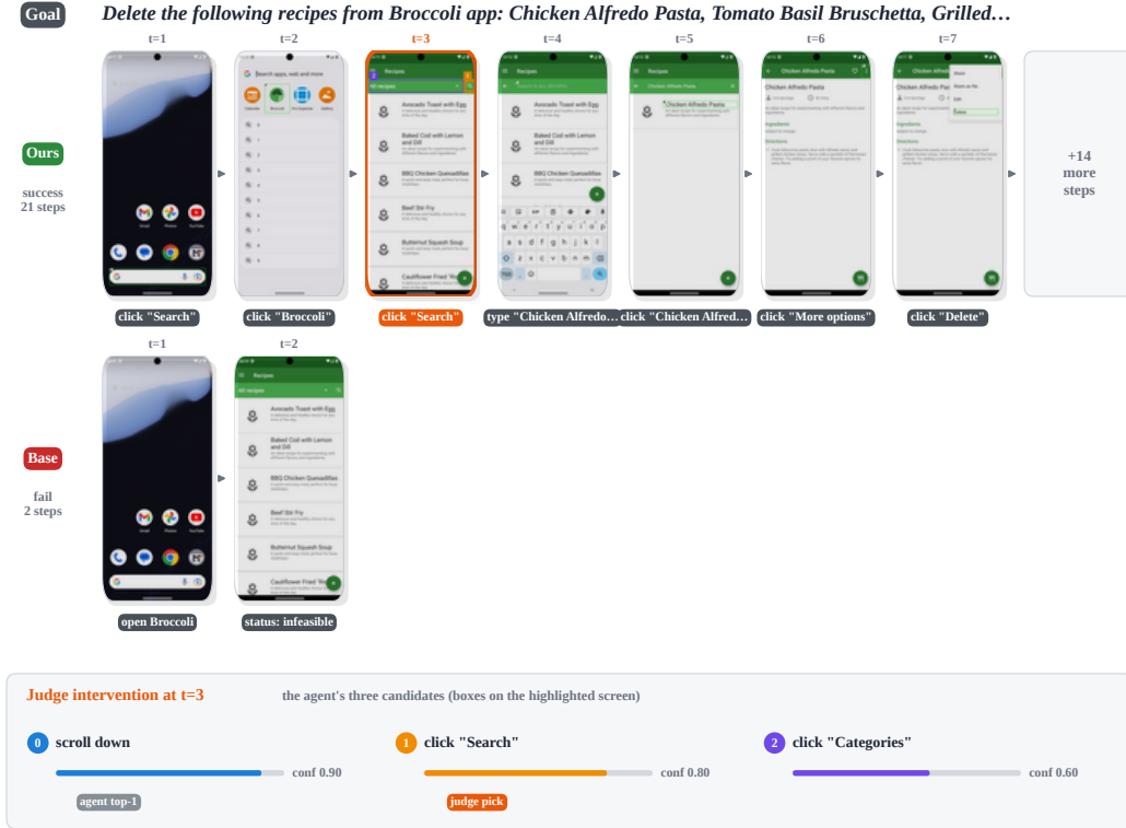
Figure A3: Long-horizon recovery. At step 3 the agent prefers to scroll the full recipe list; our model selects the search button instead. The agent then finds and deletes each recipe and completes the 21-step task, whereas Base declares the task infeasible at step 2.
