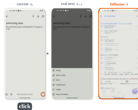
Figure A7: Identity shortcut of the diffusion-based world model (2/2).
