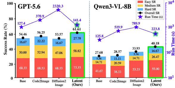
Figure 1: Our method, leveraging latent future-state representations, achieves the best GUI navigation performance with substantially improved efficiency.
