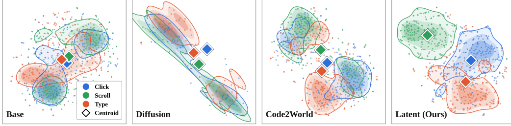
Figure 5: t-SNE visualization of action-induced future representations. Our model better aligns its predicted futures with action-specific clusters than the base agent and pixel-space world models.
