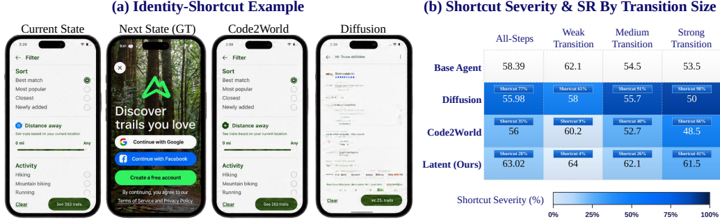
Figure 4: Identity shortcut and SR across GUI transition magnitudes. (a) Example of identity-preserving future prediction. (b) Downstream SR on a random 2.5K-sample AndroidControl subset. Shortcut severity is measured in each method’s native prediction space—pixel space for baselines and latent space for ours—as required by each formulation. In practice, larger transitions coincide with higher shortcut severity and lower SR, while ours substantially attenuates these trends.
