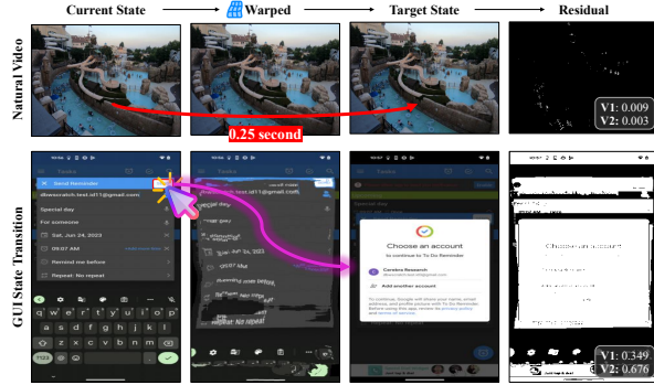
Figure A1: Natural video transitions are largely explained by pixel transport, resulting in small post-warp residuals. In contrast, GUI transitions induced by actions exhibit substantially larger residuals, revealing the inherently discontinuous nature of GUI dynamics.
