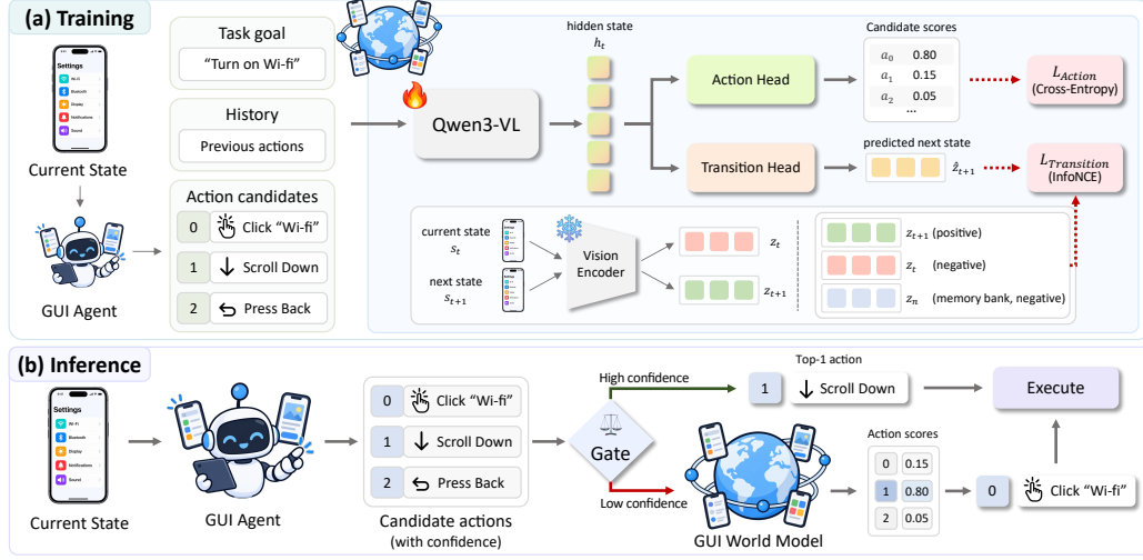
Figure 3: Overview of our latent world-action model for GUI agents. During training, we leverage a large multimodal model to learn action-specific shared representations through action scoring and contrastive future prediction. At inference, the transition head is removed for single-pass action scoring, while a confidence gate on the agent determines whether to invoke world-model rescoring.
