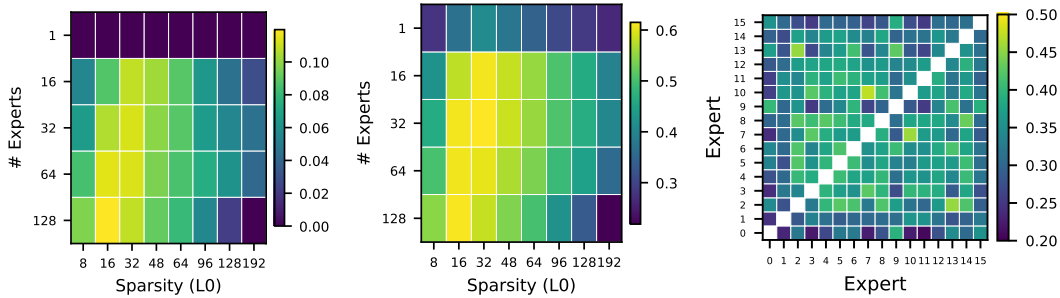
(a) Fraction of SAE decoder vectors with nearest neighbor cosine sim > 0.9 , width-matched SAEs. (b) Average cosine sim with nearest neighbor for decoder vectors, width-matched SAEs. (c) Average cosine sim between nearest neighbors across experts (16 experts, L0 = 64 ).
