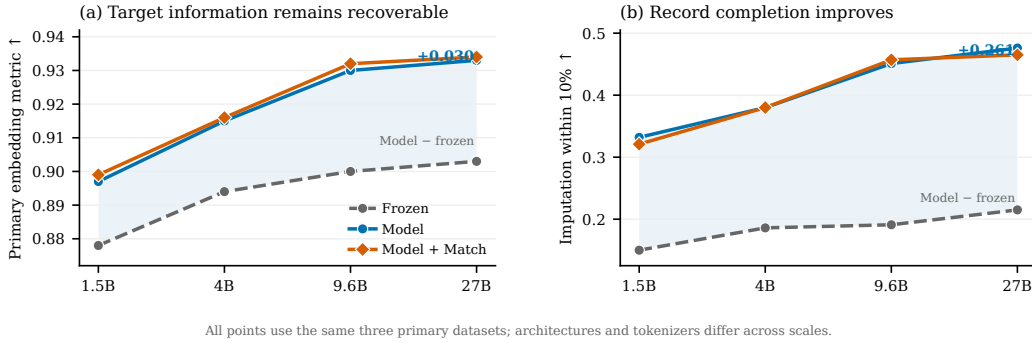
Figure 8: Fixed-order MODEL improves target prediction and record completion at every tested scale. Panel (a) reports the unweighted mean of MiniBooNE ROC–AUC, Superconductivity R^2 , and USDA R^2 ; panel (b) reports mean within-10% masked-value imputation on the same datasets. Gray dashed circles denote frozen checkpoints, blue circles denote fixed-order MODEL, and orange diamonds add MATCH. Relative to the frozen checkpoint, MODEL improves both metrics from 1.5B to 27B; adding MATCH produces only small and inconsistent changes. Lines connect separately trained checkpoint families whose architectures and tokenizers differ, so this is a one-seed robustness sweep rather than a fitted scaling law. MODEL denotes next-token record adaptation; MATCH denotes optional same-record consistency; and TUNE denotes supervised fine-tuning (SFT).
