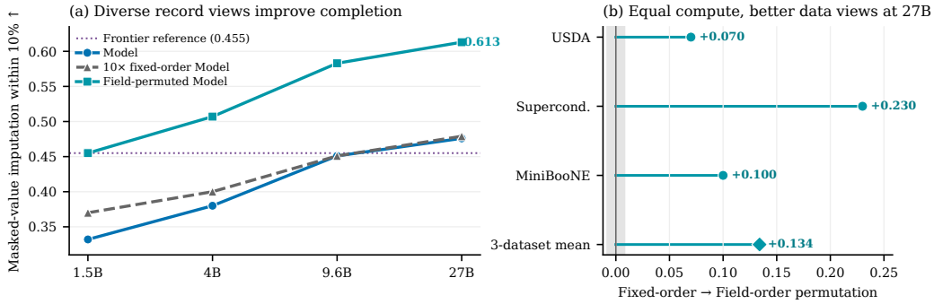
Figure 5: Field-order permutation improves completion beyond an equal-update fixed-order control. (a) Mean within-10% masked-value imputation over three-dataset from 1.5B to 27B, comparing standard fixed-order MODEL, extended fixed-order training, and field-permuted MODEL; the dotted line marks the 0.455 frontier-model reference used in this diagnostic. (b) At 27B, field-permuted MODEL improves every dataset over the equal-update fixed-order control, increasing the three-dataset mean by 0.134; the gray band marks the \pm 0.008 same-configuration imputation spread.
