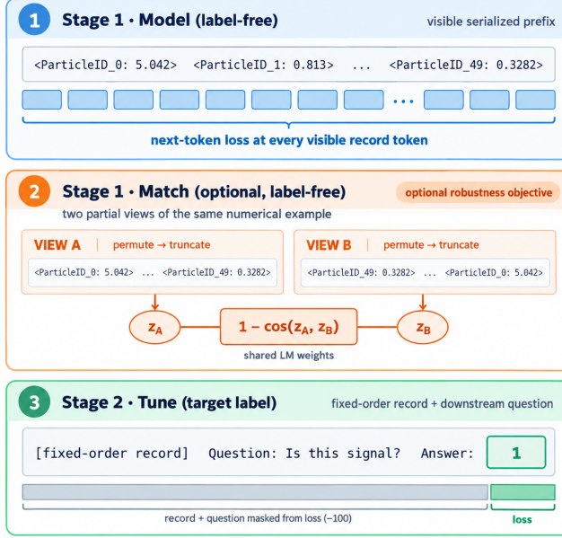
Figure 2: One numerical record supports three available training signals. MODEL applies next-token loss to every visible token in the truncated, label-free record. When partial-view robustness is desired, MATCH encodes two label-free permuted-prefix views with the same decoder and minimizes their cosine distance, without labels or negative pairs. TUNE returns to one fixed field order, masks the record and question tokens, and supervises only the label token.
