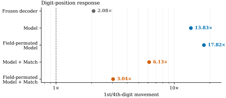
Figure 6: Digit-position sensitivity across selected 1.5B arms. MODEL produces the largest increase over the frozen checkpoint: both MODEL and field-permuted MODEL become more sensitive to a first-digit edit. Adding MATCH contracts the proxy for both MODEL and field-permuted MODEL. Every edited unit is complete in the encoded input and every variant changes one tokenizer token. MiniBooNE, 200 records; 95% paired record-bootstrap intervals are reported in Tab. 19. MODEL denotes next-token record adaptation; MATCH denotes optional same-record consistency; and TUNE denotes supervised fine-tuning (SFT).
