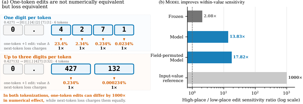
Figure 1: Token loss is numerically agnostic, but record-level adaptation improves magnitude sensitivity than target-only SFT. (a) With one digit per token, incrementing the first versus fourth fractional digit of 0.4271 produces a 1000\times difference in numerical effect. With groups of up to three digits, incrementing [427] versus [132] by one in 0.427132 also produces a 1000\times difference. Each intervention changes exactly one token. (b) We measure within-value sensitivity as the ratio between how far the pooled record embedding moves after a first-fractional-digit edit and after a fourth-fractional-digit edit. On the MiniBooNE diagnostic, applying the same objective densely through field-permuted MODEL increases this ratio from 2.08\times to 17.82\times at 1.5B. The 1000\times difference in numerical effect is a reference, not a required embedding-distance ratio. MODEL denotes next-token prediction on records, and field-permuted means reordering the attribute-value fields as data augmentation.
