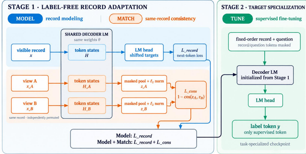
Figure 3: MoMaTune centers on MODEL → TUNE , with MATCH as an optional partial-view robustness component. Stage 1 always applies MODEL to label-free numerical records. Applications that require robustness to partial records can additionally apply MATCH . The resulting Stage-1 checkpoint initializes Stage 2, where TUNE presents a fixed-order record and target question and applies loss only to the label token.
