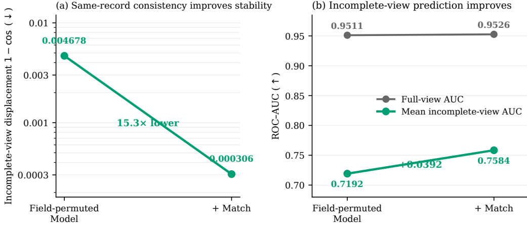
Figure 7: Same-record consistency improves incomplete-record stability and prediction when trained with permuted-prefix views. The matched field-permuted MODEL to field-permuted MODEL+MATCH comparison uses identical evaluation views and differs only by MATCH. Panel (a) reports incomplete-view displacement; lower is better. Panel (b) reports full-view and mean incomplete-view ROC–AUC from a logistic probe fitted on full-view embeddings; higher is better. MATCH reduces displacement by 15.305\times (95% CI [15.257\times, 15.354\times] ) and raises incomplete-view AUC by 0.0392 [0.0233, 0.0555] ; the full-view AUC difference is +0.00145 [-0.00453, 0.00763] . MiniBooNE, 3,000 records.
