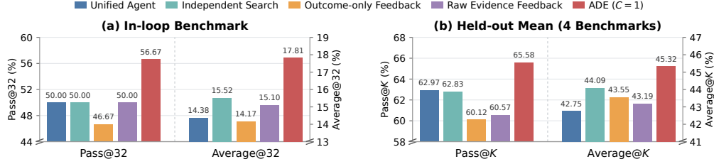
Figure 5: Data Selection–Math research organization and feedback comparisons. Each panel shows Pass@ K (left axis) and Average@ K (right axis); held-out scores average four benchmarks.
