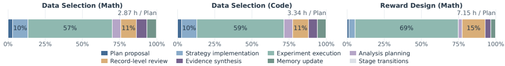
Figure 4: Estimated research-stage times at C = 1 . Each bar shows a task’s stage.
