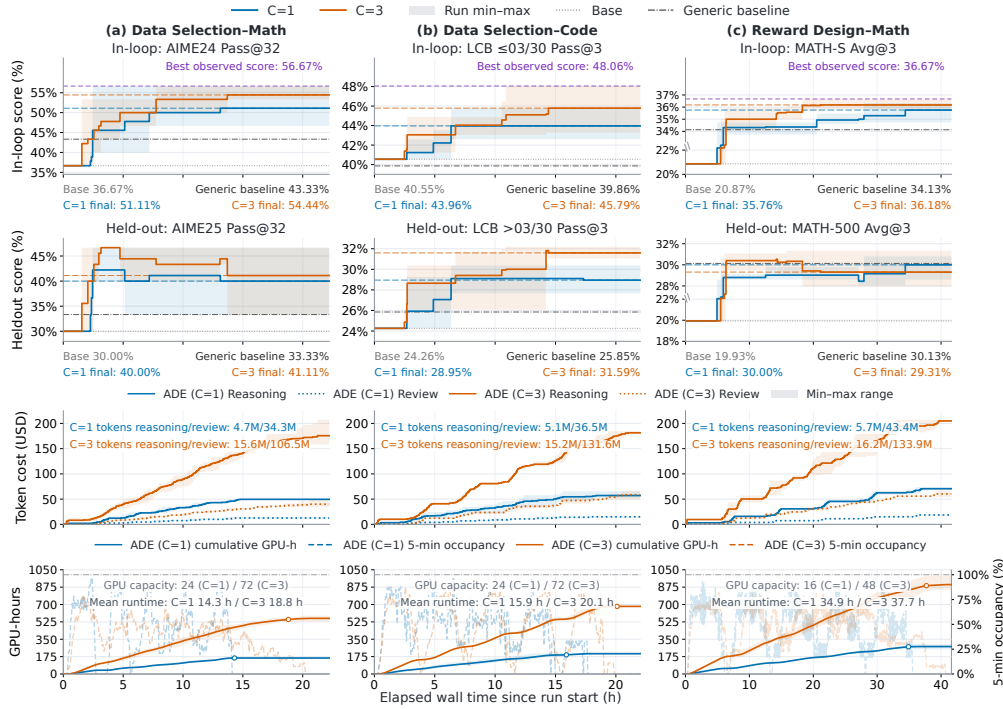
Figure 3: Research progress and cost for C = 1 (blue) and C = 3 (orange): rows show best-so-far in-loop scores, held-out scores of in-loop-selected models, cumulative token cost, and GPU-hours with allocation occupancy. Lines average three Runs per task and C ; shading shows min-max ranges.
