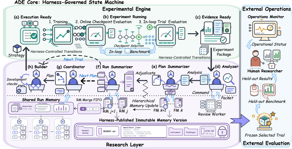
Figure 2: ADE under Harness control: Agents develop strategies using In-loop feedback and Memory; the Engine executes controlled experiments. Oversight and held-out evaluation remain external.
