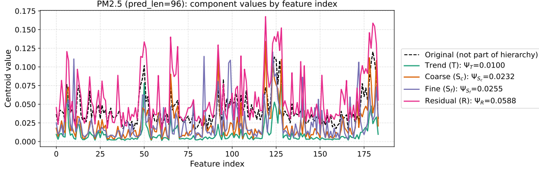
Figure 11: PM2.5 (184 channels, H = 96 ). The full ordering holds on average centroids: \Psi_T = 0.0100 < \Psi_{S_c} = 0.0232 < \Psi_{S_f} = 0.0255 < \Psi_R = 0.0588 .
