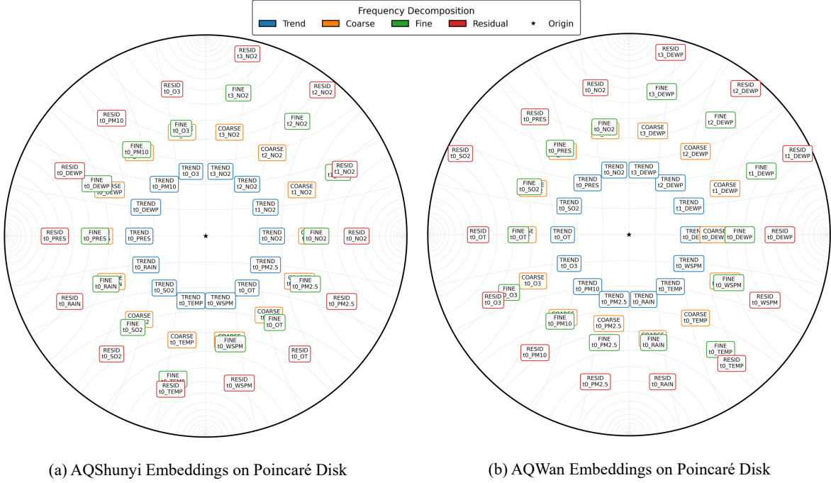
Figure 4: Each point is a (Scale, TimeSegment, Feature) tuple. The radial hierarchy shows our model learns frequency-based decomposition (Trend < Coarse < Fine < Residual). Labels follow t\{\text{segment}\}_{\text{feature}} (e.g., t_0_{\text{Feature}_1} = segment 0, feature 1).
