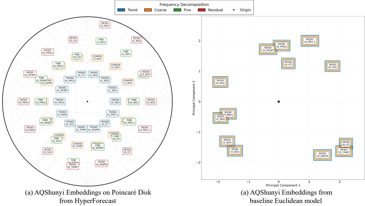
Figure 13: Segment embeddings learned on AQShunyi. Left: Poincaré disk from HyperForecast. Trend embeddings cluster near the origin, while coarse, fine, and residual components sit at increasing radii. Right: Euclidean PCA from the same architecture. All four frequency components collapse to coincident 2D positions, eliminating the radial hierarchy.
