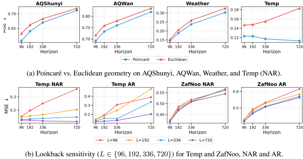
Figure 5: Ablation studies: (a) Hyperbolic vs. Euclidean geometry and (b) lookback window sensitivity, shown for both forecasting variants.
