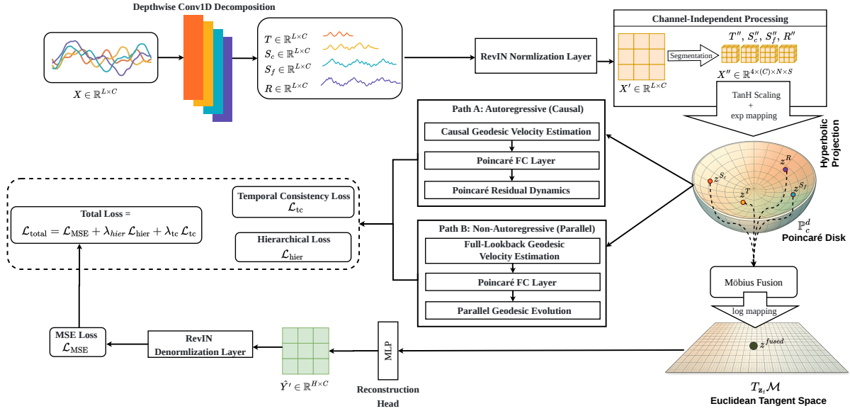
Figure 2: Overview of HyperForecast pipeline. Input \mathbf{X} \in \mathbb{R}^{L \times C} is decomposed into trend \mathbf{T} , coarse seasonal \mathbf{S}_c , fine seasonal \mathbf{S}_f , and residual \mathbf{R} components and normalized by a shared RevIN using statistics from the reconstructed signal \mathbf{X} = \mathbf{T} + \mathbf{S}_c + \mathbf{S}_f + \mathbf{R} . Each component is then segment-encoded, projected onto the Poincaré ball \mathbb{P}_c^d , forecast via geodesic dynamics on the manifold, and Möbius-fused before Euclidean decoding.
