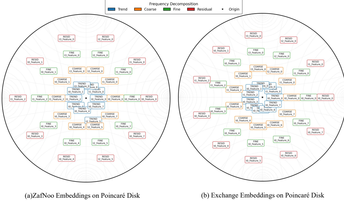
Figure 12: Each point represents a (Scale_TimeSegment_Feature) tuple at a specific frequency scale. Trend (innermost) captures low-frequency patterns closest to the origin, while Residual (outermost) encodes high-frequency noise farther from the origin. The radial hierarchy demonstrates that our model successfully learns frequency-based decomposition (Trend < Coarse < Fine < Residual). Node labels follow the format t\{\text{segment}\}_{\text{feature}} (e.g., t0\_Feature\_1 = time segment 0, feature 1).
