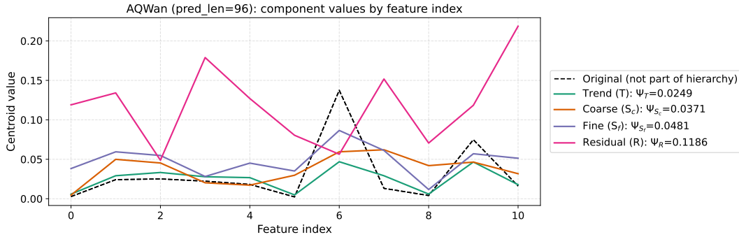
Figure 9: AQWan (11 channels, H = 96 ). The full ordering holds on average centroids: \Psi_T = 0.0249 < \Psi_{S_c} = 0.0371 < \Psi_{S_f} = 0.0481 < \Psi_R = 0.1186 .
