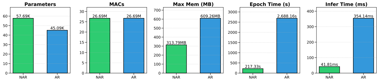
Figure 7: Efficiency of the two HyperForecast variants on Weather, \text{seq\_len}/\text{pred\_len} = 720/720 . NAR is shown in green and AR in blue.
