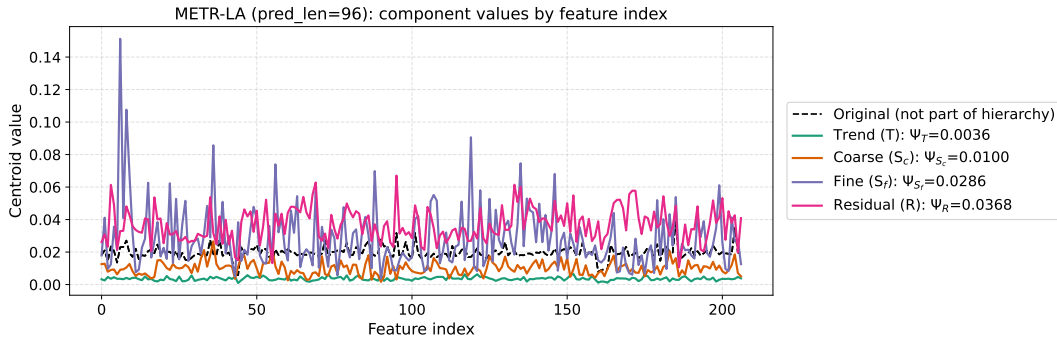
Figure 10: METR-LA (207 channels, H = 96 ). The full ordering holds on average centroids: \Psi_T = 0.0036 < \Psi_{S_c} = 0.0100 < \Psi_{S_f} = 0.0286 < \Psi_R = 0.0368 .
