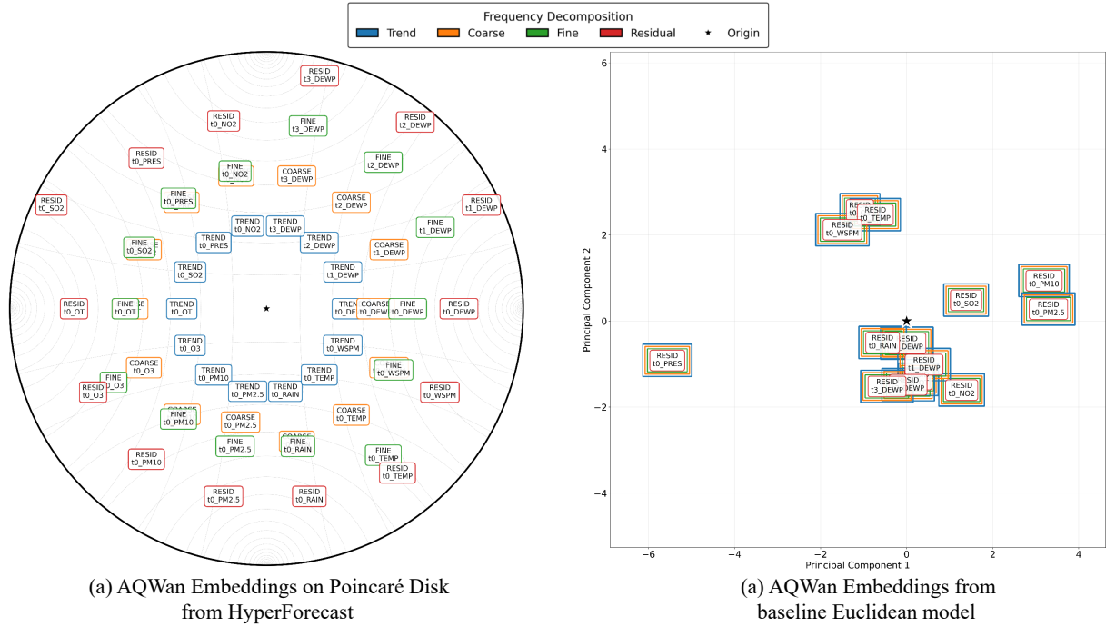
Figure 14: Segment embeddings learned on AQWan; conventions follow Figure 13. Similar radial ordering emerges in the Poincaré panel and is absent in the Euclidean PCA, where the four components stack at identical coordinates.
