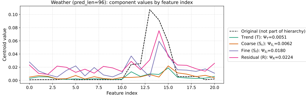
Figure 8: Weather (21 channels, H = 96 ). The full ordering holds on average centroids: \Psi_T = 0.0051 < \Psi_{S_c} = 0.0062 < \Psi_{S_f} = 0.0180 < \Psi_R = 0.0224 .
