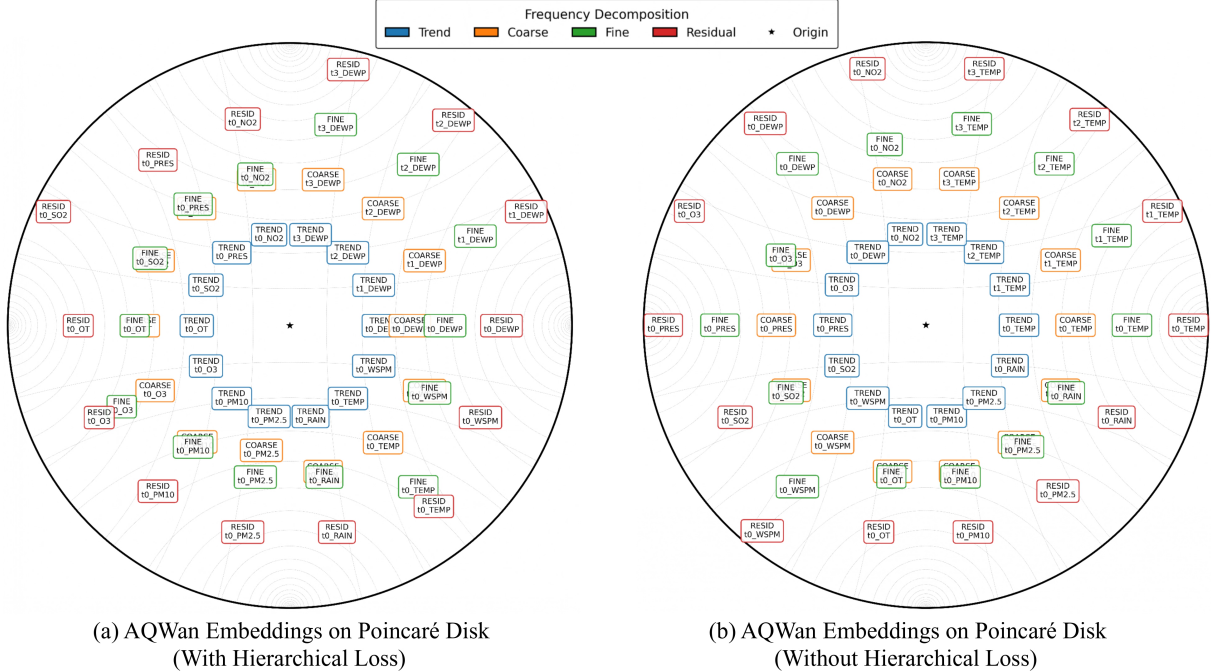
Figure 15: Poincaré-disk embeddings learned on AQWan with and without the hierarchical radial loss \mathcal{L}_{\text{hier}} .
