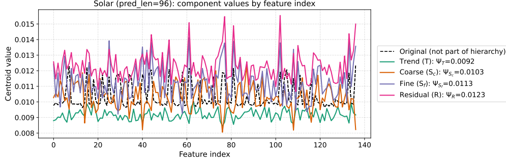
Figure 3: Per-feature Welch-PSD spectral centroid of each decomposed component on Solar (137 channels, H = 96 ). Black dashed: original (undecomposed) signal. Legend values are the per-component average across all 137 features. The ordering T < S_c < S_f < R holds on the dataset average and for the large majority of individual features.
