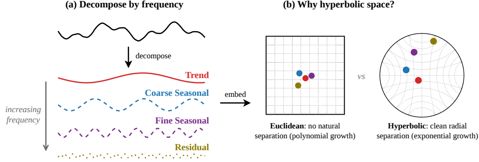
Figure 1: Multiscale temporal decomposition and geometric embedding in HyperForecast. (a) A time series is decomposed into trend, coarse seasonal, fine seasonal, and residual components with increasing frequency. (b) Euclidean space provides no natural separation of these components, whereas the Poincaré ball naturally separates them radially through its exponential volume growth.
