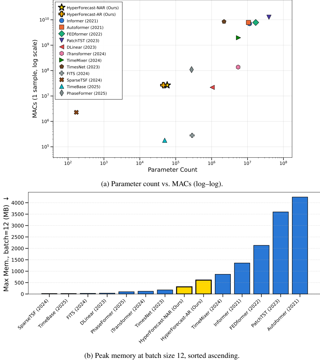
Figure 6: Efficiency comparison across all fourteen models on Weather ( \text{seq\_len} = \text{pred\_len} = 720 ). (a) Parameter count vs. MACs for a single sample. (b) Peak memory at batch size 12, sorted ascending.
