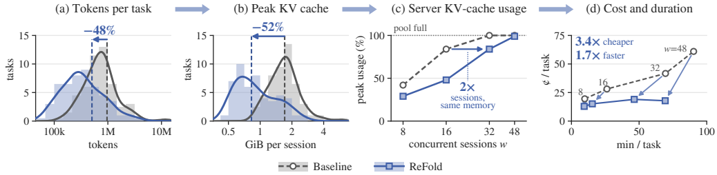
Figure 1: ReFold’s savings carry from one session to the serving system. With Qwen3.6-27B on SWE-bench Verified, it cuts (a) tokens and (b) peak KV cache per session, so a vLLM server (c) fits 2\times the sessions in the same memory and (d) runs tasks up to 3.4\times cheaper and 1.7\times faster.
