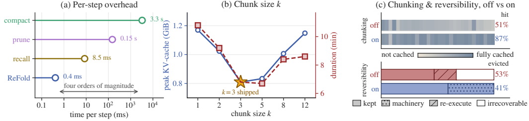
Figure 4: Ablation results. (a) Per-step context-management overhead on a log scale. (b) Peak KV-cache memory (left axis) and median duration (right axis) across chunk sizes on 20 tasks; the axes are scaled to coincide at k=3 . (c) Chunking (top) and reversibility (bottom) switched off and on.
