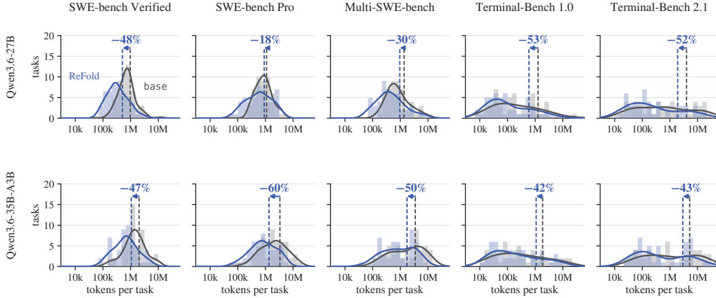
Figure 6: Tokens per task for every cell of Table 1. ReFold shifts the whole distribution toward fewer tokens rather than trimming a few long tasks.
