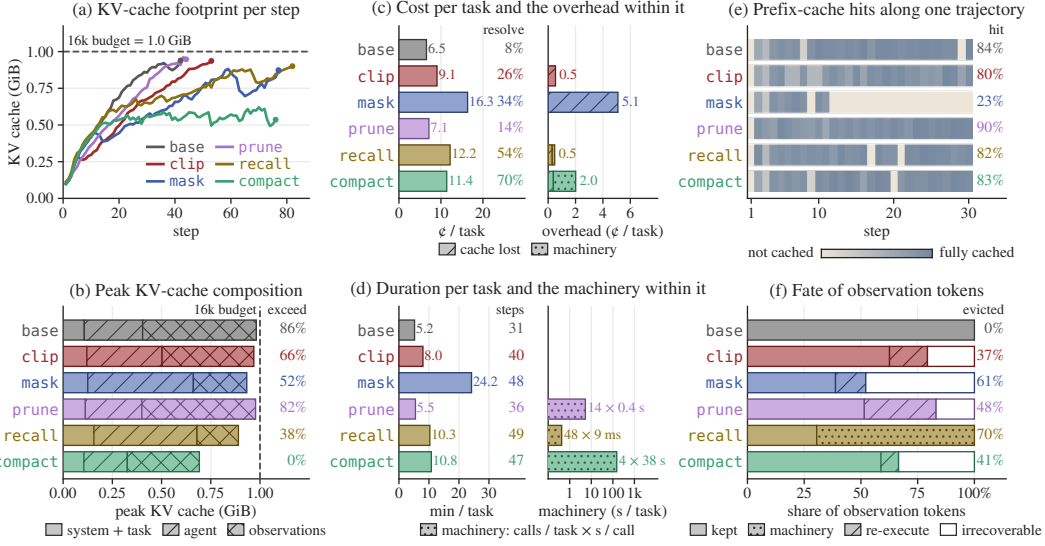
Figure 2: The six strategies on the same 50 SWE-bench Verified tasks at a 16k budget: per-session KV-cache footprint and peak composition (a, b), per-task cost and duration with resolve rate (c, d), prefix-cache reuse along one trajectory (e) and the fate of evicted observation tokens (f).
