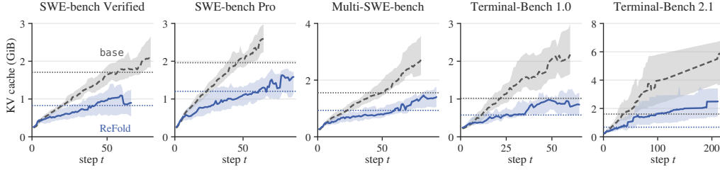
Figure 5: KV cache per session at every step with Qwen3.6-27B. The gap between base and ReFold widens with trajectory length, as base keeps everything it has read.
