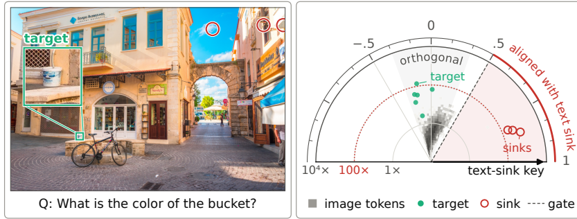
Figure 1: Visual attention sinks point the same way as the text-sink. Left: visual attention sinks (red, \geq 100\times uniform attention outside the target) and the target (green) in a V^* image. Right: key direction (angle) vs. attention (radius) of every image token
