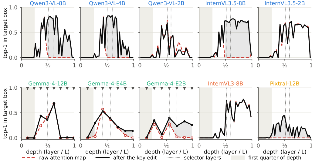
Figure 8: Per-layer top-1 localization on V^* for the raw map (dashed) and the cleaned map (solid). Here top-1 localization is the fraction of images whose most-attended image token lies in the target box. The shaded area between the curves is the gain from the key edit. Dotted lines mark the selector layers. The gray band is the first quarter of depth, which the peak-layer rule skips. Gemma-4 shows full-attention layers only (triangles).
