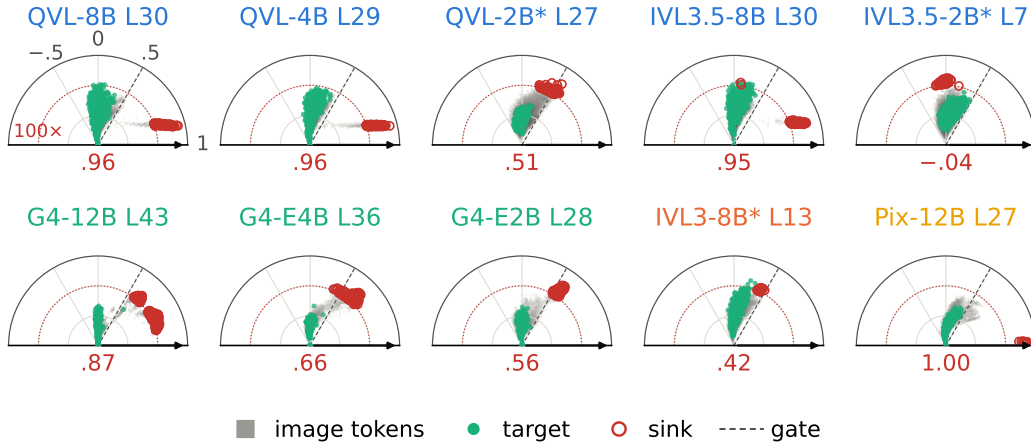
Figure 2: Image tokens on V* at each model’s peak layer. Angle: centered cosine of a token’s key with the text-sink key (Equation 2). Radius: attention received relative to uniform, log scale. Sinks: tokens above 100× uniform (dotted ring) outside the target box. Dashed ray: gate threshold .5. Red numbers: median cosine of the sinks; *: sink-free
