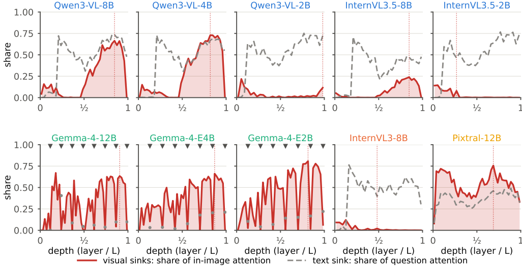
Figure 5: Sink attention across depth on V^* for all ten models. Red: visual attention sink share of in-image attention. Gray dashed: text-sink share of question attention. Dotted: peak layer. Gemma-4 reaches the text sink only in its full-attention layers (triangles). Title color marks the language-model backbone (Qwen3, Gemma-4, Qwen2.5 and Mistral).
