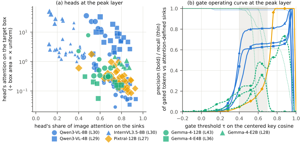
Figure 6: (a) Sink share vs. target attention per head at the peak layer on V^* . Marker size is the head’s share of image attention. (b) Precision and recall of the centered-cosine gate at threshold \tau_c against the attention-defined sinks, one curve per sink-bearing model on V^* . Shaded band: thresholds that give the same edit. The paper uses 0.5.
