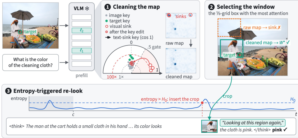
Figure 4: Overview of the entropy-triggered re-look. (1) The key edit removes the visual attention sinks from the prefill attention map. (2) The selector keeps the \frac{1}{3} -grid window with the most attention on the cleaned map. (3) When the next-token entropy first exceeds H_0 after c tokens of thought, the crop of that window is inserted into the chain of thought.
