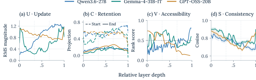
Figure 4: Layerwise representation profiles on Terminal-Bench with pointwise 95% task-bootstrap intervals; dashed and solid C curves denote response-start and response-end projections.
