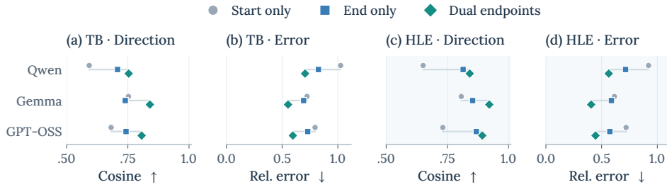
Figure 3: Endpoint approximations of mean response displacement across three models and two benchmarks; points and bars show task-balanced means and 95% task-bootstrap intervals. Layers 23, 22, and 8 are used for Qwen, Gemma, and GPT-OSS, respectively.
