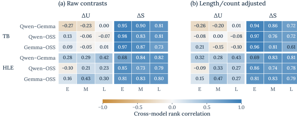
Figure 11: Cross-model correlations of same-task success-failure contrasts before and after adjustment for response length and analysis-center count. E/M/L denote early/middle/late depth bands. Every panel uses the same 34 Terminal-Bench and 208 HLE tasks; \Delta U provides the update-magnitude comparison.
