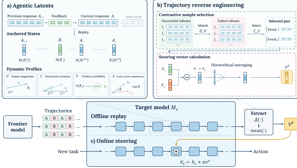
Figure 2: REVEAL reconstructs activation control from textual frontier-model trajectories. (a) Frozen replay yields Agentic Latents: anchored states and dynamic profiles. (b) Contrastive sample selection identifies matched local events; steering vector calculation combines their response-transition differences through hierarchical averaging. (c) The frozen target applies the resulting direction before each response.
