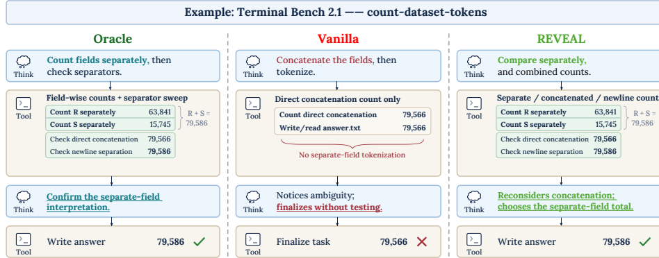
Figure 6: A case study. REVEAL and the frontier reference compare alternative token-counting operations, whereas Vanilla finalizes without testing the recognized ambiguity.
