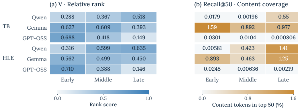
Figure 10: Task-balanced V and Recall@50 across early/middle/late depth bands on Terminal-Bench and HLE, using supported J-lens layers. Panels use separate linear scales; uniformly random vocabulary ranking has expected V = 0.5 .
