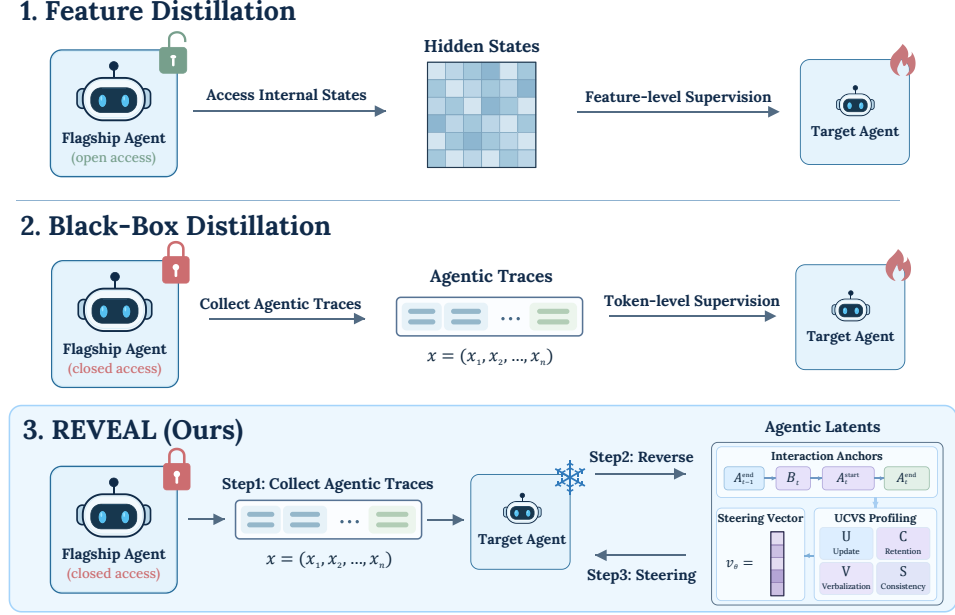
Figure 1: Three routes for reusing frontier-model experience: (1) feature distillation trains on internal states; (2) black-box distillation trains on textual trajectories; (3) REVEAL characterizes Agentic Latents through frozen target-model replay of textual trajectories and derives steering directions.
