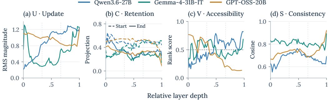
Figure 8: Full-depth HLE profiles with pointwise 95% task-bootstrap intervals. Dashed and solid C curves mark response start and end, respectively. U/C/V use 1,303 tasks; S uses 1,091 with valid adjacent updates. Only horizontal depth is rescaled; V excludes unsupported final layers.
