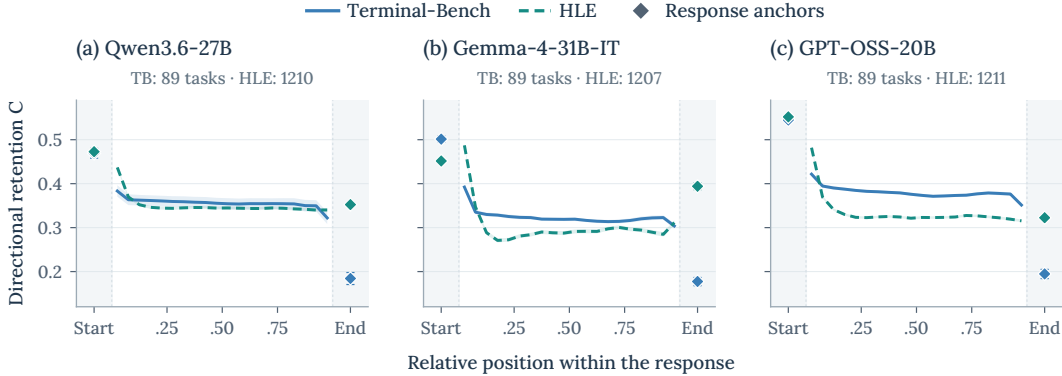
Figure 9: Within-response retention at layers 23/22/8 for Qwen/Gemma/GPT-OSS. Lines show 20 relative-position bin means; separate diamonds mark the response-start and response-end anchors. All recorded events with at least 20 content tokens are included. Shading and bars show 95% task-bootstrap intervals.
