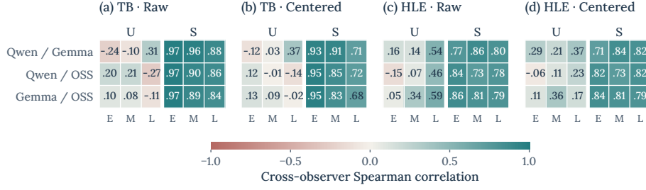
Figure 5: Cross-model Spearman correlations of trajectory-level U and S across depth bands, before and after task centering on matched trajectories. E/M/L denote early/middle/late bands.
