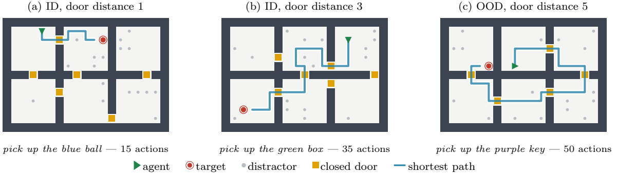
Figure 3 Representative BabyAI evaluation layouts at increasing door distance. The blue line is the shortest collision-free path from the agent to a cell adjacent to the target; the action count below each panel additionally includes turns, door toggles, and the final pickup. The path crosses one, three, and five doors respectively, which is what door distance measures. Every layout holds the same inventory of 18 objects, so distractor identities carry no information and only the spatial arrangement and the choice of target vary. The agent never observes this map: it receives a textual egocentric description (Figure 4).
