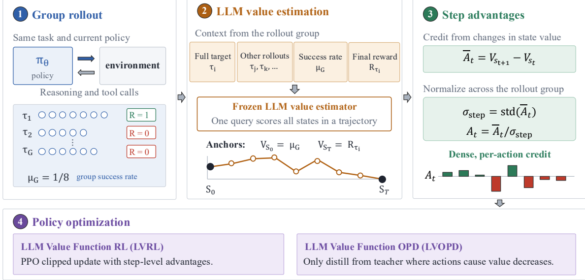
Figure 1 Overview of the proposed framework. (1) Group rollout: We sample a group of trajectories from the current policy and use their sparse outcome rewards to compute the empirical group success rate \mu_G . (2) LLM value estimation: A frozen LLM critic scores all trajectory states, conditioned on group context. Estimates are anchored to empirical outcomes: the initial-state value to the group success rate and the terminal-state value to the actual reward. (3) Step advantages: We compute unnormalized step advantages as consecutive value differences ( \bar{A}_t = V_\phi(s_{t+1}) - V_\phi(s_t) ) and normalize them across the group, yielding a dense, per-action credit signal. (4) Policy optimization: These step-level advantages drive standard PPO updates in LVRL, or act as a gating mechanism in LVOPD to restrict teacher supervision to actions that decrease the estimated value.
