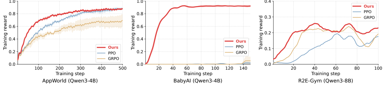
Figure 9 RL training reward curves across three training environments. For AppWorld and BabyAI, curves show the mean over three seeds; shaded regions denote one standard deviation.
