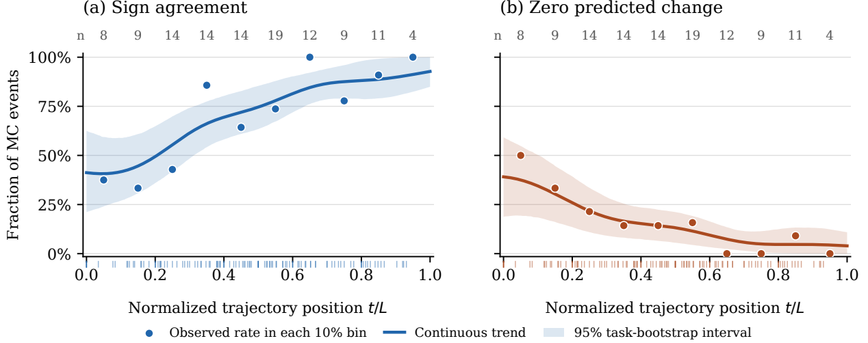
Figure 11 Agreement between predicted value changes and Monte-Carlo events across normalized trajectory position t/L , where L is the number of actions. (a) Fraction of MC events in each position bin for which the predicted value changes in the same direction as the MC estimate: a decrease for pitfalls and an increase for recoveries. (b) Fraction of MC events for which the model predicts no value change ( \Delta_t^{\text{pred}} = 0 ), despite an MC increase or decrease large enough to meet the event threshold ( |\Delta_t^{\text{MC}}| \geq 3\sigma ).
