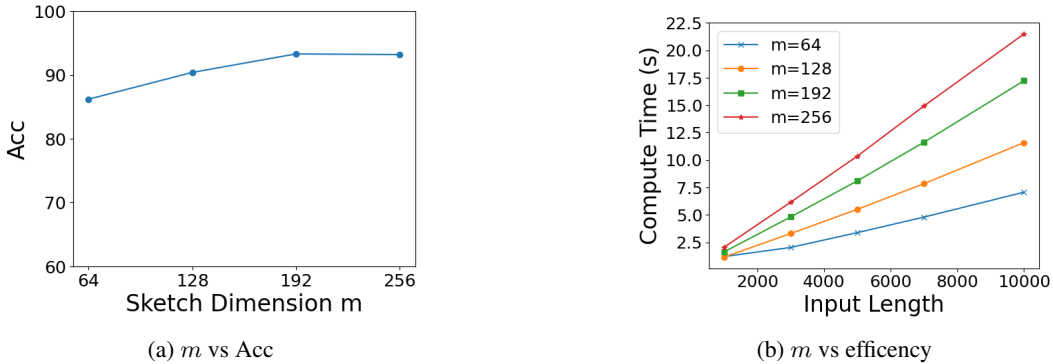
Figure 3: Results of how accuracy and forward time changes with sketch dimension m \in \{64, 128, 192, 256\} and d = 128 , p = 4 .
