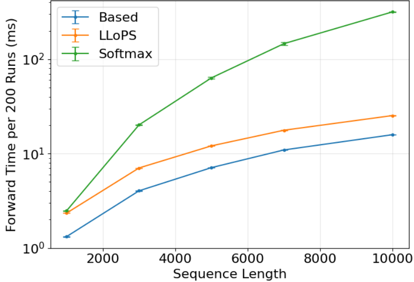
Figure 2: Time cost of different attention kernels at different input length with p = 2 .
