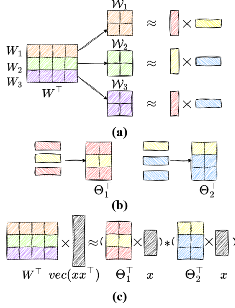
Figure 1: Illustration of LLoPS with an example where p = 2, d = 2, m = 3 . (a) Given the optimal linear projection matrix W , each column of W can be written as a 2 by 2 matrix, and be approximated by its rank-1 CP decomposition; (b) The rank-1 CP decomposition can be stacked into two weight matrices \Theta_1, \Theta_2 ; (c) In this way, the linear projection W^T \text{vec}(xx^T) can be approximated as (\Theta_1^T x) * (\Theta_2^T x) where * is an element-wise product.
