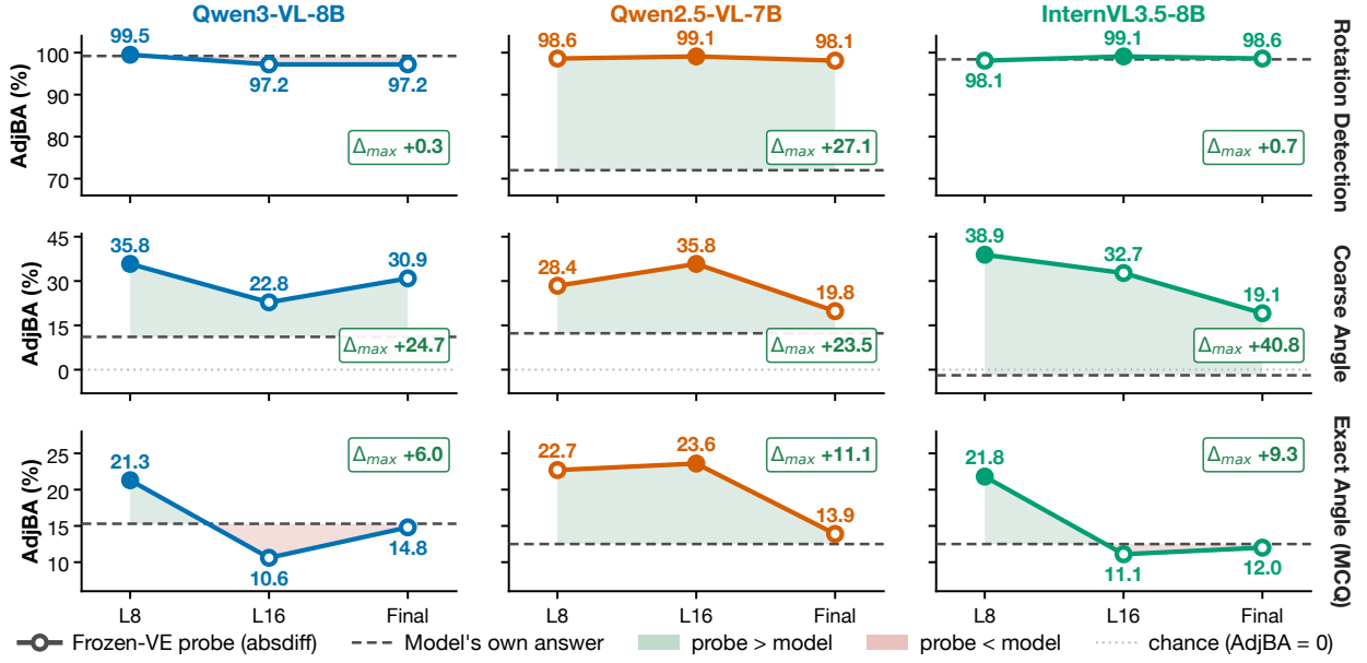
Figure 4 | Linear probe accuracy at L8, L16, and the final VE layer, with the model’s own answer as a reference. Recoverability declines from Rotation Detection to Coarse Angle to Exact Angle.
