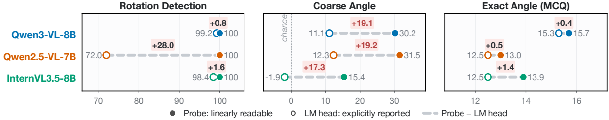
Figure 5 | Probe vs. LM head at h_{pre} . Probe (filled) and LM head (open) are two linear heads reading the same pre-answer representation. The gap is largest on Coarse Angle.
