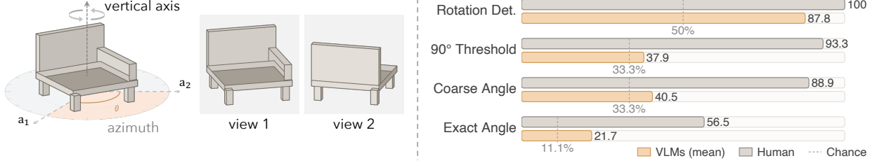
Figure 1 | Object-rotation reasoning in OR-Bench. Left: two views of the same object under azimuth rotation. Right: VLMs detect rotation reliably, but performance drops sharply once rotation magnitude must be estimated, even coarsely, leaving a large gap to humans.
