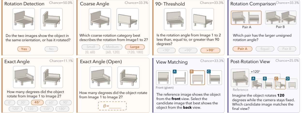
Figure 2 | Overview of OR-Bench. Eight tasks span two-view rotation understanding (orange) and multi-view rotation use (purple), covering multiple levels of answer granularity, from detecting whether a rotation occurred to specifying its exact angle.
