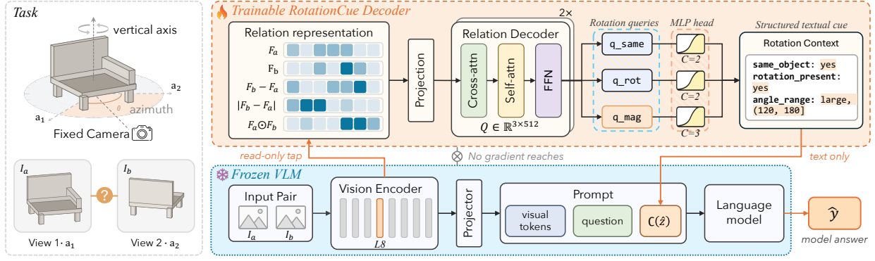
Figure 6 | RotationCue. The relation representation is read from vision layer L8 and passed to a lightweight decoder, without modifying the frozen VLM. Three learnable rotation queries predict a three-field rotation context, which is reinjected into the VLM as text only.
