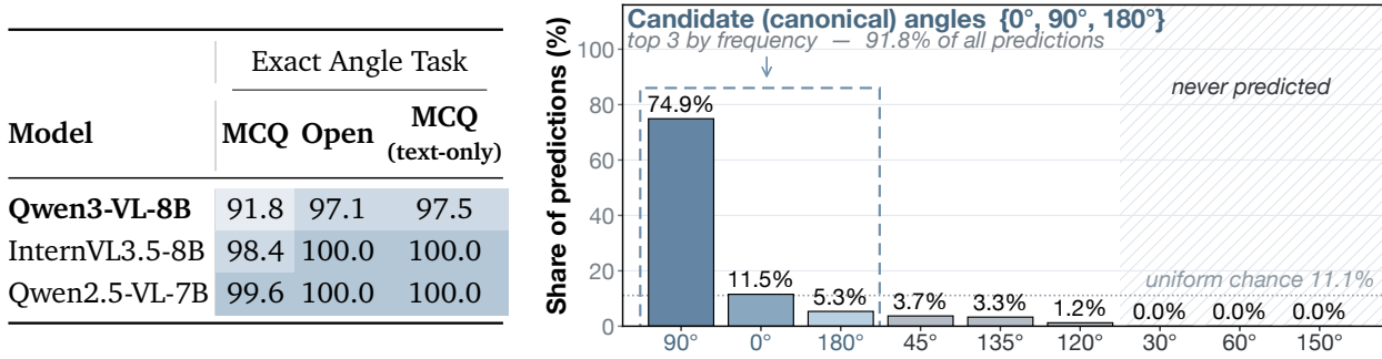
Figure 3 | Canonical-angle collapse across input and response settings. Left: share of predictions in the canonical set \{0^\circ, 90^\circ, 180^\circ\} ; darker cells indicate stronger collapse. Right: Qwen3-VL-8B’s Exact Angle (MCQ) predictions concentrate primarily at 90^\circ .
