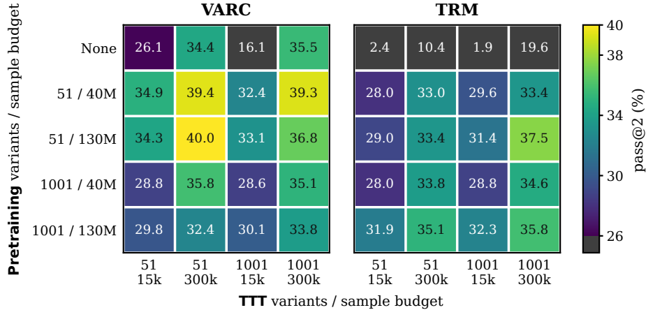
Fig.3. Performance under fixed pretraining and TTT budgets. We report pass@2 results for VARC and TRM. Rows vary the pretraining task-variant count V and sample-presentation budget B ; columns vary them for TTT. Both tables use a shared linear 26–40% scale, with values below 26% shown in dark grey.
