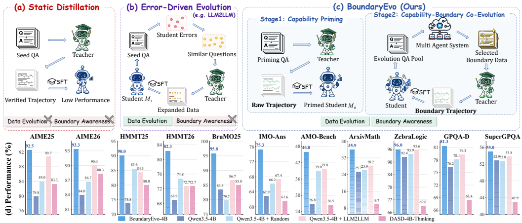
Figure 1: BoundaryEvo evolves supervision along the capability boundary of the student model. (a-c) Comparison with static distillation and error-driven acquisition, BoundaryEvo dynamically adapts supervision according to the evolving capability boundary of the student model. (d) BoundaryEvo-4B consistently outperforms strong baselines across various reasoning benchmarks.
