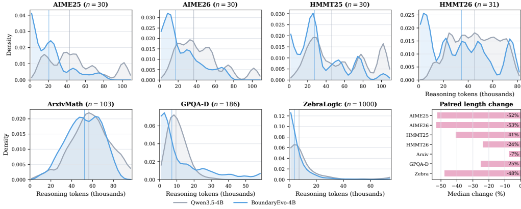
Figure 5: Reasoning-length distributions on matched evaluation questions. Curves show smoothed densities of per-question reasoning-token counts, and vertical lines mark medians. The final panel reports the relative change in median length from Qwen3.5-4B to BoundaryEvo-4B. Repeated rollouts of the same question are summarized by their median before plotting.
