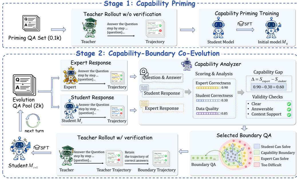
Figure 2: Overview of BoundaryEvo. Stage 1 performs judge-free teacher distillation to obtain the capability-primed checkpoint. In Stage 2, responses from the current student and a fixed expert are used to judge the candidate QAs, from which replay and novel records are selected for multiple teacher rollouts. The resulting trajectories are then independently verified against reference answers, and only those that pass verification supervise the next student.
