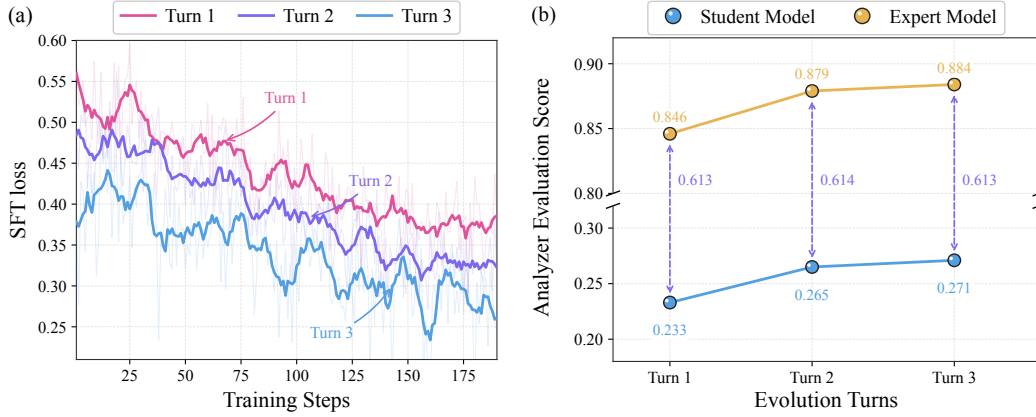
Figure 3: Training and selection dynamics across the Stage 2. (a) SFT loss for representative runs. (b) Mean student and expert scores on each turn. Annotations show the score gap.
