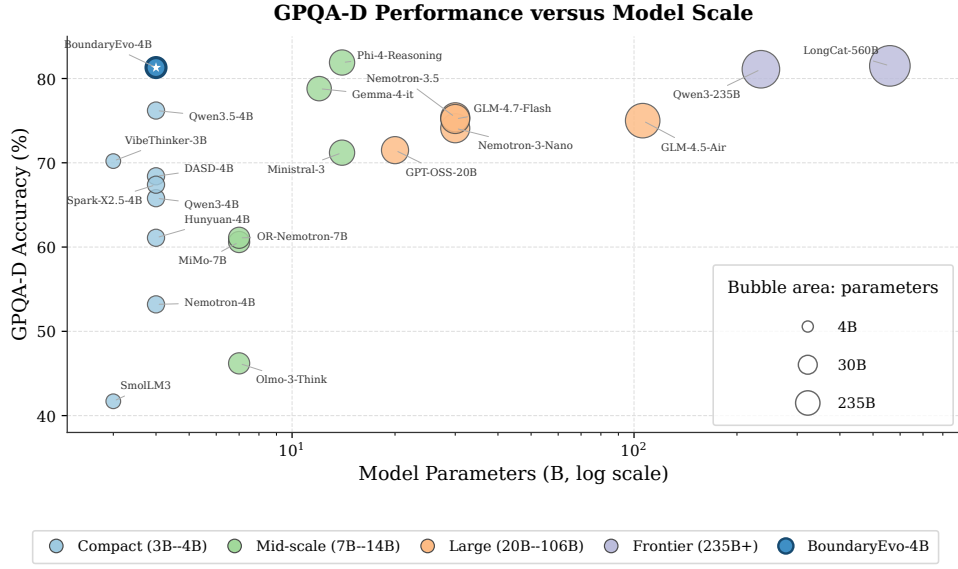
Figure 6: GPQA-D performance versus model scale. The horizontal axis is logarithmic, bubble area encodes parameter count, and color denotes the parameter range. BoundaryEvo-4B is highlighted with a white star. Only models with both a reported parameter count and GPQA-D score in Table 1 are included.
