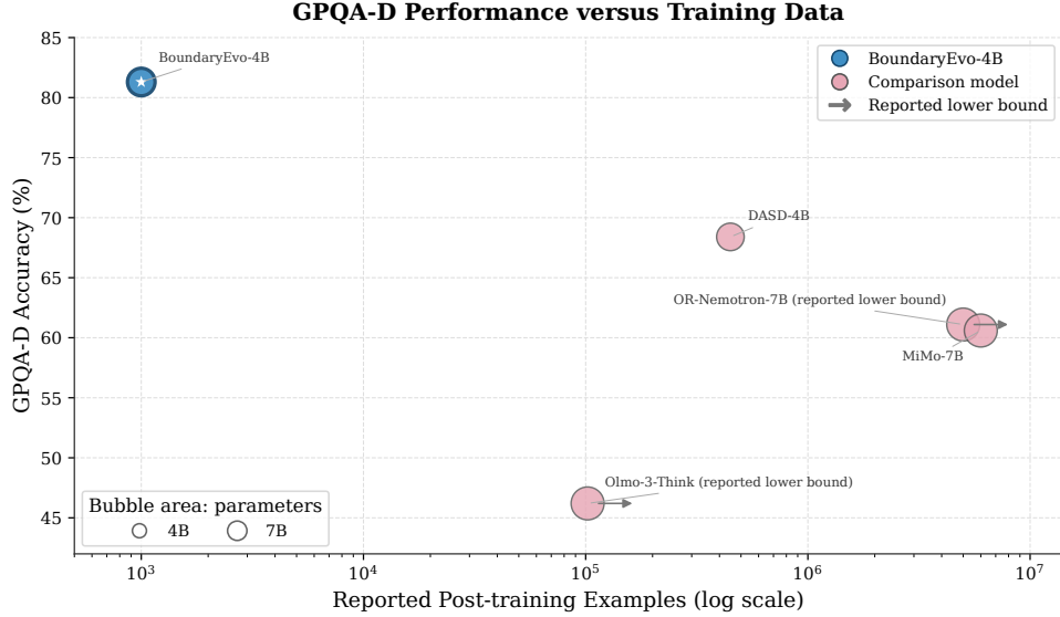
Figure 7: GPQA-D performance versus publicly reported reasoning post-training data. The horizontal axis is logarithmic and bubble area encodes model parameters. Right-pointing arrows mark reported lower bounds rather than exact dataset sizes. Only systems with disclosed data amounts and GPQA-D scores in Table 1 are shown.
