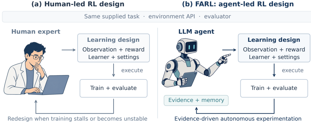
Figure 1: Automating the RL design loop. (a) An expert revisits the learning setup when training stalls or becomes unstable. (b) FARL’s LLM agent designs and directs experiments using behavioral evidence and scientific memory. Both receive the same task interface and evaluator.
