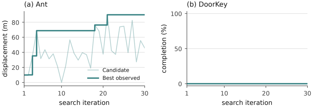
Figure 5: All 30 LiMEN search evaluations in Ant and DoorKey. Faint lines connect candidate results; dark lines show the best observed result. The horizontal axis counts search iterations.
