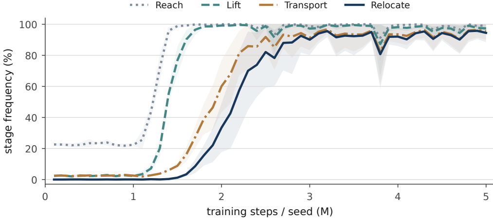
Figure 8: Learning progress of the Hand design selected at iteration 13. Lines and bands are three-seed means and SDs of 100k-step training frequencies. The objective completion curve shows how training extends beyond lifting and transport to sustained relocation.
