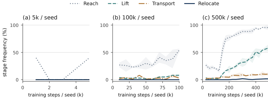
Figure 6: Early Hand learning within three independently trained cohorts of the retained design 031b6a159bb610d7: iteration/trial 0/165 at 5k, 1/1 at 100k, and 4/1 at 500k. Curves are marginal stage-completion frequencies from all recorded training episodes, using nonoverlapping 1k-, 10k-, and 25k-step windows, respectively. Each seed contributes 25, 500, or 2,500 episodes in the corresponding panel. Lines average equally across the one, two, or three training seeds; bands show sample SD where multiple seeds are available. Each panel starts with a fresh policy and uses its own executed training configuration. The panels are separate training histories, rather than checkpoints of one continuously trained policy; saved-policy evaluations are reported separately.
