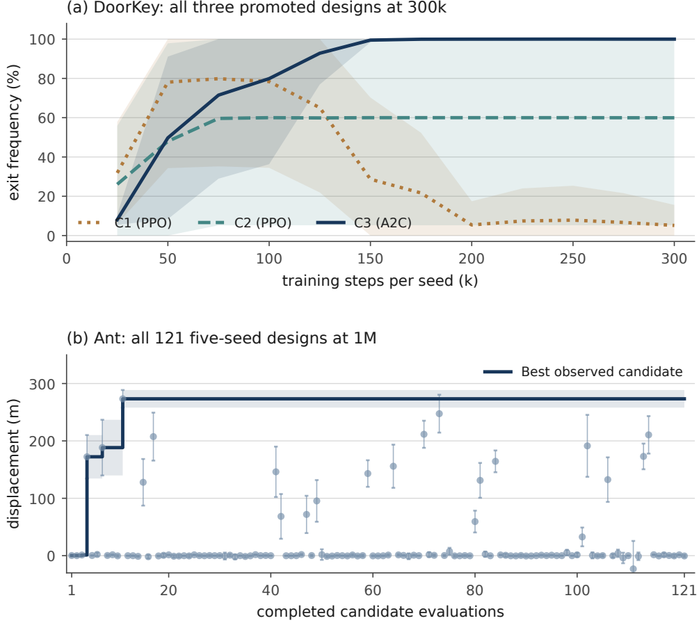
Figure 4: Candidate learning and selection at fixed training budgets. (a) DoorKey: five-seed mean exit frequency and sample SD for each of three 300k candidates. (b) Ant: all 121 candidate evaluations at 1M, with their five-seed SDs; the step line tracks the incumbent. The horizontal axes are policy-training steps in (a) and completed candidate evaluations in (b).
