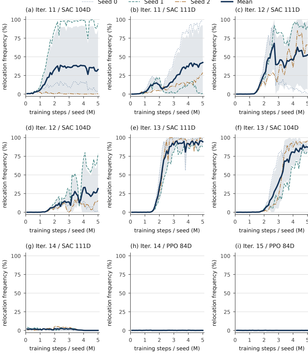
Figure 7: Learning curves for nine of the ten completed 5M Hand configurations. The final raw-input SAC configuration is reported in Table A21. Thin curves are the three training seeds, the thick curve is their mean, and shading is sample SD. Each point aggregates a 100k-step training window. Iteration 12 panels (c–d) form the matched representation experiment. Panel (e) is the selected design; panels (g–i) show the later completed alternatives.
