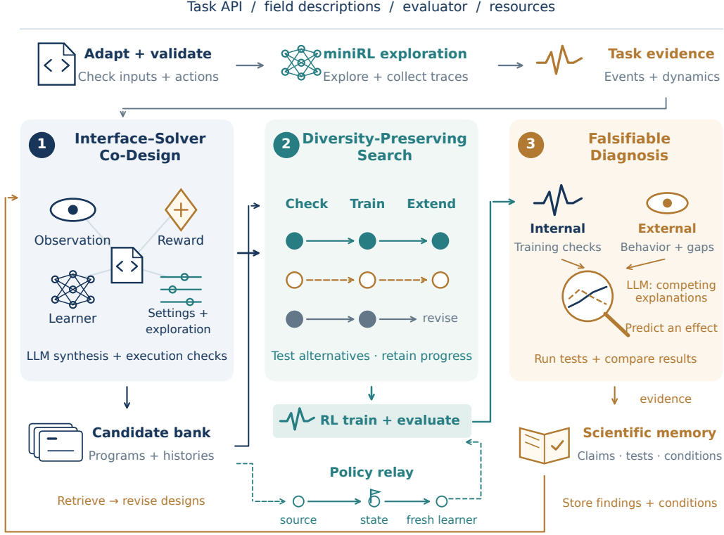
Figure 2: FARL’s architecture. An adapter exposes the task API, and miniRL collects initial experience. (1) LLMs propose observations, rewards, and solver configurations. (2) Search screens diverse candidates at short budgets and trains selected designs and controls for longer. (3) Diagnosis uses training statistics and behavior to propose the next experiment. Programs enter the candidate bank; findings and test conditions enter scientific memory. A trained policy may help a new learner reach an intermediate state during training. Final evaluation uses the new policy alone from the original resets.
