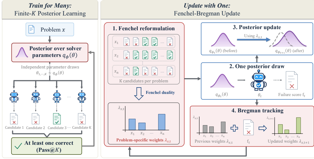
Figure 1: Overview of finite- K posterior learning and FBI. Left: K independent posterior draws generate a candidate pool, and training targets the probability that all K candidates fail. Right: Fenchel reformulation enables a one-draw IVON posterior update with a fixed problem-specific weight, while Bregman tracking reuses the observed failure to update the weight for the next visit.
