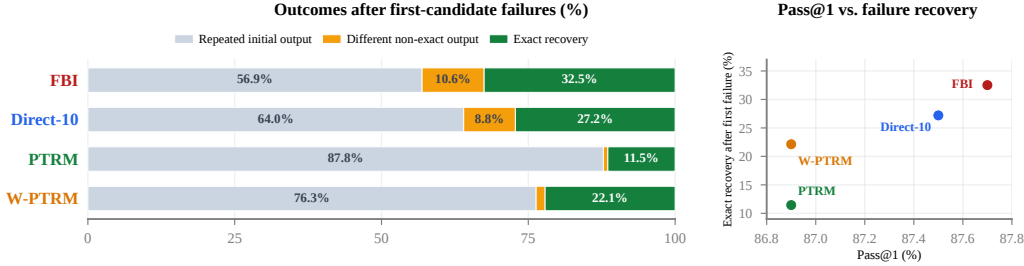
Figure 5: Recovery after first-candidate failures on Maze-Hard. Left: first-candidate failures are partitioned into three outcomes: only repeated initial outputs, different outputs with no exact solution, or at least one exact solution. Right: Pass@1 versus the exact-recovery rate among candidates 2–10 after each method’s first candidate fails. FBI has the highest conditional exact-recovery rate of 32.5%.
