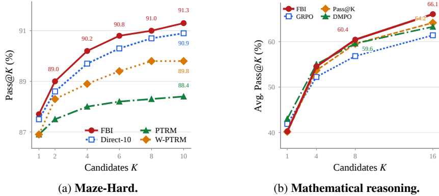
Figure 2: Candidate coverage across recursive and autoregressive models. (a) Pass@ K on 1,000 Maze-Hard test problems using TRM at depth 16. (b) Mean Pass@ K across five mathematical-reasoning benchmarks using Qwen3-4B-Base. FBI improves candidate coverage in both settings.
