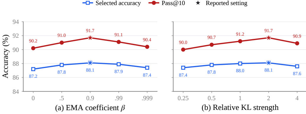
Figure 6: EMA and KL sensitivity of FBI on Maze-Hard. (a) varies the failure-EMA coefficient \beta at relative KL strength 2. (b) varies relative KL strength at \beta = 0.9 while keeping the implied prior fixed. Selected accuracy uses the frozen prefix-Q selector, and Pass@10 measures coverage among ten posterior candidates on test set with one fixed seed. Both metrics are highest at \beta = 0.9 in (a) and relative KL strength 2 in (b) among the tested settings.
