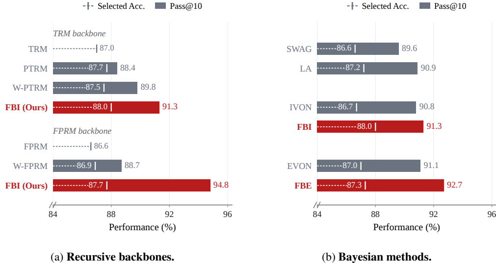
Figure 3: Performance across backbones and Bayesian methods. (a) Comparison across TRM and FPRM backbones. (b) Comparison of Bayesian methods with the TRM backbone. Bars show Pass@10, and dashed markers show selected accuracy. FB-based methods achieve higher Pass@10 than the corresponding baselines across the evaluated recursive backbones and variational optimizers.
