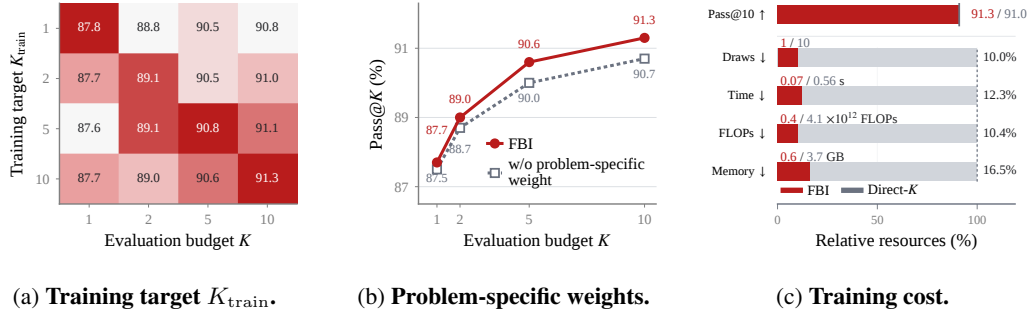
Figure 4: Finite- K posterior learning and training efficiency. (a) The diagonal pattern shows that K_{\text{train}} = K attains the highest reported Pass@ K at each budget. Cells show Pass@ K (%); darker shades indicate higher within-column coverage. (b) Problem-specific weights outperform their minibatch-mean replacement at K_{\text{train}} = 10 . (c) At K_{\text{train}} = 10 , FBI achieves comparable coverage to Direct-10 using 12.3% of its measured training time per update. Resources are relative to Direct-10 (100%); FLOPs are in units of 10^{12} .
