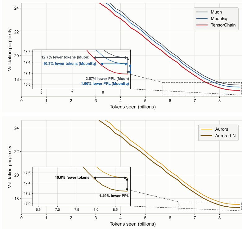
Figure 1: Top: Comparison of Muon, MuonEq and TensorChain; Bottom: Comparison of Aurora and Aurora-LN, both setups are training on Qwen3-0.6B with a 1M-token batch at 1\times Chinchilla under cosine LR. For other setups see section F.6.
