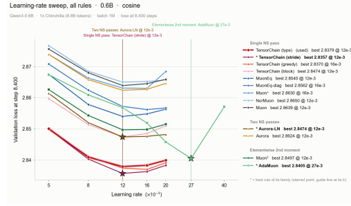
(b) COS learning rate tuning
