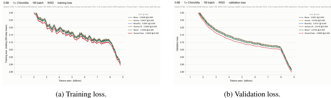
Figure 4: WSD trajectories for Qwen3-0.6B, 1M-token batch, 1 \times Chinchilla.
