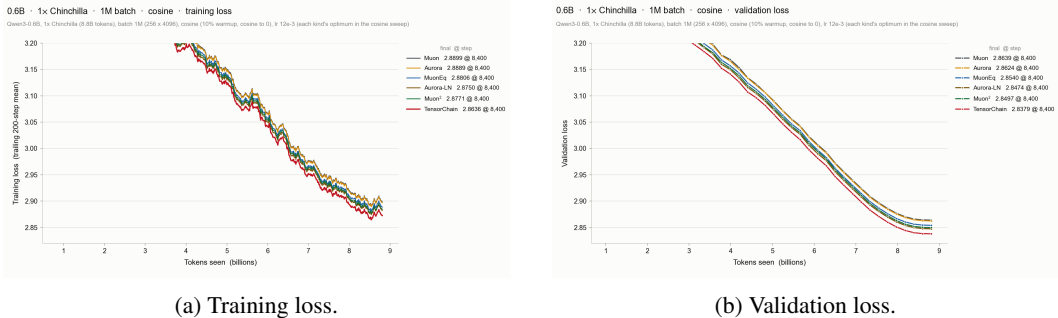
Figure 6: Cosine trajectories for Qwen3-0.6B, 1M-token batch, 1 \times Chinchilla.
