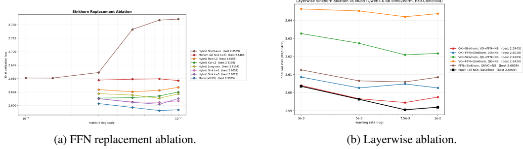
Figure 2: Replacing Newton–Schulz with cheaper axis-wise normalizations on Qwen3-0.6B after 8.8B training tokens. (a) NS5 is retained on Q, K, V, O while the FFN uses the indicated replacement. (b) A single row–column equilibration sweep is applied to the indicated parameter classes, with NS5 retained elsewhere.
