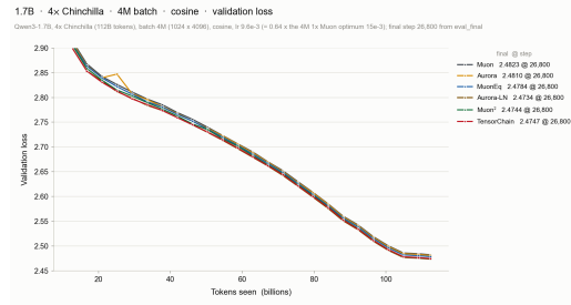
(b) Validation loss.
