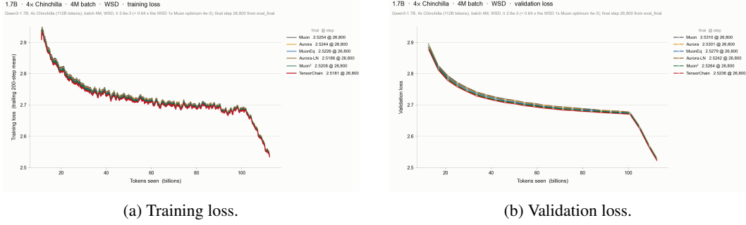
Figure 5: WSD trajectories for Qwen3-1.7B, 4M-token batch, 4 \times Chinchilla.
