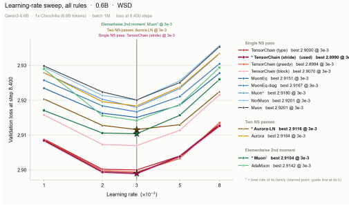
(a) WSD learning rate tuning loss.
