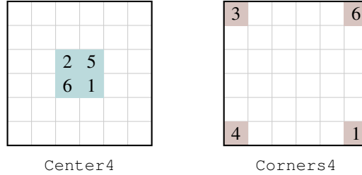
Figure 10: Left: \text{Center4} requires the four center cells (shaded) to all differ from each other - only 4 of the 6 symbols are involved, so unlike the region rules above, no symbol is required to appear. Right: \text{Corners4} imposes the same all-different requirement on the four corner cells instead.
