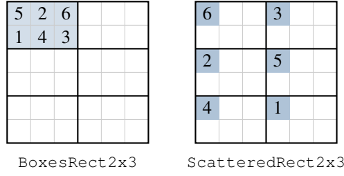
Figure 3: Left: the BoxesRect2x3 rule requires the six cells physically inside one 2 \times 3 box (shaded, one possible filling shown) to together contain every symbol exactly once. Right: its scattered counterpart ScatteredRect2x3 instead groups the six cells that share the same position across the grid's six boxes (here, each box's top-left corner, shaded) into one such group.
