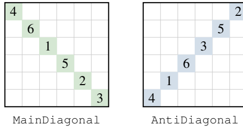
Figure 4: Left: MainDiagonal requires the six cells on the \searrow diagonal (shaded, one possible filling shown) to together contain every symbol exactly once. Right: AntiDiagonal imposes the same requirement on the six cells of the \swarrow diagonal instead.
