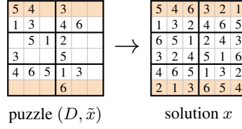
Figure 1: A completion problem (Definition 2.3): given cells D (left) determine a unique admissible configuration x (right) in some world W_N(\mathcal{A}, \mathcal{F}) . This particular puzzle comes from the concrete family introduced in Section 3.
