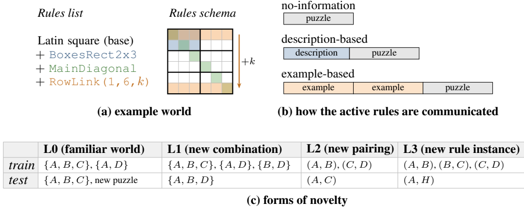
Figure 2: Overview of the setup. (a) Example world: list of rules and schematic representation of these rules. (b) How the rules are communicated: information is appended before the puzzle under diverse forms. (c) Illustration of the forms of novelty. Letters designate rules.
