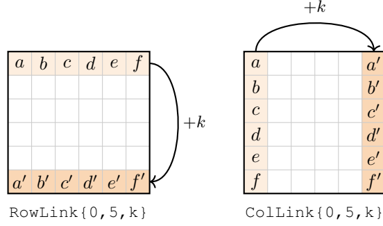
Figure 9: Left: \text{RowLink}\{0, 5, k\} links only row 1 and row 6 (shaded) - every column’s value in row 6 must equal its value in row 1 shifted by k in the alphabet ( x' denotes x+k \bmod 6 ); every other row is unconstrained by this rule. \mathcal{V} includes two more such row pairs, (2, 5) and (3, 4) (1-indexed), and the column analogues, each at any k \in \{1, \dots, 5\} as a separate instance. Right: \text{ColLink}\{0, 5, k\} is the column-wise version, linking only column 1 and column 6.
