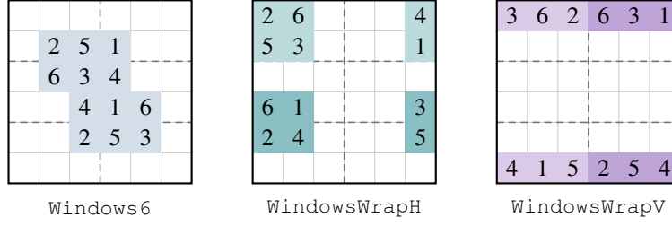
Figure 7: The three window placements (shaded, one possible filling shown), with the 2 \times 3 box tiling from Figure 3 overlaid as a dashed reference grid. Windows6’s pair straddles the box boundaries, in the spirit of a real Windoku puzzle. WindowsWrapH and WindowsWrapV instead each wrap a window pair around the grid’s border (matching shade intensity marks the two pieces of the same window, split across the wrap); neither ever coincides with a BoxesRect2x3 box.
