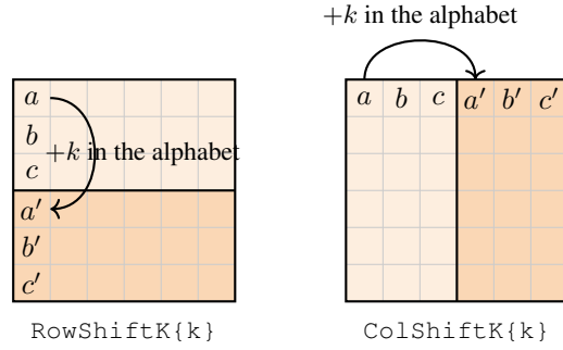
Figure 8: Both rules cut the grid into two fixed areas and then shift the alphabet value , position by position, by k between them - the areas themselves never move or depend on k ( x' denotes x shifted by k in the alphabet, mod 6). Left: RowShiftK{k} cuts the grid into a top and a bottom area (one column shown: top values a, b, c ; the corresponding bottom values must be a', b', c' ); every other column is cut and shifted the same way. Right: ColShiftK{k} is the column-wise analogue, cutting a left and a right area instead.
