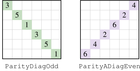
Figure 6: Left: ParityDiagOdd restricts every cell on the main diagonal (shaded) to the odd values \{1, 3, 5\} ; unlike the earlier diagonal rule, repeats are allowed here, since membership in this fixed set is all that is required. Right: ParityADiagEven applies the analogous restriction to the anti-diagonal, with the even set \{2, 4, 6\} . The remaining two combinations, ParityDiagEven and ParityADiagOdd , swap which parity set applies to which diagonal.
