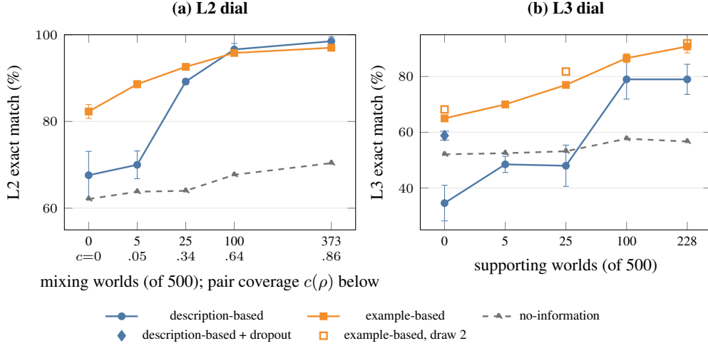
Figure 12: Exposure dials (Section 3.4). (a) L2 accuracy on draw 1 of the no-mix split as training worlds mixing the two rule groups are added; the test worlds are the same at every level and the training sets are nested. (b) L3 accuracy on the held-out column links as training worlds containing a supporting column link are added; held-out instances and test worlds are the same at every level. Points are means over 4 seeds, bars are one standard deviation. The diamond is the description-based model trained with description dropout; hollow squares are the example-based setup on a second draw of the training worlds.
