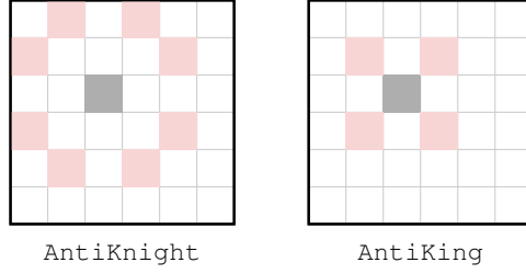
Figure 5: Left: AntiKnight forbids the highlighted cell (dark grey) from sharing a value with any cell a chess knight’s-move away (red). Right: AntiKing forbids the same cell from sharing a value with any diagonally-adjacent cell (red).
