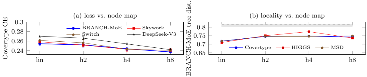
Figure 2: Node-map effect. (a) Covertypes loss of the learned routers vs. node map, \pm sd (Hash, at 0.447, is off-scale). (b) BRANCH-MoE’s tree distance vs. node map on UCI; dashed: random pairs (0.817); shaded: flat routers at their best maps.
