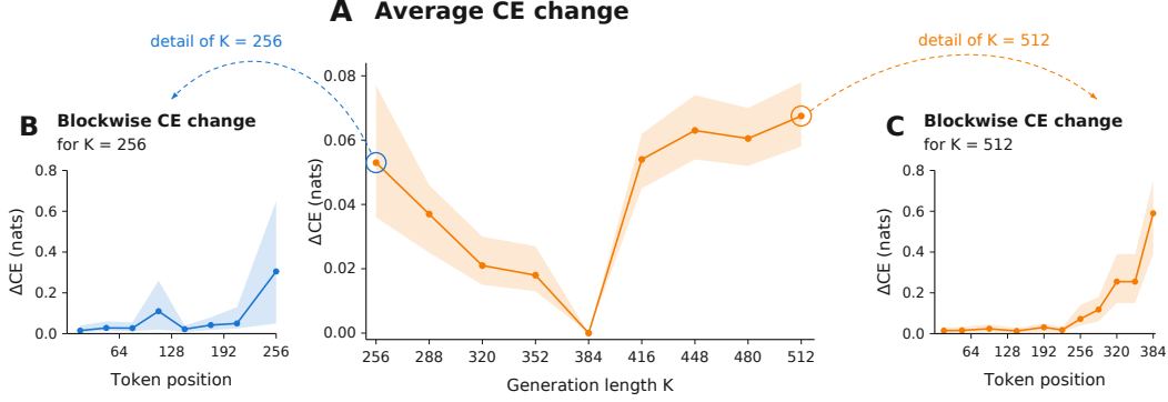
Figure 4: Canvas-extent mismatch increases reference cross-entropy. Target responses are generated at source generation length K_0 = 384 , and \Delta\text{CE} is the change of CE compared to that evaluated at K_0 . A (center): Mean \Delta\text{CE} across generation lengths, evaluated along each candidate’s own reference-conditioned trajectory. B (left) and C (right): Detailed blockwise \Delta\text{CE} across response positions for K = 256 (blue) and K = 512 (orange).
