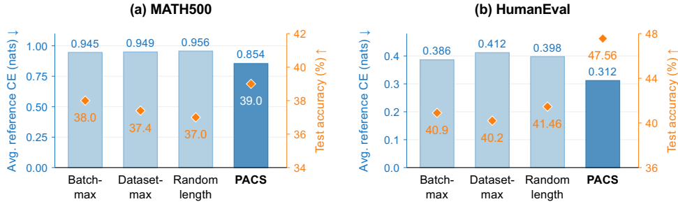
Figure 5: Canvas choice and reference predictability. Target CE (blue bars, left) and post-SFT test accuracy (orange diamonds, right) for four canvas-length rules on MATH500 and HumanEval with LLaDA-8B-Instruct at K_{\text{eval}} = 256 .
