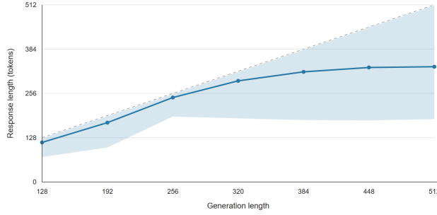
Figure 2: Longer canvases induce longer responses. Realized response length increases with allocated generation length.
