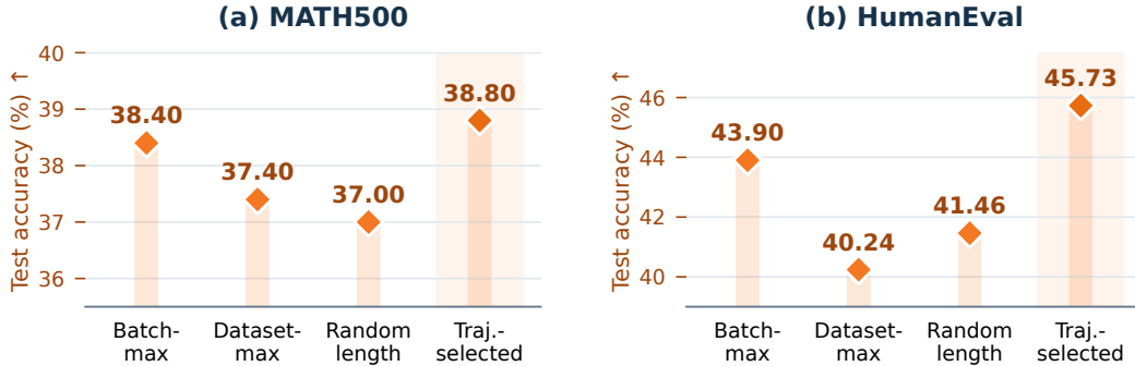
Figure B.1: Semi-AR block canvas-choice test accuracy. Post-SFT test accuracy (orange diamonds) on MATH500 and HumanEval at K_{\text{eval}} = 256 for four canvas-length rules.
