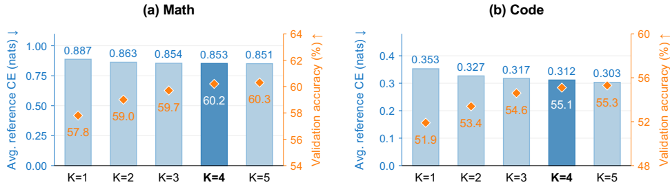
Figure 6: Canvas search extent at K_{\text{eval}} = 256 . Bars show average reference CE (left axis); orange diamonds show held-out validation accuracy (right axis).
