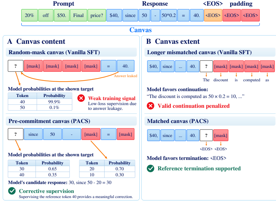
Figure 1: The training canvas changes reference supervision. Top: A canvas includes prompt tokens (green), visible answer tokens (blue), and masked positions (red). A: Visible reference content can conceal or expose a commitment-time disagreement. B: Canvas extent can alter the prediction problem, inducing an extra stopping signal on a mismatched canvas but not on the matched canvas.
