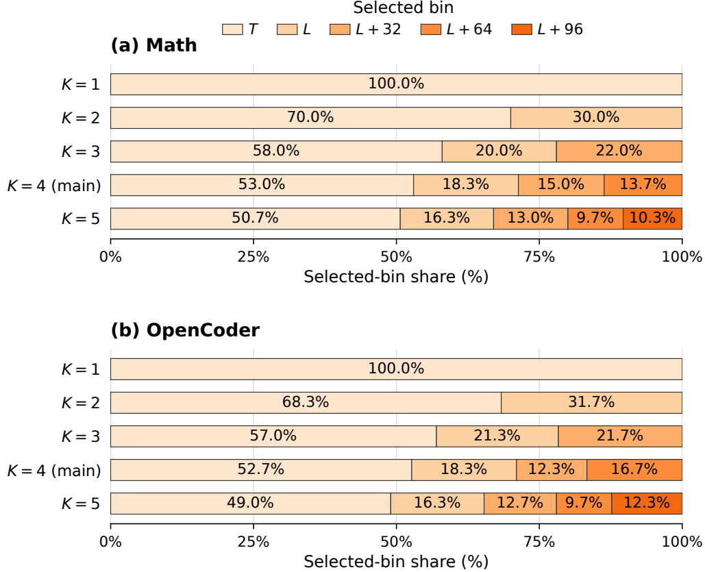
Figure A.1: Selected-bin proportions across candidate families. Each horizontal bar is normalized independently to 100% and shows the fraction of examples for which PACS selects each candidate in the nested family \Lambda_K(P, A) . We use L_{\text{ref}} = |P| + |A| , L_{\min} = B \lceil L_{\text{ref}}/B \rceil , and B = 32 , so the bins correspond to L_{\text{ref}} , L_{\min} , L_{\min} + B , L_{\min} + 2B , and L_{\min} + 3B . Segment labels give percentages rounded to one decimal place. Bins not contained in a given \Lambda_K have no segment, and colors identify the same candidate lengths across datasets and families. \Lambda_4 is the main configuration.
