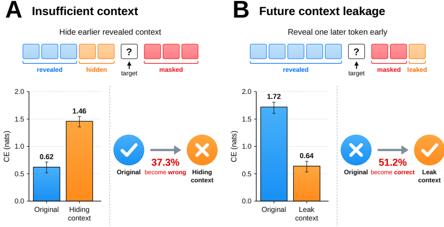
Figure 3: Changing context around commitment can create or conceal reference disagreement. LLaDA-8B-Instruct on GSM8K. A: Insufficient context. Hiding reference tokens revealed in the preceding step makes 37.3% of initially correct predictions wrong. B: Future context leakage. Revealing one reference token scheduled for the following reveal step early makes 51.2% of initially wrong predictions correct.
