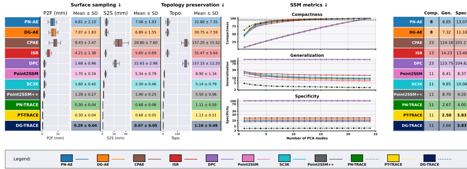
Fig. 2. Quantitative comparison of our modular architecture against prior SSMs on the held-out test set. We report point-to-face distance (P2F), surface-to-surface distance (S2S), and topology preservation metric (Topo), as well as the statistical shape model metrics, compactness (Comp.), generalization (Gen.), and specificity (Spec.). Lower is better for all metrics. Bold characters denote the best quantitative result for a metric.
