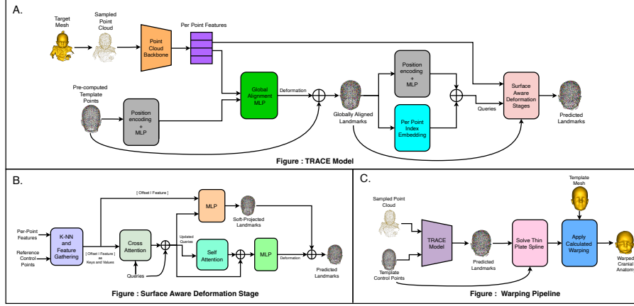
Fig. 1. Overview of the Template-constrained Robust Artifact-aware Correspondence Estimation (TRACE) framework. (A) A point-cloud backbone encodes the input scan, global-alignment stage predicts initial template-control-point displacements, and two Surface-Aware Deformation (SAD) stages refine landmarks onto the observed head surface. (B) A SAD stage takes the current reference landmarks and query embeddings. For each landmark, it gathers the k_s nearest target points and backbone features, uses cross-attention to form a neighborhood-aware query, softly projects the landmark as a weighted average of nearby target points, and applies self-attention plus an MLP to predict a residual update. (C) TPS warping deforms the dense template mesh using the transformation defined from template control points toward predicted landmarks, reconstructing head anatomy while suppressing artifacts.
