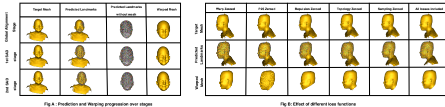
Fig. 5. Qualitative ablation analysis: (A) Prediction and warping progression across the deformation cascade. (B) Effect of removing individual loss terms to show the importance of each loss term.
