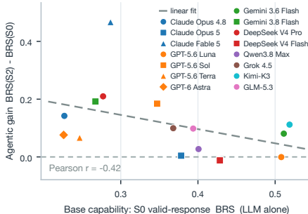
Figure 4: Agentic gain negatively correlates with base capability. Models with lower S0 BRS tend to gain more, reflecting convergence toward a tool-limited risk ceiling.
