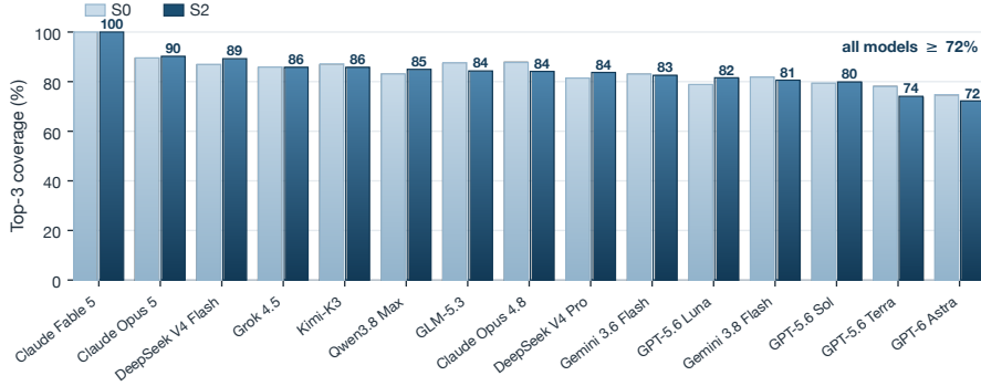
Figure 5: Almost every design lands on a measurement. Top-3 coverage against the hidden ground truth, per model, in S0 and S2, on a full 0–100% scale; models are ordered by their S2 coverage. A unit enters the average when the model submitted a complete, legal top-3, so a low value here means three legal designs that the assay did not measure, not a failed answer.
