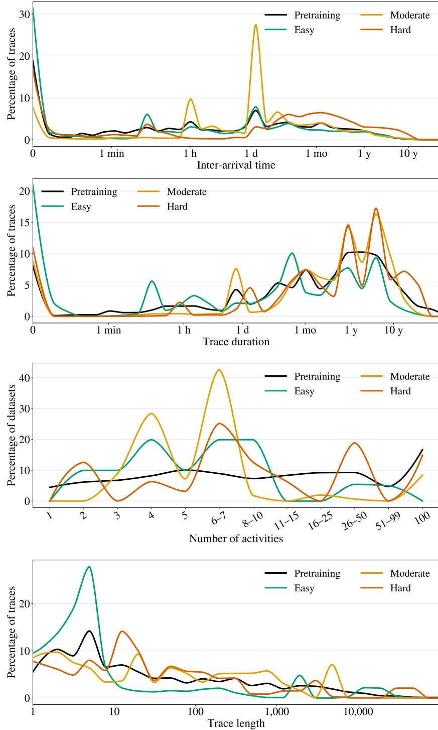
Figure 5: Interarrival times, trace durations, activity counts, and trace lengths per difficulty in the test datasets, and among the pretraining datasets. Interarrival times, trace durations, and trace lengths are per-dataset averages.
