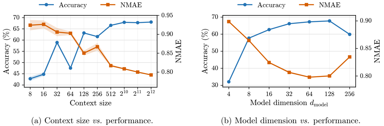
Figure 3: Ablation results for context size and model dimension.
