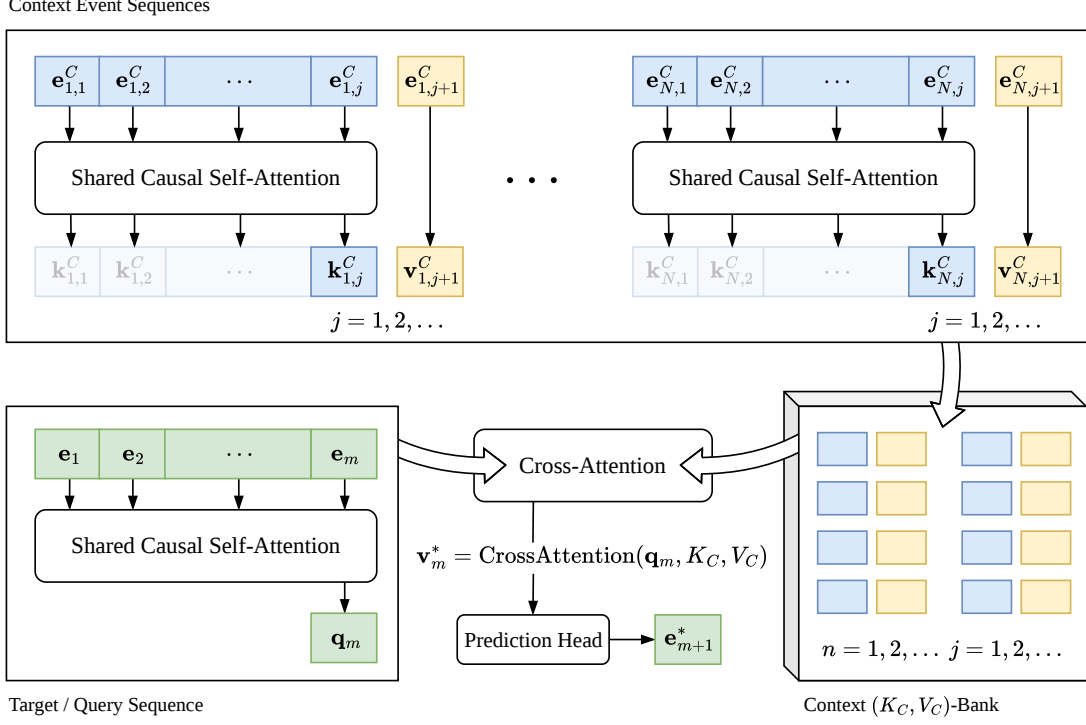
Figure 1: The architecture of Foundation Event Predictor (FEP). Context histories and observed next events form keys and values, respectively, while target histories form queries for cross-attention-based nonparametric prediction.
