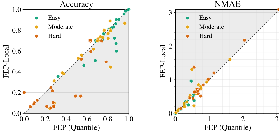
Figure 4: Dataset-wise comparison of FEP (Quantile) and FEP-Local on the 50 held-out datasets. Colors denote dataset difficulty, and the dashed line indicates equal performance. Points below the diagonal favor FEP for accuracy, whereas points above the diagonal favor FEP for NMAE. The FEP-favoring region is shaded in both panels.
