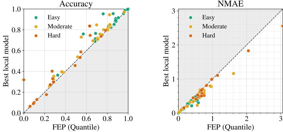
Figure 2: Dataset-wise comparison between FEP and the best locally trained model. Colors indicate empirical dataset difficulty, and the dashed line denotes equal performance. The shaded region indicates the side of the diagonal where FEP performs better.
