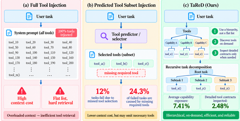
Figure 1: Motivation for tool-aware recursive decomposition. (a) Injecting descriptions and contracts of the full library consumes substantial context and distracts selection of task-relevant tools. (b) A fixed predicted subset can omit necessary tools and offers little structural guidance for dividing a task into capability-aligned subtasks. (c) TaReD navigates a capability hierarchy to retrieve relevant information on demand, guide recursive decomposition toward executable stages, and inspect detailed contracts only when needed.
