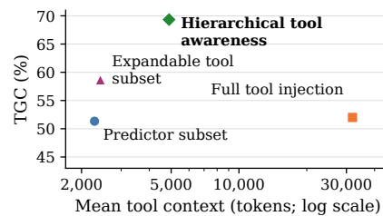
Figure 3: Mean tool-context tokens per saved decision (log scale) versus TGC for the four settings in Table 2.
