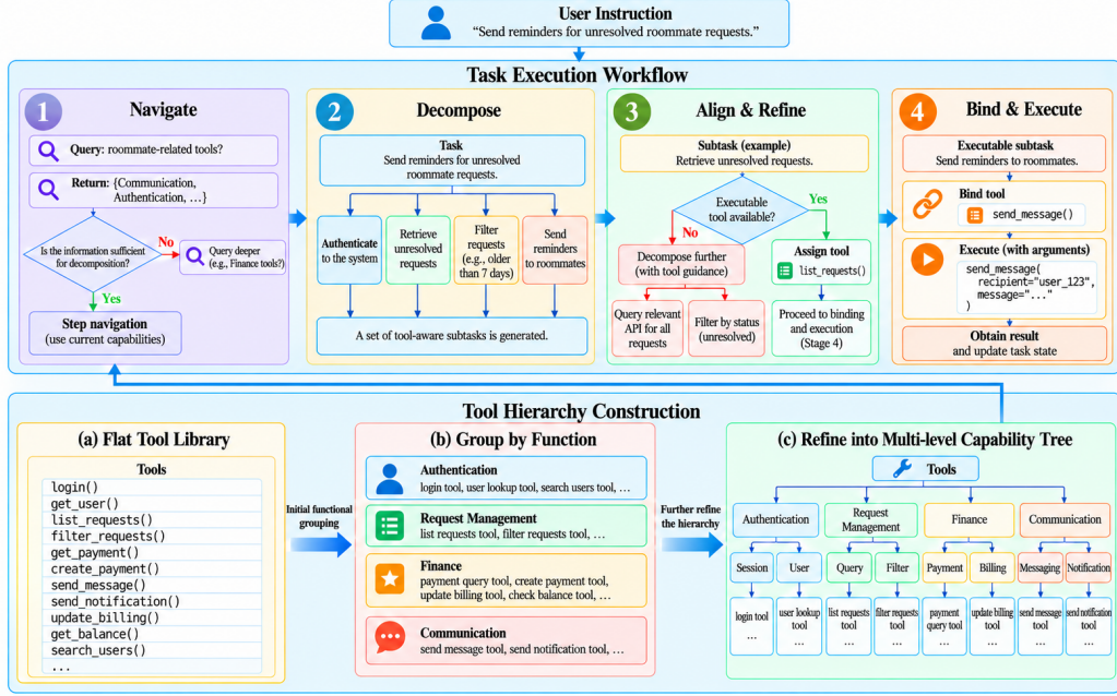
Figure 2: Overview of TaReD. Bottom: a flat tool library is grouped by function and refined into a multi-level capability tree. Top: the agent navigates this hierarchy, decomposes and refines subtasks using capability information, then binds arguments and executes tools when a stage is ready to execute. Returned results update the task state for subsequent stages.
