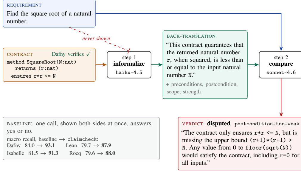
Figure 1: One claimcheck run, on a Dafny contract from CloverBench whose postcondition was weakened (class C2). Like the sorting example, the contract still verifies and is satisfied by returning zero. Step 1 translates the contract into English without ever seeing the requirement, so the informalization can only report what the contract says. Step 2 compares the informalization with the requirement and names the discrepancy; it never sees the contract. Colours follow the data: blue is the natural-language requirement, amber the formal artifact, green its informalization. A single-call baseline shown both sides at once scores lower on all four languages (Table 2).
