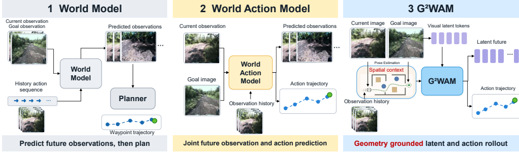
Figure 1: Navigation world model paradigms. Conventional world models plan over predicted observations, whereas world action models jointly predict observations and actions. G^2WAM further leverages estimated spatial context to efficiently roll out future latents and executable actions.
