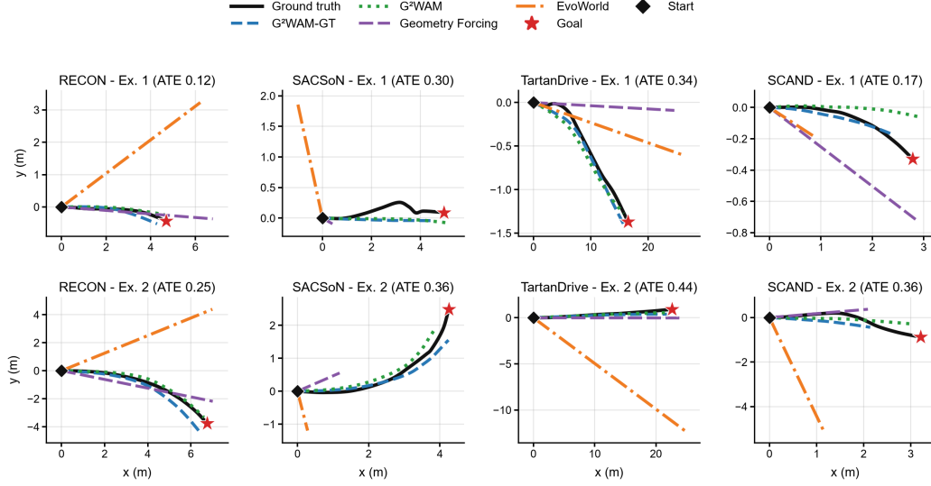
Figure 3: 8-step trajectory rollouts on RECON, SACSoN, TartanDrive, and SCAND, with all paths aligned at the rollout origin.
