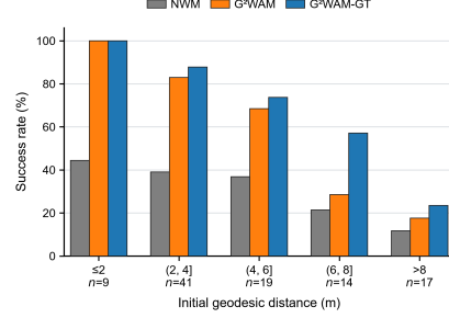
Figure 4: Closed-loop success rate grouped by initial geodesic distance. n denotes the number of episodes in each distance range.
