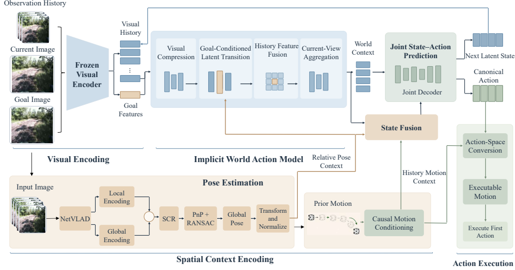
Figure 2: Overview of G 2 WAM. A learned localizer anchors the goal and observed frames in a shared scene frame to obtain the goal-relative pose and causal history motions. The goal image and pose guide joint latent and waypoint prediction, while the history motions condition the action branch.
