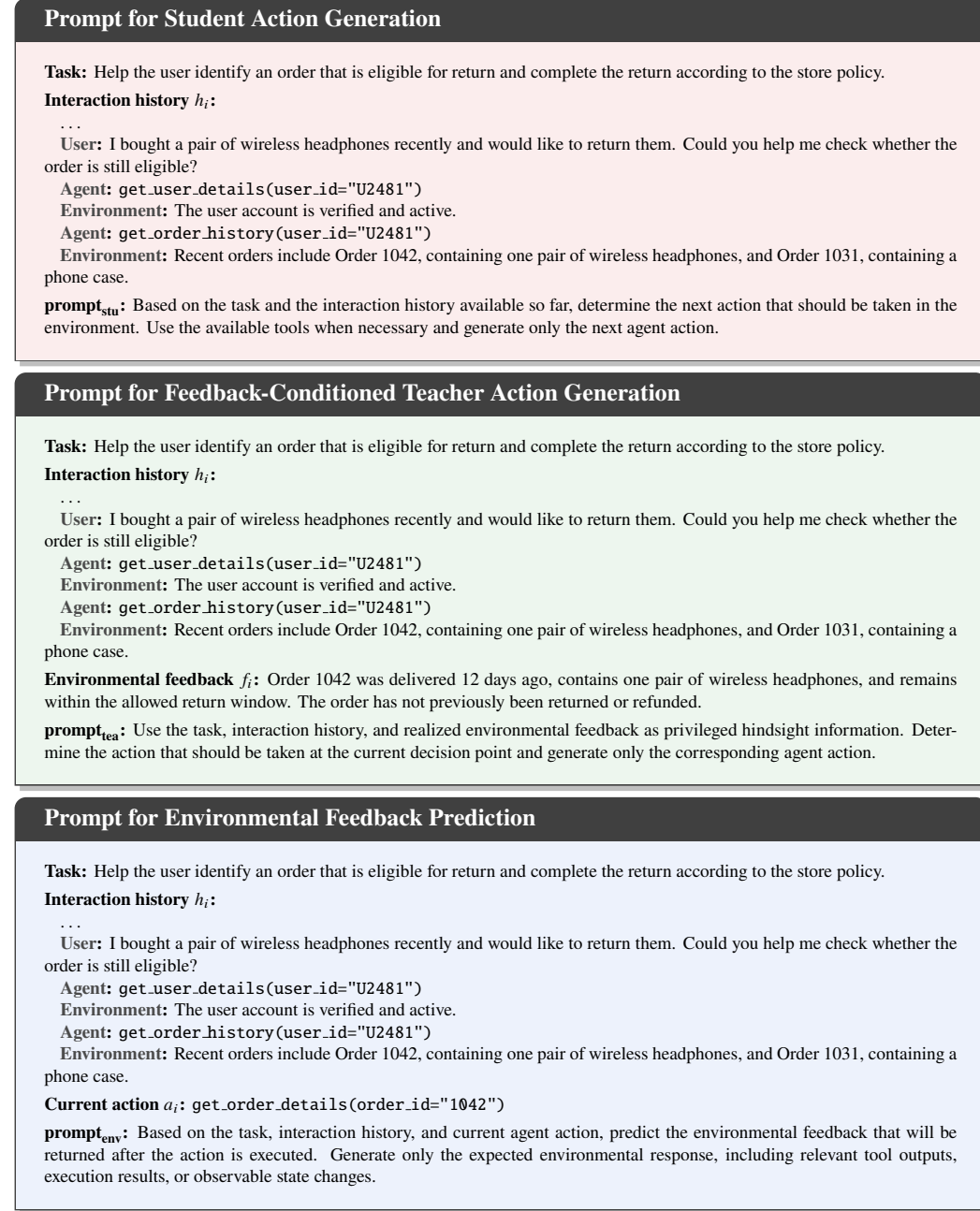
Figure 4: Illustrative prompting interfaces used in SELF. The student prompt \text{prompt}_{\text{stu}} generates the next action a_i from the interaction history h_i ; the teacher prompt \text{prompt}_{\text{tea}} additionally conditions on the realized environmental feedback f_i as privileged hindsight information; and the environmental-feedback modeling prompt \text{prompt}_{\text{env}} predicts f_i from h_i and the current action a_i .
