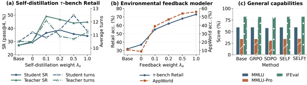
Figure 3: Ablation studies and general capability evaluation with Qwen3-4B-Instruct. (a) Student and privileged teacher success rates (SR, pass@4) and average interaction turns on \tau -bench Retail across different values of \lambda_o . (b) Environmental feedback prediction accuracy on \tau -bench Retail and AppWorld across different values of \lambda_a . (c) Performance on MMLU, MMLU-Pro, and IFEval; SELF† denotes the privileged teacher. Vertical dashed lines in (a) and (b) indicate default settings.
