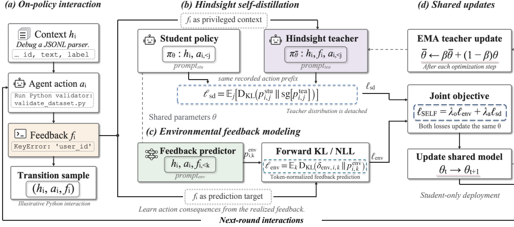
Figure 1: Overview of SELF. The current policy interacts with the environment to collect transitions (h_i, a_i, f_i) . Each transition is used for two complementary objectives: hindsight self-distillation, where a feedback-conditioned EMA teacher supervises the student policy, and environmental feedback modeling, where the model predicts the realized feedback from the interaction history and action. The two objectives are jointly optimized to obtain the next-round policy.
