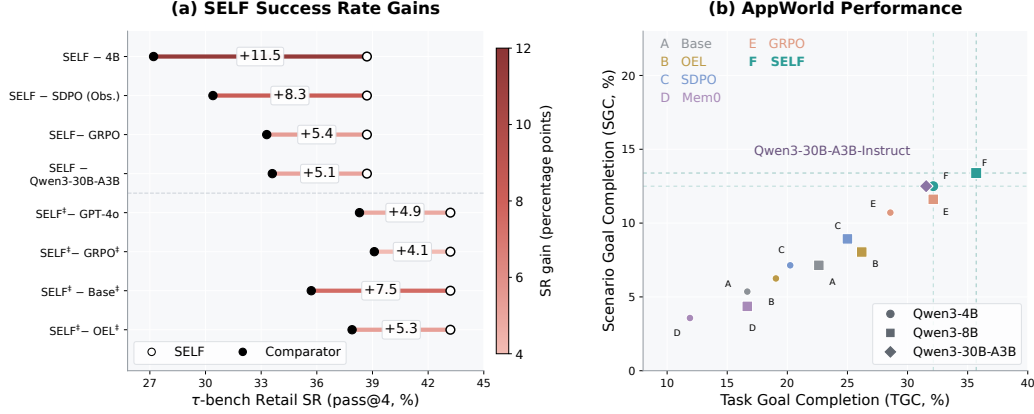
Figure 2: Performance comparison on \tau -bench Retail and AppWorld. (a) Success rate (SR, pass@4) gains of SELF over selected comparators on \tau -bench Retail. Open and filled circles denote SELF and comparator scores, respectively; annotations and line colors indicate gains in percentage points. The superscript \ddagger denotes Qwen3-8B; unmarked methods use Qwen3-4B-Instruct unless otherwise specified. (b) Task goal completion (TGC) and scenario goal completion (SGC) on AppWorld. Colors distinguish methods, and marker shapes distinguish model backbones.
