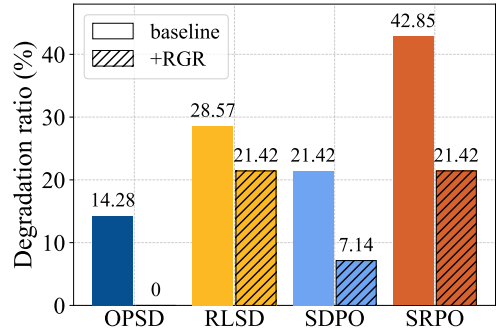
Figure 3: Comparison of the capability degradation ratio between the baseline and the baseline+RGR model on AIME24 (%).
