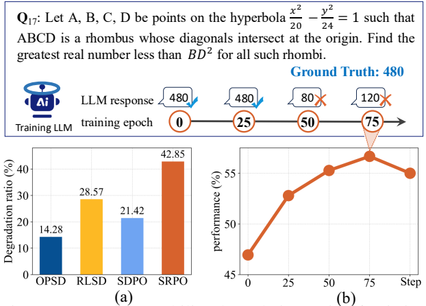
Figure 1: (a) The capability degradation ratio of existing methods; (b) Although the overall performance improves during training, some problems that were previously responded correctly become incorrectly answered as optimization progresses.
