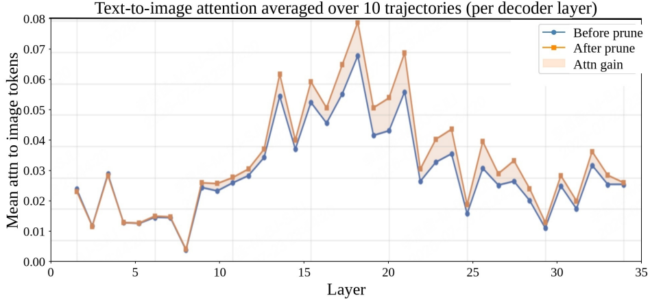
Figure 2: Text-to-image attention across decoder layers, averaged over 10 tool-use trajectories. Blue and orange denote attention before and after pruning, respectively, and the shaded region shows the gain. Pruning summary-covered reasoning consistently increases attention to image tokens, indicating stronger reliance on visual evidence.
