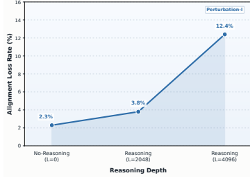
(a) Qwen3-8B (LogicAsker)
