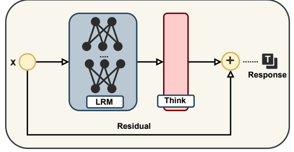
Figure 5: The framework of RRA. After the LRM generates the reasoning process Y based on input X , RRA re-injects the X as a residual connection to construct the context [X; Y; X] .
