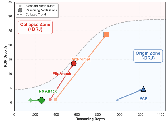
Figure 3: The alignment collapse trend under RT. Small markers denote baseline RSR ( y -axis) drops without RT, while large markers indicate the amplified degradation when RT is integrated with attacks. The plot reveals that as reasoning depth ( x -axis) increases, models enter an alignment collapse zone.
