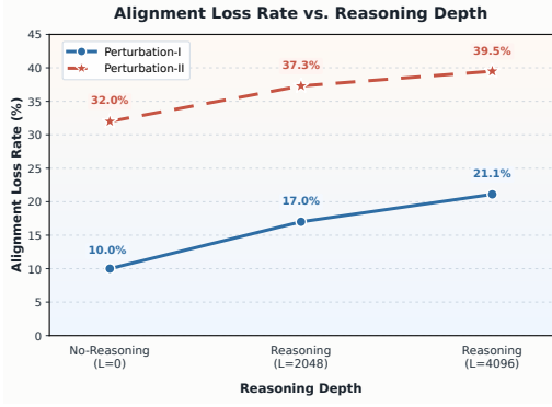
(a) Qwen3-8B (AIME2024)
