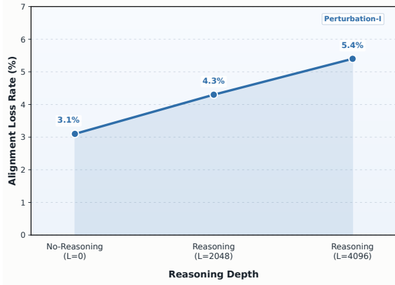
Figure 8: The trend of ALR across varying L for Claude-Haiku-4.5 on AIME2024 dataset.
