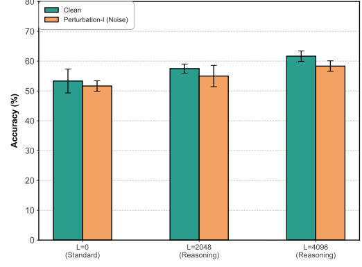
(b) Claude-Haiku-4.5
