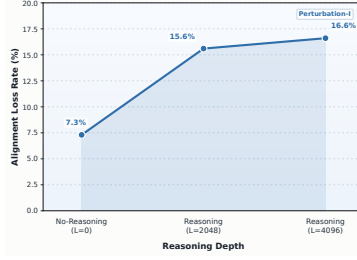
(b) Qwen3-14B (LogicAsker)
