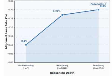
(c) GLM4.6 (LogicAsker)
