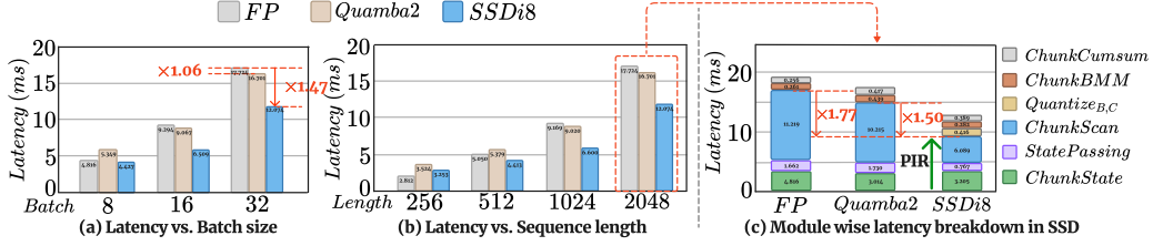
Figure 4: SSD latency of quantization methods on Mamba-2 2.7B: (a) varying batch ( L = 2048 ), (b) varying length ( B = 32 ), and (c) module-wise latency ( B = 32 , L = 2048 ). PIR denotes Persistent INT8 Representation. SSDi8 achieves up to 1.47\times overall speedup and 1.77\times in the State path.
