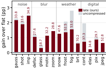
Figure 5: Per-corruption gain over flat at iso-GFLOPs (DeiT-S, r_{\text{base}}=8 , \gamma=2 , ImageNet-C sev=5); uncompressed in gray. All 15 corruptions improve; labels are late’s top-1.
