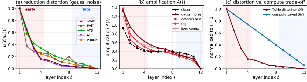
Figure 3: Per-layer reduction distortion and amplification (DeiT-S, ImageNet-C severity 5; means over N=1024 images, standard error < 2\% ). (a) The directly-measured distortion D(\ell) of reducing at layer \ell only (relative output-logit change, gaussian noise), normalized to layer 1, for all five reducers. (b) The amplification A(\ell) (clean and one corruption per ImageNet-C group). (c) D(\ell) against the compute a removal at layer \ell saves, S(\ell) , both normalized; D falls far faster than S .
