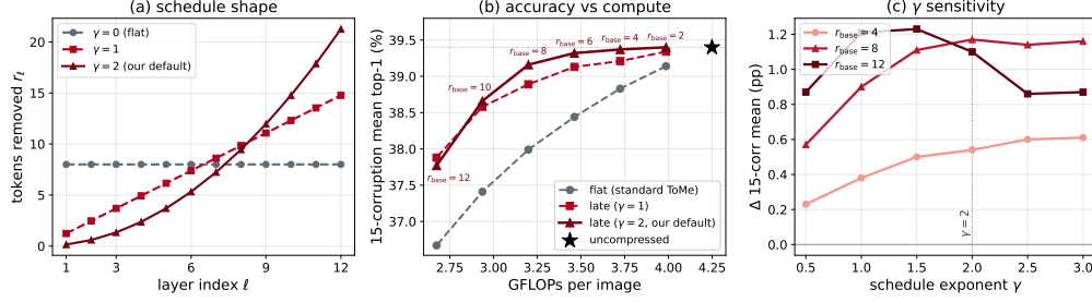
Figure 2: The late-concentrated schedule and its effect (DeiT-S, ImageNet-C severity 5). (a) schedule shape: tokens removed per layer r_\ell \propto (\ell/L)^\gamma vs. layer index (at r_{\text{base}}=8 ), for \gamma=0 (flat), 1, and our default 2; larger \gamma defers removal to later layers. (b) 15-corruption-mean top-1 vs. compute (GFLOPs), each curve a schedule swept over compression (points labeled by r_{\text{base}} ); \star marks the uncompressed model. (c) gain over flat vs. \gamma , one curve per compression level r_{\text{base}} \in \{4, 8, 12\} .
