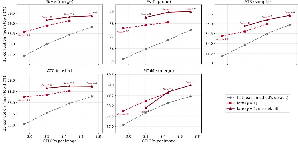
Figure 7: 15-corruption-mean top-1 vs. compute for each of the five training-free reducers (DeiT-S, ImageNet-C severity 5), each curve a schedule swept over compression (points labeled by r_{\text{base}} ). Flat and late \gamma=2 at r_{\text{base}} \in \{4, 6, 8\} are the cells of Table 3, late \gamma=1 at r_{\text{base}} \in \{6, 8, 10\} those of Table 17; each late point is drawn at the GFLOPs of the flat schedule it is calibrated to (its own cost is at or below that).
