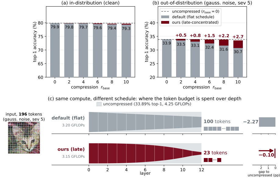
Figure 1: Token reduction increasingly sacrifices out-of-distribution accuracy; a late-concentrated schedule recovers it at no extra compute . (a, b) DeiT-S top-1 vs. the per-layer token removal rate r_{\text{base}} on clean and gaussian-noise ImageNet-C. (c) each ribbon’s height is the tokens remaining, so the pale band above is what was removed; flat removes the same number at every layer, ours follows the late-concentrated power law. Ours ends with far fewer tokens, yet closer to uncompressed.
