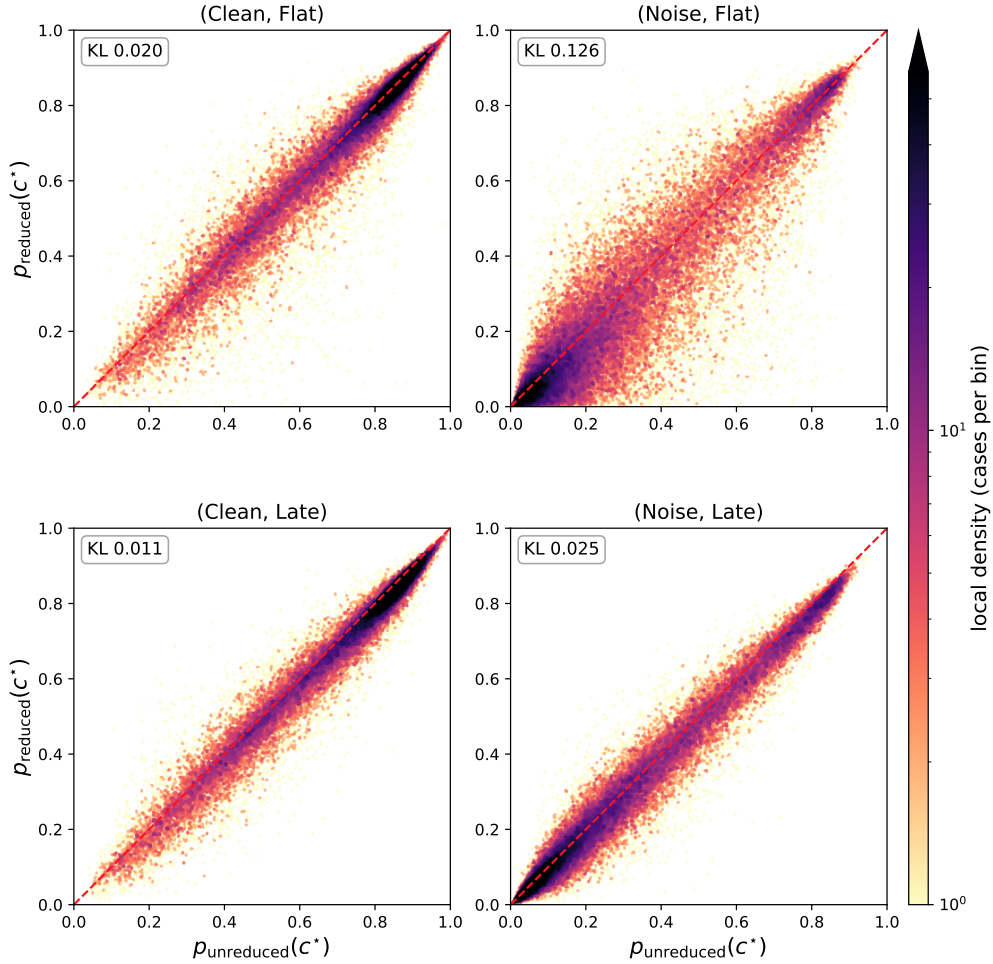
Figure 9: Per-image agreement with the unreduced model (DeiT-S, r_{\text{base}}=8 , iso-GFLOPs, 50,000 images per panel). Horizontal axis: the probability the unreduced model assigns to its own predicted class c^* ; vertical axis: the probability the reduced model assigns to that same class; exact agreement lies on the dashed line. Color is the local density of cases, on a shared scale across panels, saturating above its 75th percentile. Reduction is nearly harmless on clean input under either schedule and remains so for ours under corruption; the flat schedule departs from the unreduced model only where reduction and corruption meet. KL is the mean per-case \text{KL}(p_{\text{unreduced}} \parallel p_{\text{reduced}}) over the full class distribution on the same input. Gaussian noise at severity 5 is shown for legibility; the aggregate over all 15 corruptions is quoted above.
