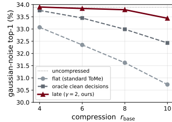
Figure 4: Oracle clean merge decisions recover less than the late schedule at every r_{\text{base}} , the gap widening with compression.
