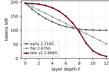
Figure 8: Tokens remaining after each layer at r_{\text{base}}=12 (DeiT-S), for the early-concentrated, flat and late-concentrated schedules; the legend gives each schedule’s GFLOPs.
