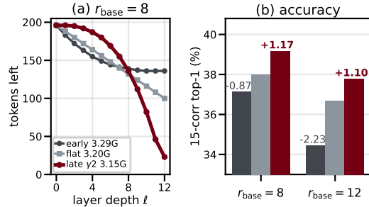
Figure 6: Schedule placement (DeiT-S, ImageNet-C sev=5). (a) tokens left per layer at r_{\text{base}}=8 , with each schedule’s GFLOPs; the r_{\text{base}}=12 profiles are in Appendix Q. (b) top-1 at both rates, \Delta vs. flat.
