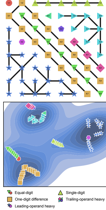
Figure 1: (top) Each node represents a distinct subtask. An undirected path exists between two nodes if and only if they are \alpha -equivalence for \alpha = 0.6 . (bot) t -SNE embeddings of the soft circuits for each subtask with perplexity=3. The node shape and color combinations are consistent with the circuit clusters in (top).
