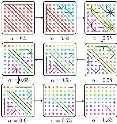
Figure 3: The emergent families of \alpha -equivalent subtasks as \alpha varies between [0, 1] .
