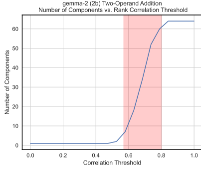
Figure 2: The number of \alpha -circuit equivalence families as \alpha varies between [0, 1] . We omit visualization of \alpha < 0 since the number of circuit families is a monotonic function of \alpha . The red region shows that 80% of circuit families emerge between \alpha = 0.58 and \alpha = 0.79
