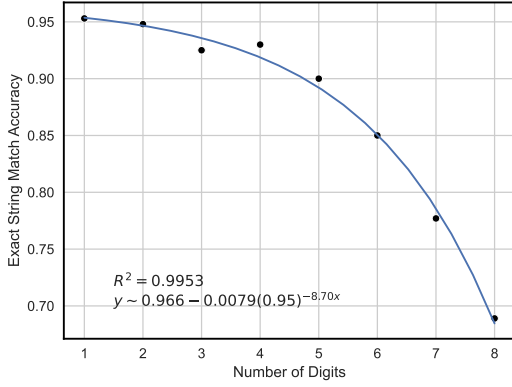
Figure 10: Exponential regression on exact string accuracy for one-digit subtasks. That is o_2 = 1 . The x -axis of the regression is simply the number of digits in o_1 as o_2 is constant.
