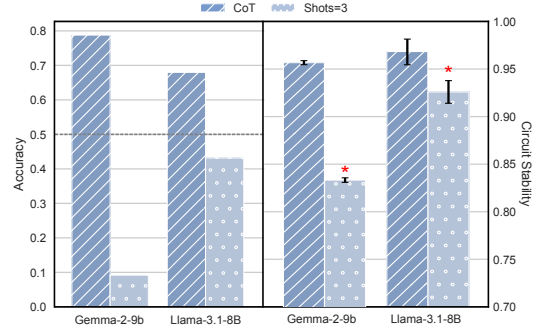
Figure 8: (left) Exact string match accuracy of sports understanding task under chain-of-thought versus few-shot prompting. (right) Circuit stability across random partitions. We perform a two-sample t -test, “*” denotes a significant difference ( p < 0.05 ).
