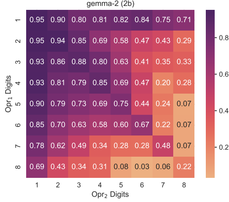
Figure 4: Performance of gemma-2-2b over arithmetic subtasks as \text{Opr}_1 := o_1 and \text{Opr}_2 := o_2 increase. Each cell denotes the exact string match accuracy.
