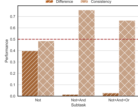
Figure 7: (left columns) The performance difference after adding parentheses. (right columns) The self-consistency of \phi-1.5 as a result of adding parentheses. The dotted line denotes random chance of 0.5 for the consistency estimates.
