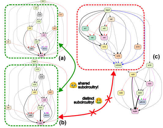
Figure 5: Circuits for (a) (8, 8) (b) (7, 7) and (c) (2, 7). (a) and (b) share many subcircuit components and are \alpha -equivalent for \alpha = 0.6 . On the other hand, (c) is not \alpha -circuit equivalent with either (a) or (b).
