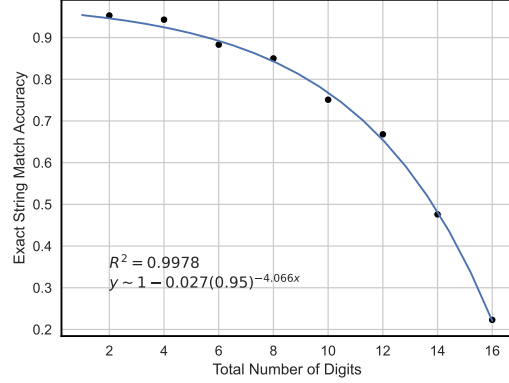
Figure 9: Exponential regression on exact string accuracy for equal-digit subtasks. That is, o_1 = o_2 . The x -axis of the regression is the sum of the number of digits in both operands.
