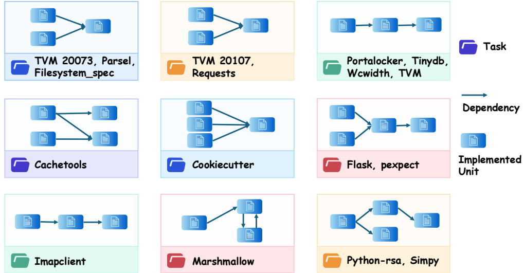
Figure 7: Task-level dependency graphs in AsyncCodeBench. Across the benchmark, we identify nine types of dependency relations, each defined by explicit upstream and downstream implementation units. These dependencies form the basis for dependency-level evaluation with ADPR.
