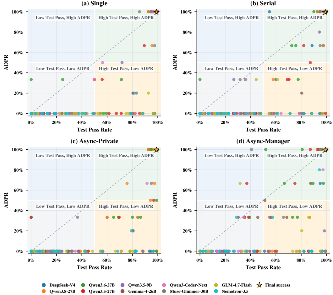
Figure 10: Test Pass Rate versus ADPR under the four protocols not shown in Figure 2(b). Each point represents a model–task outcome and colors denote models. The dashed line indicates equality between Test Pass Rate and ADPR, while the 50% boundaries provide a common visual partition. All panels use identical axes and encodings.
