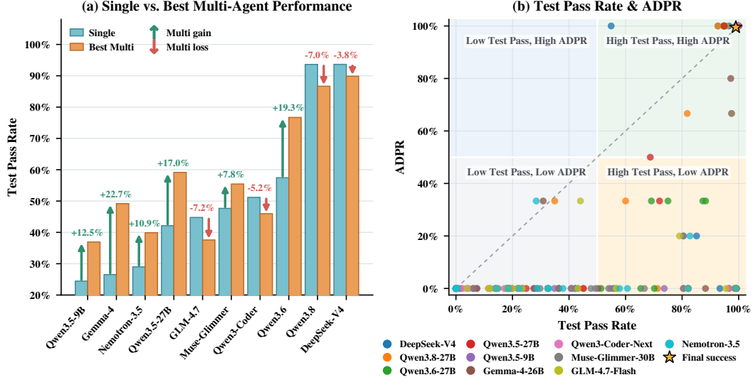
Figure 2: Collaboration gains and hidden dependency failures. (a) For each model, SINGLE is compared with the highest task-macro Test Pass Rate achieved by any of the four multi-agent protocols; arrows show the signed gain. (b) Test Pass Rate versus ADPR for 190 ASYNC-MANAGER-RO model-task outcomes. The dashed line indicates equality between the two metrics, and the 50% boundaries provide a visual partition.
