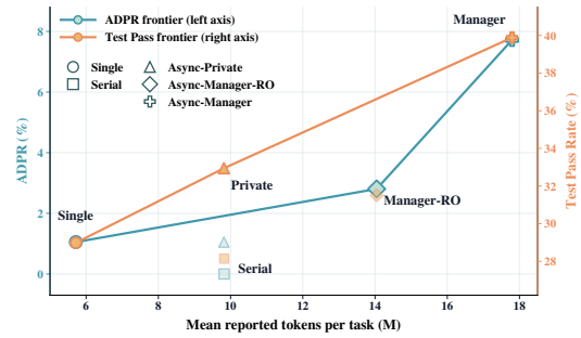
Figure 6: Quality–cost Pareto frontiers for Nemotron-3.5 under ADPR and Test Pass Rate. Both use identical protocols and token costs, yet identify different non-dominated configurations. Marker shapes indicate execution protocols, and lines connect their respective Pareto frontiers.
