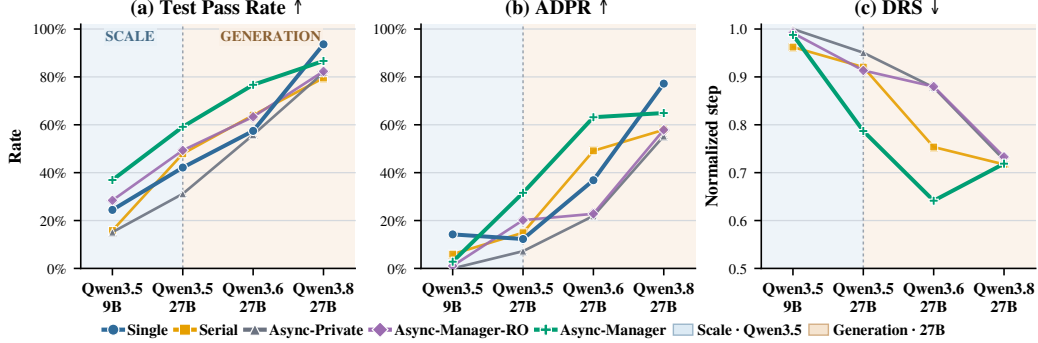
Figure 3: Qwen scale and generation analysis under five matched execution protocols. The left region compares Qwen3.5-9B and Qwen3.5-27B, while the right region compares Qwen3.5, Qwen3.6, and Qwen3.8 at a nominal scale of 27B. Panels report Test Pass Rate, ADPR, and normalized DRS; lower DRS indicates earlier dependency resolution.
