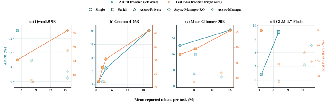
Figure 13: Metric-dependent quality–cost trade-offs for four additional models. Each panel shows the within-model Pareto frontiers under ADPR (blue, left axis) and Test Pass Rate (orange, right axis). Marker shapes distinguish execution protocols, and lines connect non-dominated configurations under each metric. Dominated configurations remain visible. Axis ranges are independently scaled across models.
