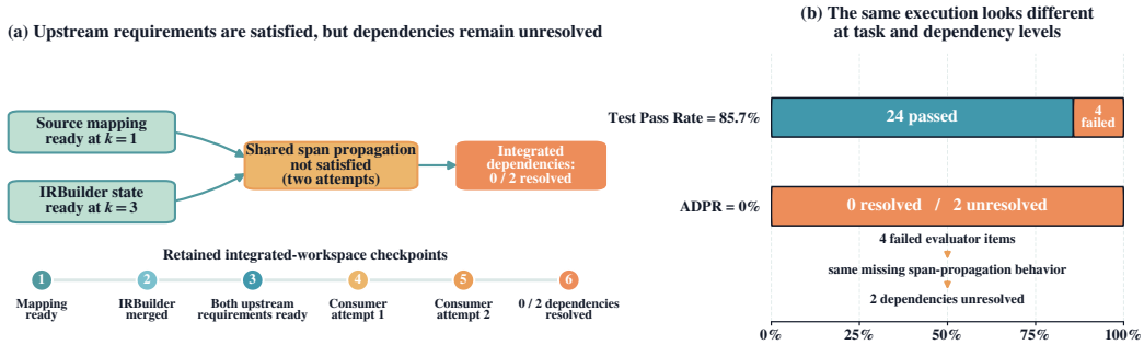
Figure 14: Case study of DeepSeek-V4 under ASYNC-MANAGER on TVM-20073. Although both upstream requirements become available during execution, the shared downstream span-propagation logic remains unsatisfied after two attempts, leaving both dependencies unresolved. The final workspace nevertheless passes 24 of 28 evaluator items (85.7% Test Pass Rate), while ADPR remains 0%, illustrating how task-level performance can obscure unresolved cross-agent dependencies and the coordination failures behind them.
