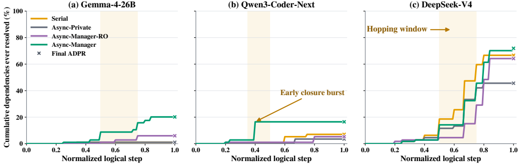
Figure 5: Representative dependency-closure trajectories across execution protocols. Each panel shows the cumulative fraction of dependencies ever resolved over normalized logical steps for one model. The shaded region marks the hopping window.
