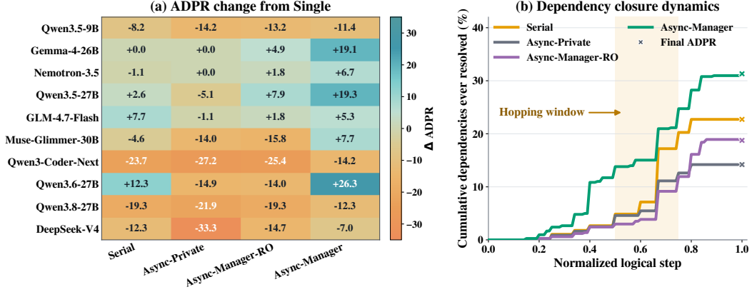
Figure 4: Protocol effects and dependency-closure dynamics. (a) ADPR change relative to Single across models and multi-agent protocols. (b) Cumulative dependency closure over normalized logical steps k/T , showing a recurrent middle-to-late hopping window ( 0.50 < k/T \leq 0.75 ).
