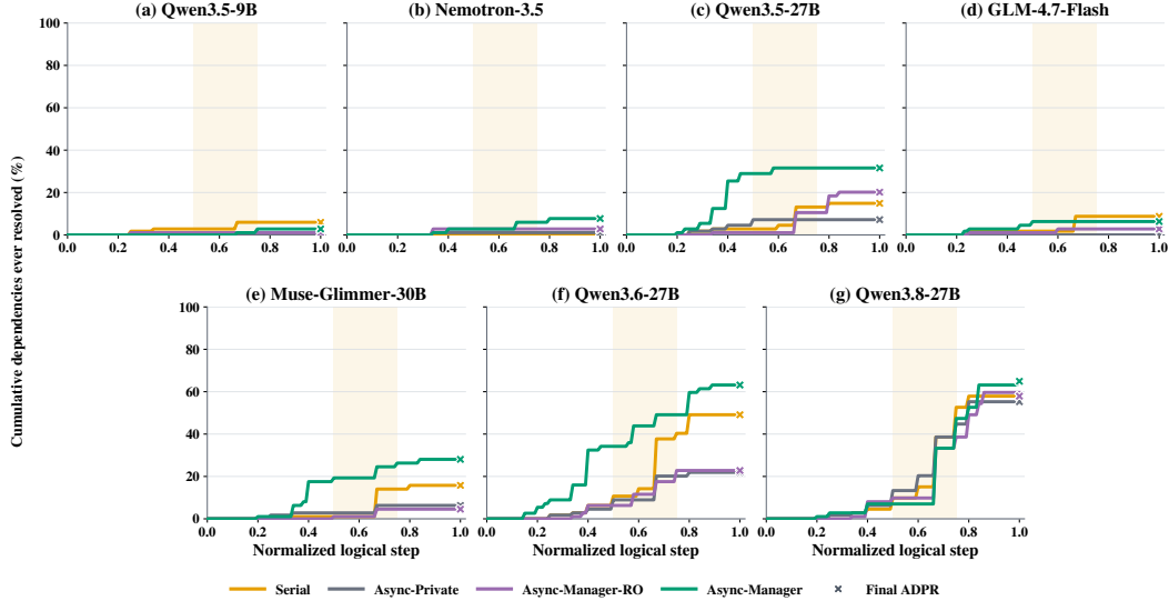
Figure 12: Dependency-closure trajectories for the seven models not shown in the main-text case studies. Curves report cumulative dependencies ever resolved over normalized logical execution, and crosses denote final ADPR. The shaded region marks the representative aggregate concentration 0.50 < x \leq 0.75 . Individual trajectories show that the onset and magnitude of concentrated closure vary substantially across models and protocols.
