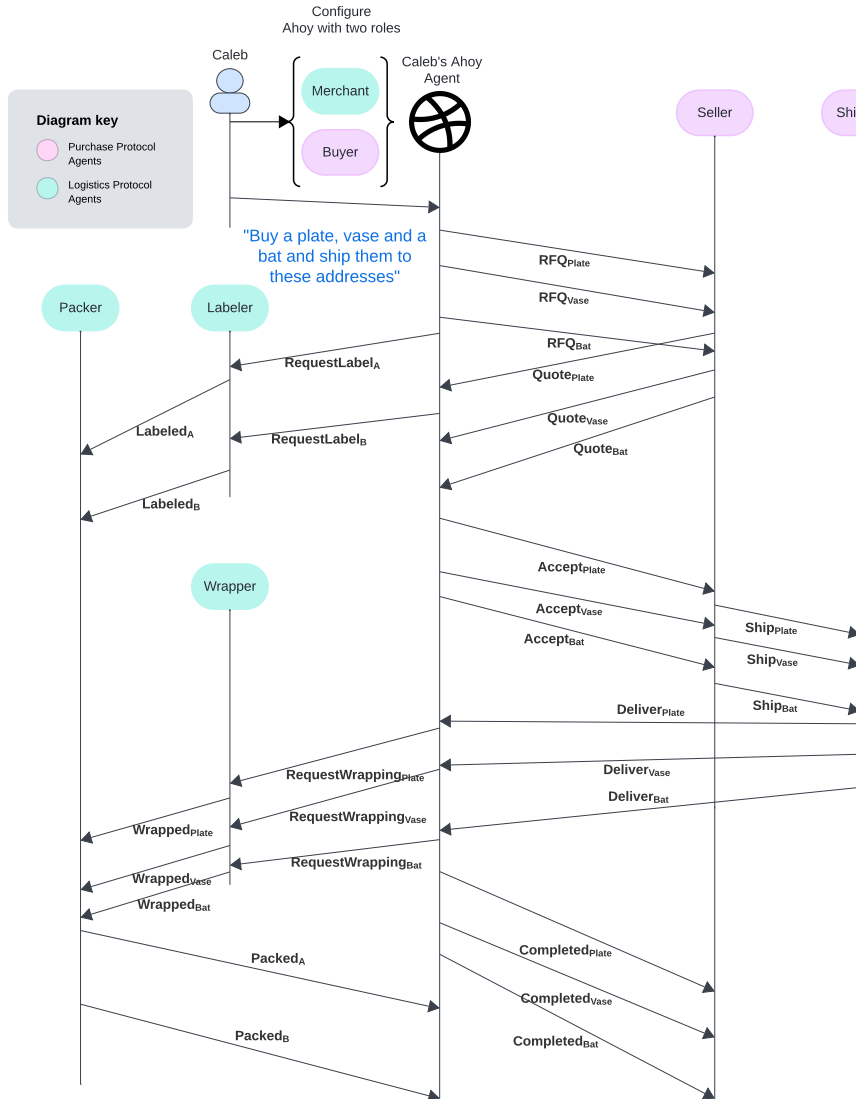
Fig. 7. Concurrent participation in multiple protocols.
