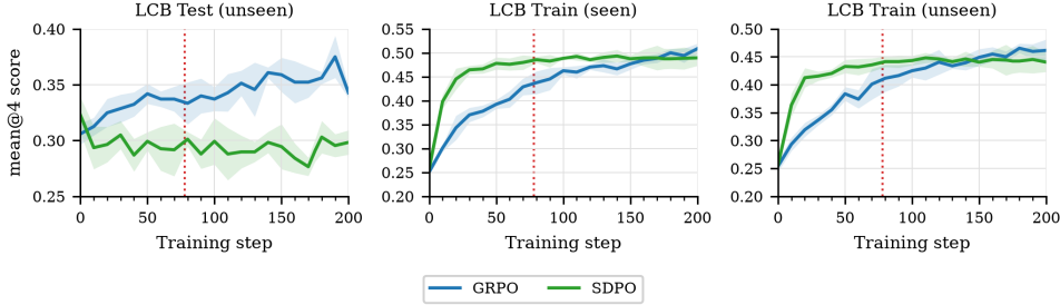
Figure 3: Qwen3-8B SDPO vs. GRPO on LiveCodeBench v6 across four seeds, scored as the fraction of problems with no failing test cases (mean \pm std). TRAIN_SEEN and TRAIN_UNSEEN evaluate training problems on seen and on held-out test cases respectively; TEST_UNSEEN evaluates held-out problems. The 20000 training generations reported by Hübotter et al. (2026) is marked in red.
