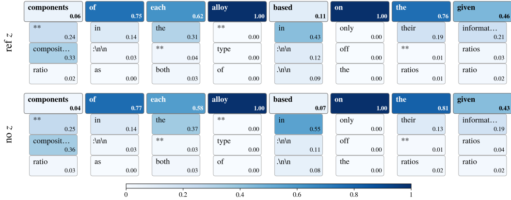
Figure 2: The reference solution barely changes the self-distillation teacher. Teacher log-probabilities (thinking on) along a Qwen3-8B thinking-off student rollout on an OpenThoughts problem, with the problem’s reference solution in context (ref z , top) and with no solution (no z , bottom). In each panel, the first row is the sampled token and the three rows below are the student’s next three most likely tokens. The two teachers assign very similar probabilities, suggesting that OPSD distillation effects do not significantly depend on z (Section 4.3).
