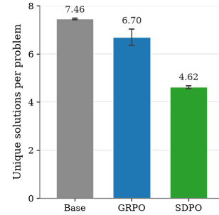
Figure 1: SDPO reduces solution diversity on Live-CodeBench v6. AST-unique solutions per training problem (from 8 samples) for Qwen3-14B before (Base) and after 200 steps of GRPO or SDPO (mean \pm std, four seeds). Diversity collapse suggests memorization.
