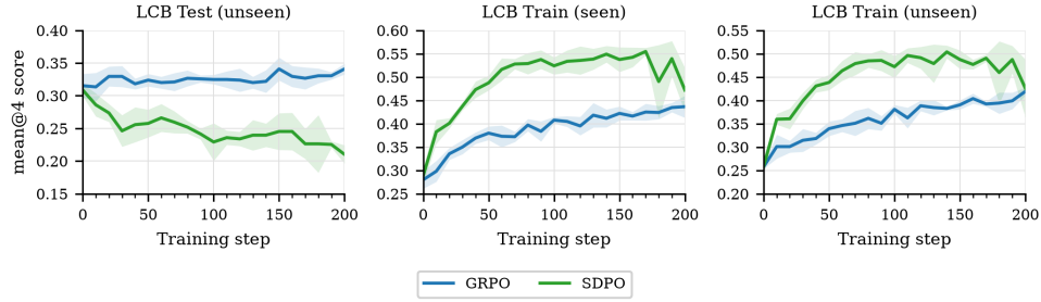
Figure 5: Olmo-3-7B-Instruct SDPO vs. GRPO on LiveCodeBench v6 across four seeds, scored as the fraction of problems with no failing test cases (mean \pm std). TRAIN_SEEN and TRAIN_UNSEEN evaluate problems seen during training, on seen and on held-out test cases respectively; TEST_UNSEEN evaluates held-out problems.
