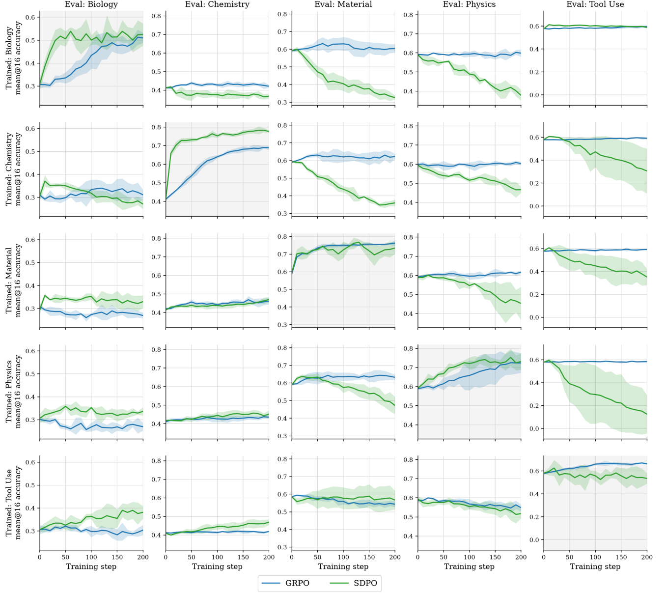
Figure 6: Cross-domain validation accuracy of Qwen3-8B trained with GRPO and SDPO on Sci-KnowEval and ToolAlpaca, averaged over four seeds. Panels vary over training domains (across rows) and evaluation domains (across columns).
