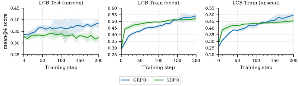
Figure 4: Qwen3-14B SDPO vs. GRPO on LiveCodeBench v6 across four seeds, scored as the fraction of problems with no failing test cases (mean \pm std). TRAIN_SEEN and TRAIN_UNSEEN evaluate problems seen during training, on seen and on held-out test cases respectively; TEST_UNSEEN evaluates held-out problems.
