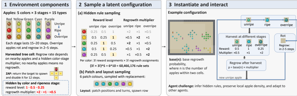
(b) Overview of OpenHarvest. (1) Apples vary across five colors and three ripeness stages. (2) Hidden reward and regrowth rules, patch colors, and the map layout are sampled. (3) In the instantiated environment, harvested cells regrow according to local apple density and a hidden multiplier, whereas rotted apples regrow independently.
