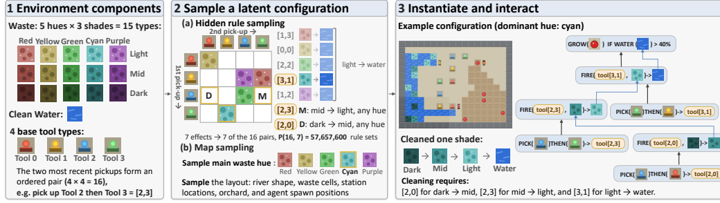
(a) Overview of OpenCleanup. (1) Five waste hues, three shades, and four base tools define the environment components and 16 possible ordered tool pairs. (2) Seven cleaning effects are assigned to different pairs, while a dominant waste hue and map layout are sampled to form a latent configuration. (3) Agents must infer the sampled tool rules and progressively clean waste from dark to mid, light, and water to enable apple growth. The sampled configuration remains fixed across trials within an episode.
