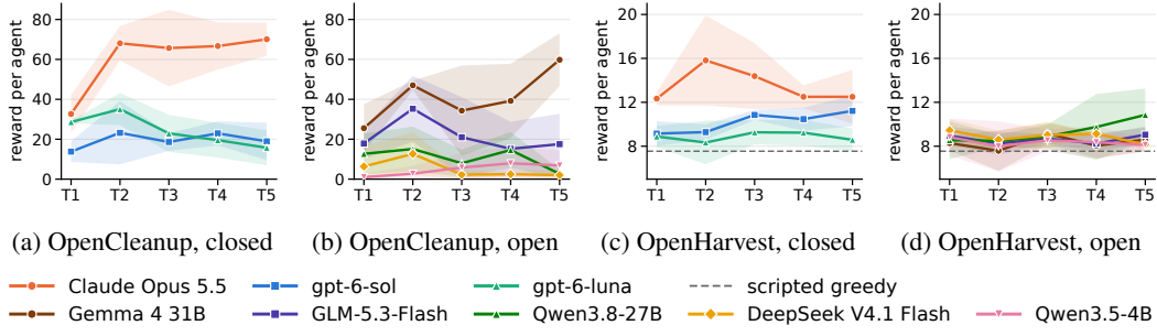
Figure 3: Mean per-agent reward per trial for closed source (closed) and open source (open) models. Shaded bands: \pm 1 s.d. across seeds. Dashed line: scripted greedy policy.
