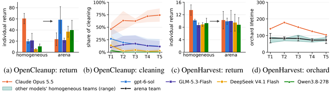
Figure 6: OpenSocialJax arena: each model controls one of the five agents, with seats rotated across seeds. (a, c) Individual return of each model in a homogeneous team and in the arena. (b) Each model’s share of its team’s cleaning in the arena. (d) Orchard lifetime of the arena team, compared with homogeneous teams: Claude Opus 5.5 and, shaded in teal, the range covered by the other four arena models’ homogeneous teams.
