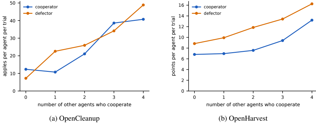
Figure 7: Schelling diagrams, averaged over five trials. Blue: return of a cooperator, C(x) ; orange: return of a defector, D(x) ; x is the number of other agents that are cooperative.
