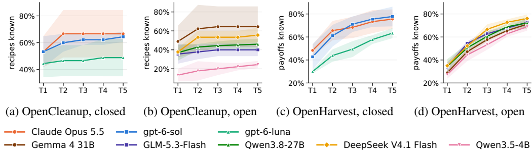
Figure 4: Hidden rules an agent knows by the end of each trial, averaged over agents.
