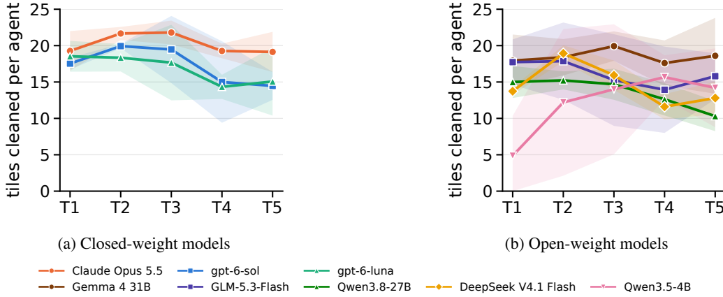
Figure 8: Waste tiles cleared per agent (team total divided by five) in each OpenCleanup trial. Shaded bands: \pm 1 s.d. across 3 seeds.
