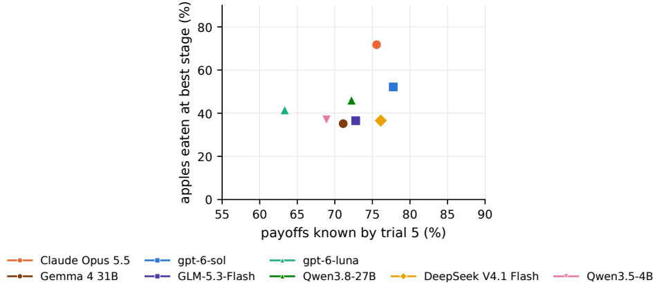
Figure 9: OpenHarvest self-play: share of the payoffs known by the end of trial 5 against the share of apples eaten at their best-paying stage.
