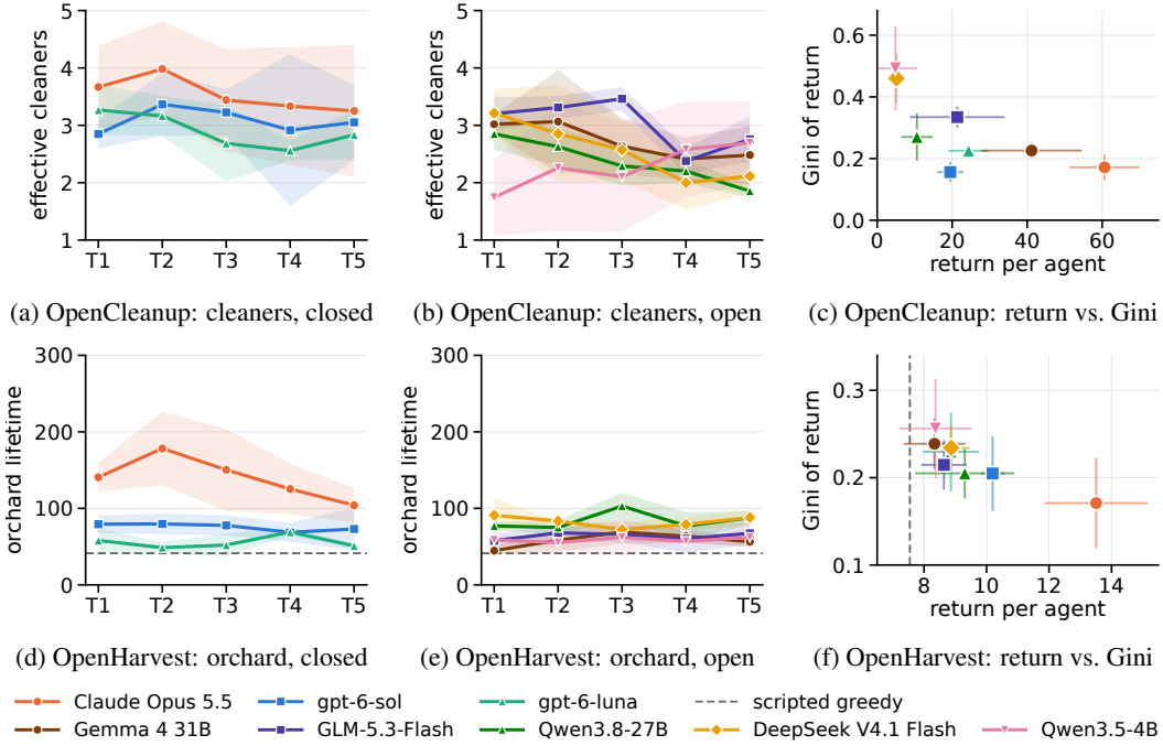
Figure 5: Social dilemma analysis. (a, b) Effective number of cleaners in each OpenCleanup trial, defined as 1/\sum_i s_i^2 , where s_i is agent i ’s share of the team’s total cleaning contribution, measured by the number of waste tiles cleared. A value of 5 indicates that all five agents contribute equally, whereas a value of 1 indicates that a single agent performs all the cleaning. (d, e) Orchard lifetime in each OpenHarvest trial, measured as the timestep at which the final apple is eaten. (c, f) Mean per-agent return against the Gini coefficient of returns within a trial, averaged over trials; bars show \pm 1 s.d. across seeds, and the dashed line in (f) is the scripted greedy policy.
