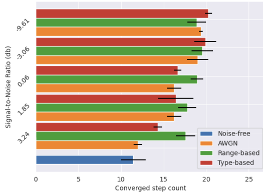
(a) Average steps taken across episodes at convergence under all noise conditions. All methods are trained with HetNet-PPO (S) and 16-bit messages.
