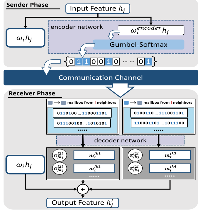
Fig. 4: The sender and receiver phases of the feature update process in a HetGAT layer for one agent, j , of class i .
