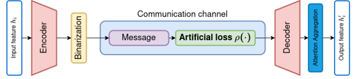
Fig. 5: Visualization of modification to the communication channel for artificial loss
