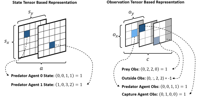
Fig. 3: Proposed tensorized input representations for an agent's state and observation, utilizing multi-dimensional tensors with dimensions (i, c, s_x, s_y) and (i, c, o_x, o_y) . The visualization shows the encoding for a 5 \times 5 PCP environment with a 3 \times 3 observation range.
