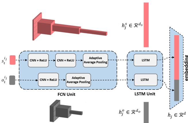
Fig. 2: Visualization of our proposed preprocessing architecture. Separate FCN Units, for state and observation inputs, generate fixed-length embeddings from size-varying tensorized input representations. The hidden embeddings of the following LSTM units are combined, generating a fixed-length embedding for the HetGAT communication channels.
