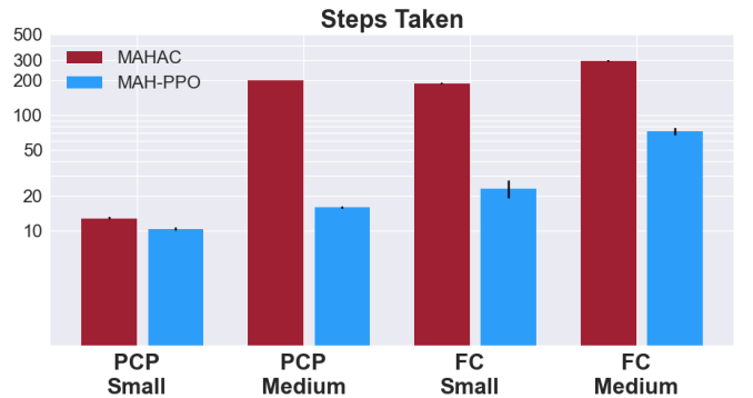
Fig. 8: Performance comparison between HetNet trained with MAHAC in prior work [72] and HetNet trained with MAH-PPO. As shown, HetNet trained with MAH-PPO outperforms HetNet trained with MAHAC across domain configurations.
