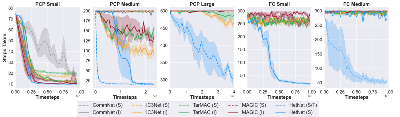
Fig. 6: Learning curves of training in the PCP and FC domains. Shown is average steps taken ( \pm SE) by each method across episodes and three different random seeds as training proceeds. Baseline methods are trained with shared (S) and individual rewards (I). HetNet PPO (S) is trained with shared reward, and HetNet PPO (S/T) is trained with shared reward via transfer. HetNet outperforms all baselines in both domains in performance at convergence and sample efficiency.
