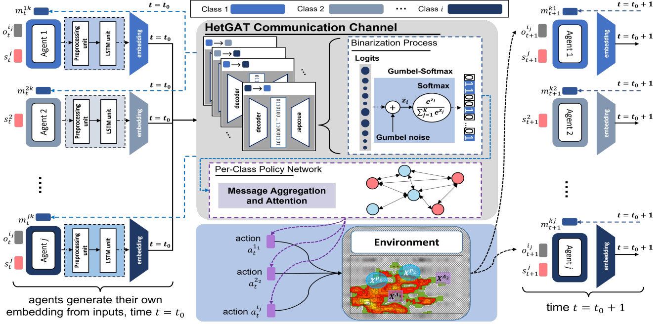
Fig. 1: Overview of our multi-agent heterogeneous attentional communication architecture in a CTDE paradigm. At each time point t = t_0 , each agent j of class i generates a local embedding from its own inputs, by passing its input data through class-specific preprocessing units and an LSTM cell. Each agent then sends the embedding to a class-specific encoder-decoder networks to generate a binarized message, m_t^{jk} , from its local neighbor k . The message information is then decoded and aggregated via learned attention coefficients by the receiving agent to compute the action probabilities as its policy output.
