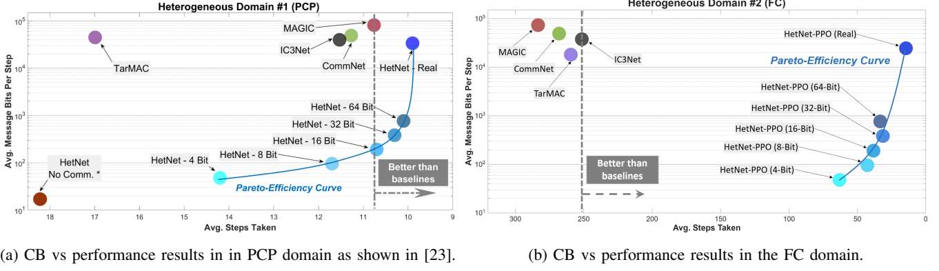
Fig. 9: Results of experiments assessing Communication Bandwidth (CB) as Communicated bits per round of communication. HetNet facilitates binarized messages among agents which requires significantly less CB as compared to real-valued baselines.
