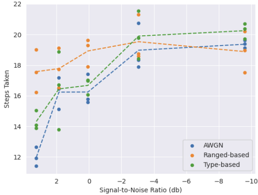
(b) Average steps taken across episodes as SNR decreases in small domain configuration of PCP.
