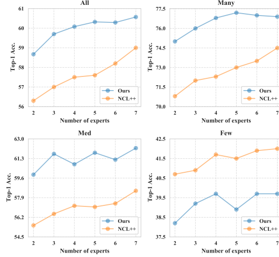
Fig. 4: Comparisons of our method and NCL++ on CIFAR-100-LT (IF=100) with different numbers of experts. While NCL++ achieves superior accuracy in the tail classes, this is accompanied by a high cost in many and medium-shot performance.
