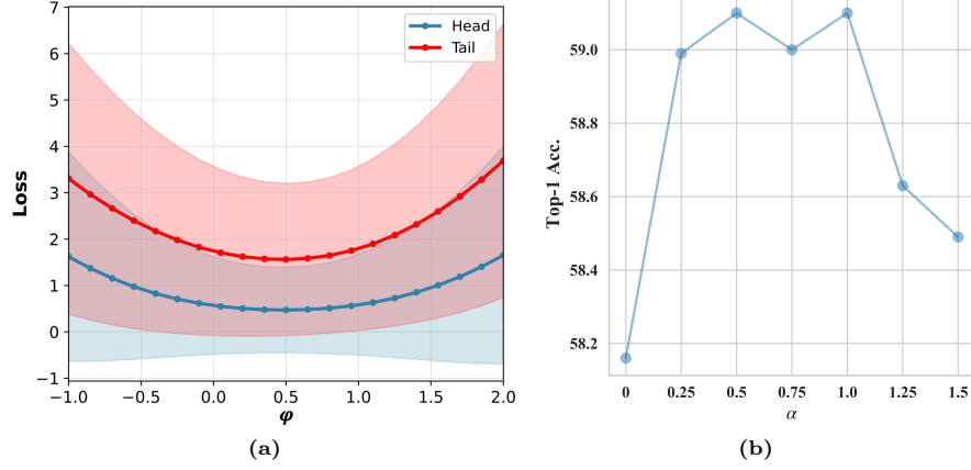
Fig. 3: Ablations of (a) the teacher logit aggregation weight \varphi and (b) the Beta-distribution parameter \alpha on CIFAR-100-LT (IF=100).
