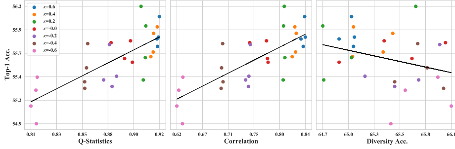
Fig. 1: We use three different diversity metrics, i.e. , Q-statistics, Correlation, and Diversity accuracy, to measure the relationship between model diversity and ensemble accuracy on CIFAR-100-LT with an explicit diversity regularizer . Each point represents an independently trained multi-expert model. \kappa controls the explicit diversity regularizer intensities. A larger \kappa value encourages each expert to align with the ensemble prediction \bar{p} , while a negative \kappa forces predictions to diverge from this ensemble consensus. Ensemble accuracy shows a positive correlation with both Q-statistics and the correlation coefficient \rho . (The Pearson correlation coefficients are 0.76, 0.76, and -0.31 for Q-statistics, Correlation, and Diversity accuracy.)
