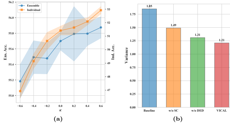
Fig. 2: (a) Ensemble accuracy and mean individual expert accuracy across different \kappa . A large positive \kappa yields better individual accuracy, thereby leading to an improved ensemble performance. (b) Inter-expert logit variance on the CIFAR-100-LT test set. We compute the variance of logits across experts. Lower values indicate stronger cross-expert consistency.
