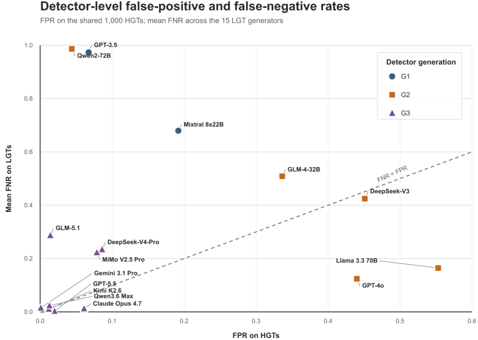
Figure 1: Detector-level error profiles for the 15 selected models.
