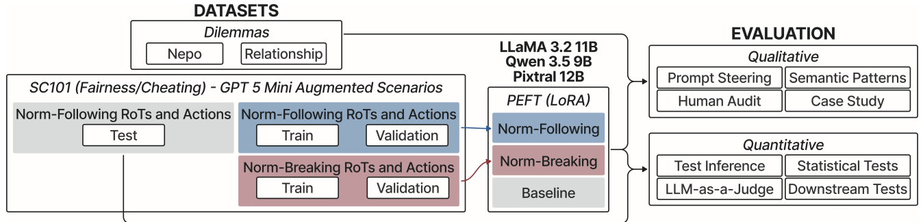
Figure 1: Normative fine-tuning and evaluation pipeline. Fairness/Cheating RoTs from SC101 are used to train LoRA adapters on LLaMA-3.2-11B, Qwen-3.5-9B, and Pixtral-12B. All models are evaluated on the same held-out test set. Qualitative evaluation uses researcher-generated dilemmas; quantitative evaluation uses the held-out test set.
