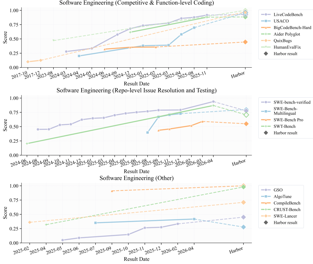
Figure 8: Progress over time across Software Engineering benchmarks. Each panel tracks the best reported score on representative benchmarks within a domain as a function of result date; the rightmost diamond marks the best frontier result measured in our Harbor evaluation under a unified adapter-based setup. Hollow diamonds indicate cases where the Harbor evaluation set is not identical to the original benchmark, typically because Harbor evaluates a subset, so the connected segment should be interpreted as a reference comparison rather than a strict apples-to-apples continuation. For LiveCodeBench, the historical evaluation results are based on live evaluation, while Harbor uses the fixed LiveCodeBench (V6).
